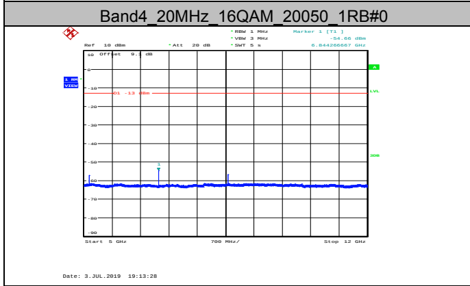
Band4_20MHz_16QAM_20050_1RB#0
