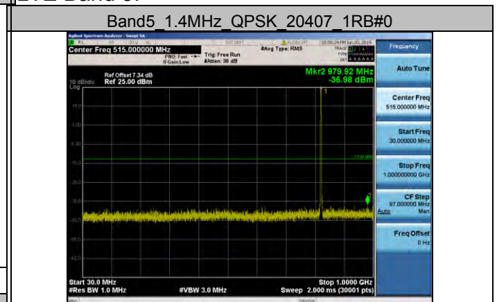
Band5_1.4MHz_QPSK_20407_1RB#0
