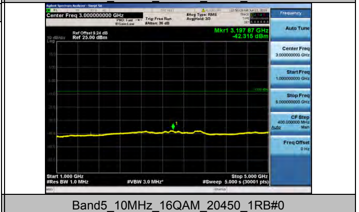
Band5_10MHz_16QAM_20450_1RB#0
