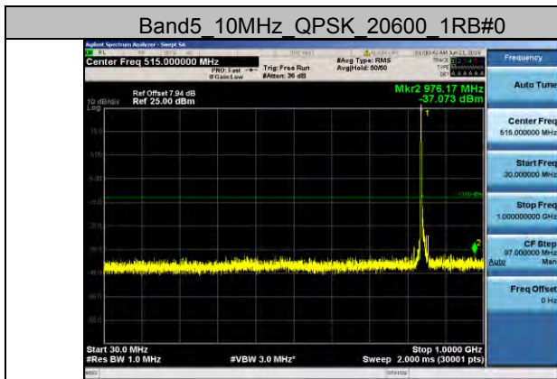
Band5_10MHz_QPSK_20600_1RB#0
