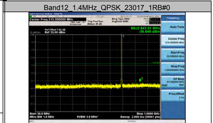
Band12_1.4MHz_QPSK_23017_1RB#0
