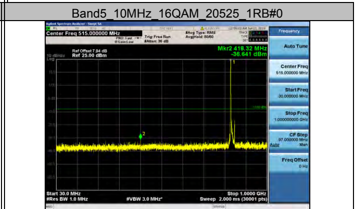
Band5_10MHz_16QAM_20525_1RB#0
