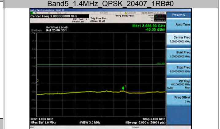
Band5_1.4MHz_QPSK_20407_1RB#0
