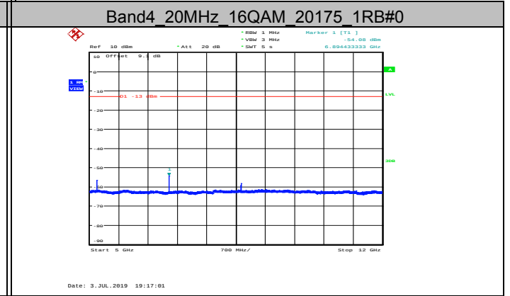
Band4_20MHz_16QAM_20175_1RB#0
