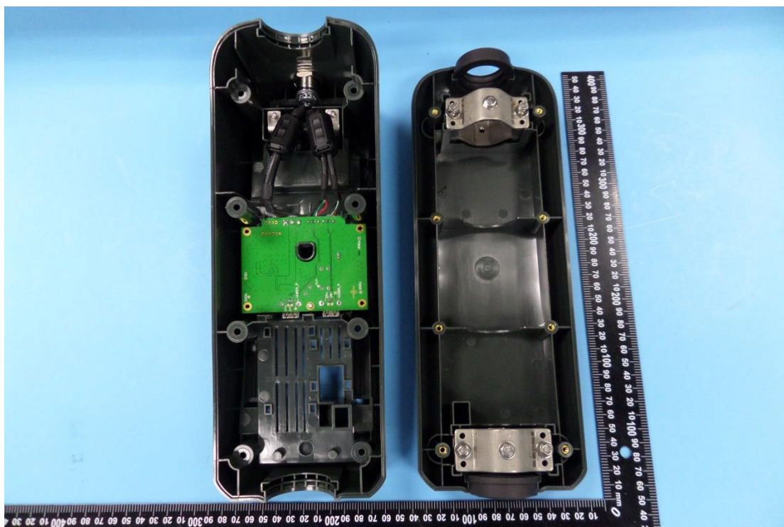
Inside of FX925SF-ING-VPDC-PRE, 011P
