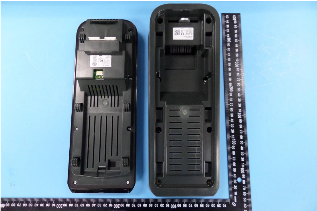
Inside of FX925SF-ING-VWDC-PRE, 011P
