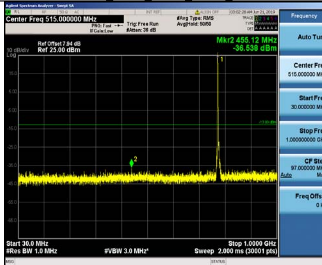
Band13_5MHz_QPSK_23205_1RB#0
