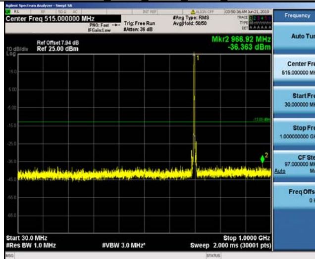
Band17_5MHz_QPSK_23755_1RB#0
