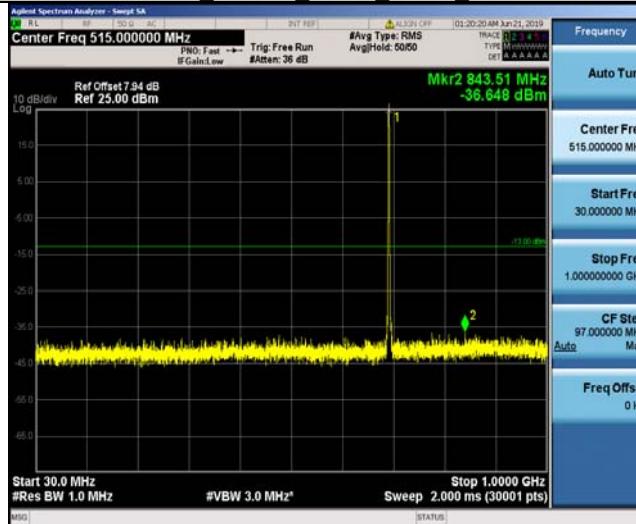
Band12_1.4MHz_QPSK_23017_1RB#0
