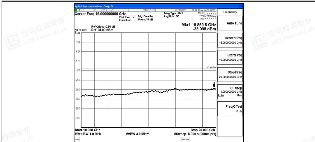
Band2-20MHz-16QAM-19100-1RB#0-Range5:10000~20000MHz
