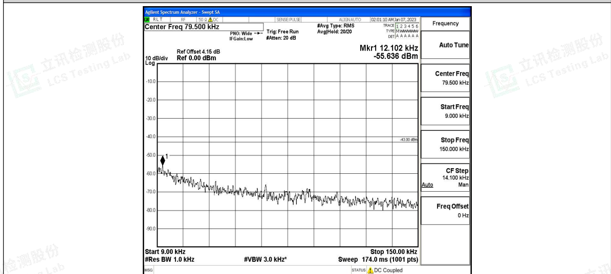
Band2-15MHz-QPSK-18900-1RB#0-Range2:0.15~30MHz
