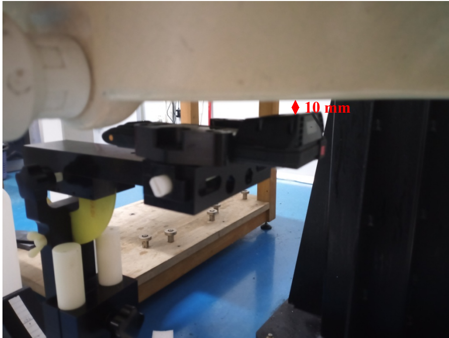
Body Back For WLAN Setup Photo(10mm)
