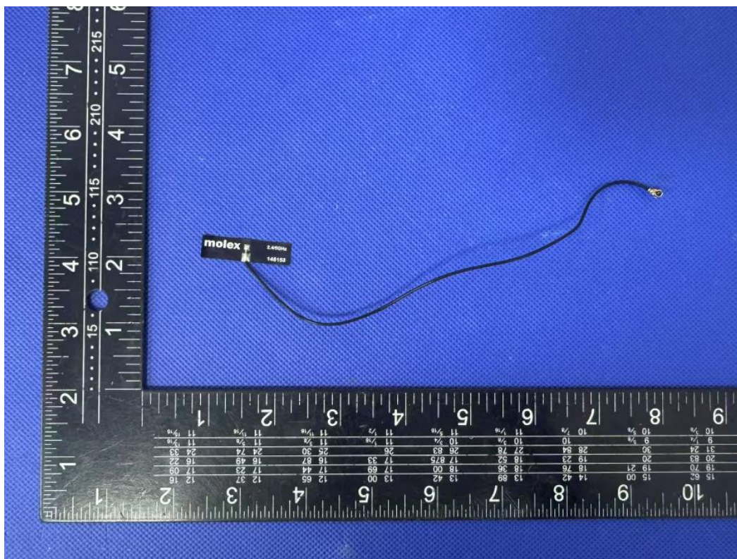
Antenna length:200mm
