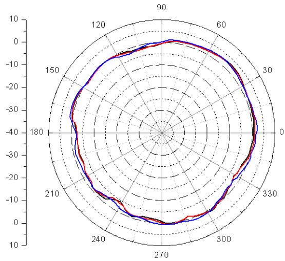
2.4G_Horizontal
