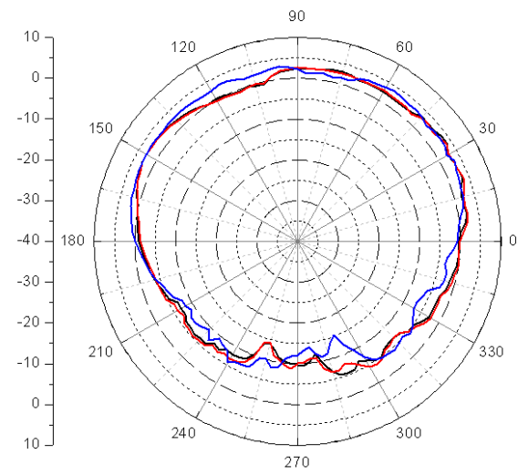
5G_Horizontal
