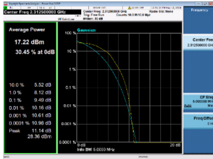
Peak-Average Ratio LTE_40a_LTE_LCH_2312.5MHz_NTNV
