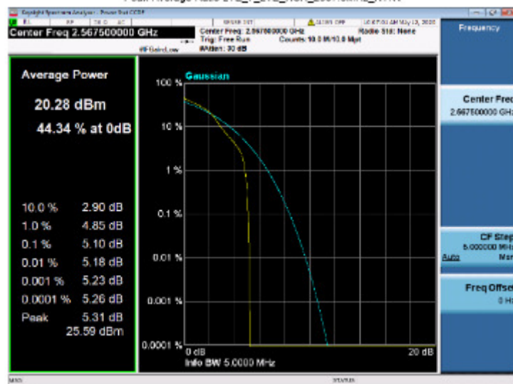
Peak-Average Ratio LTE_7_LTE_MCH_2567.5MHz_NTNV
