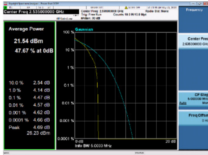
Peak-Average Ratio LTE_7_LTE_MCH_2535.0MHz_NTNV
