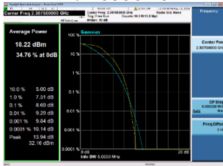
Peak-Average Ratio LTE_40a_LTE_LCH_2307.5MHz_NTNV
