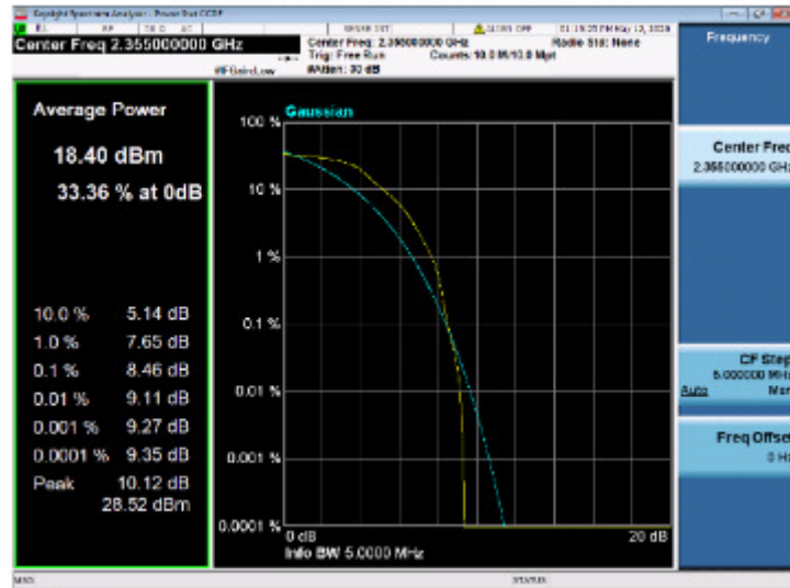
Peak-Average Ratio LTE_40b_LTE_MCH_2355.0MHz_NTNV
