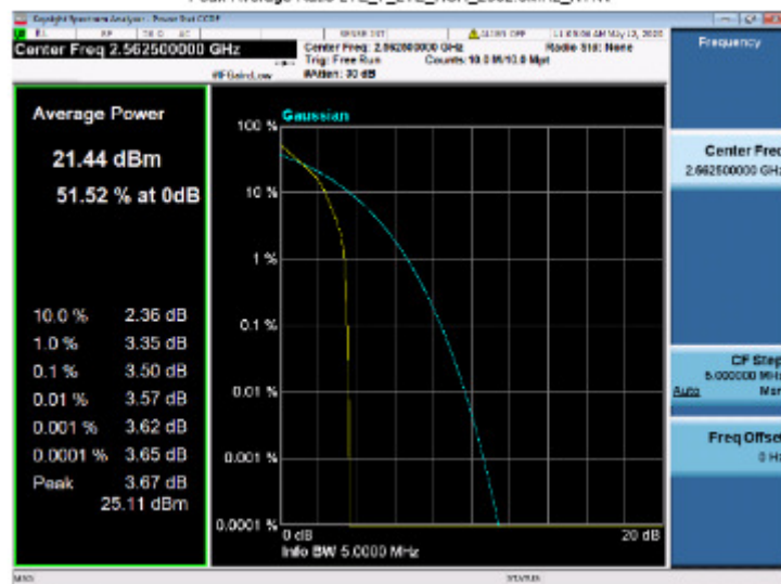
Peak-Average Ratio LTE_7_LTE_MCH_2562.5MHz_NTNV
