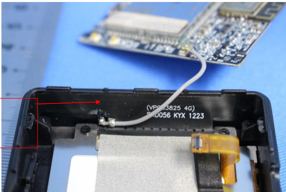
2G3G4G Antenna
