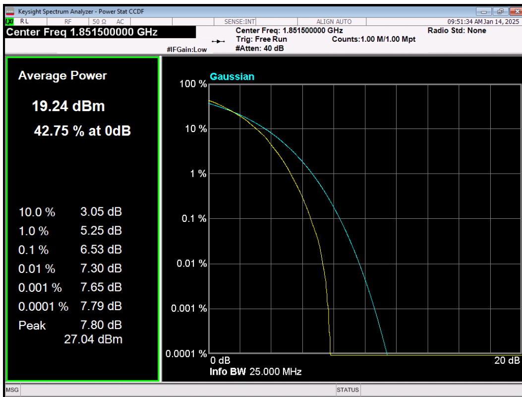
LTE Band2 64QAM BW=3MHz Channel=18615 RB Size=15 Position=#0
