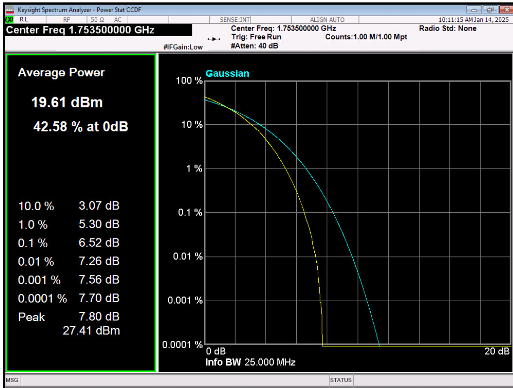
LTE Band4 64QAM BW=3MHz Channel=20385 RB Size=15 Position=#0
