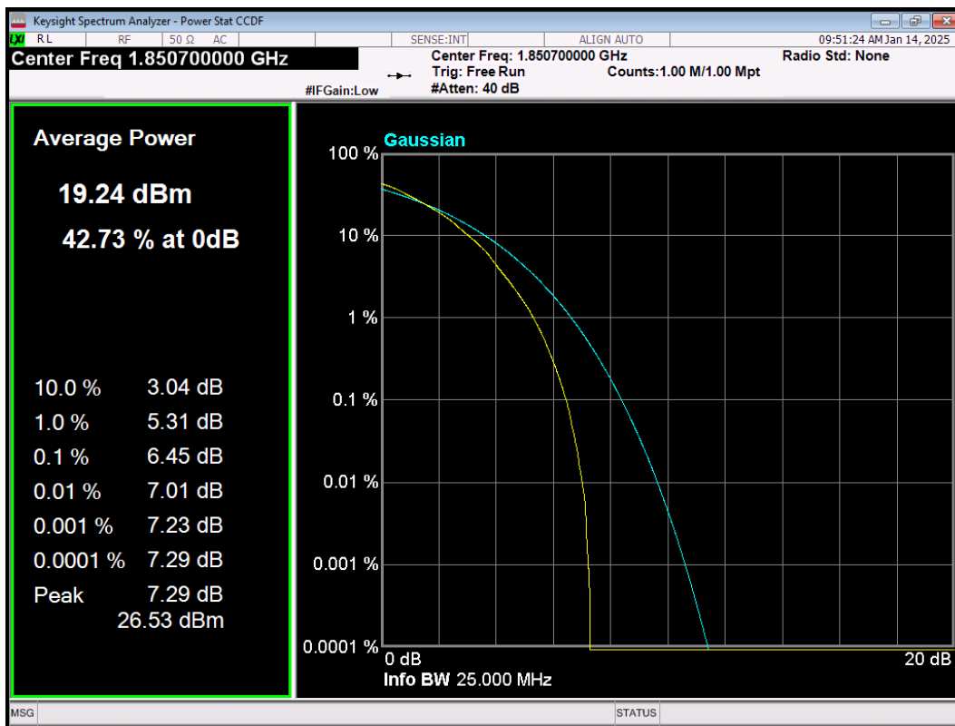
LTE Band2 64QAM BW=1.4MHz Channel=18607 RB Size=6 Position=#0
