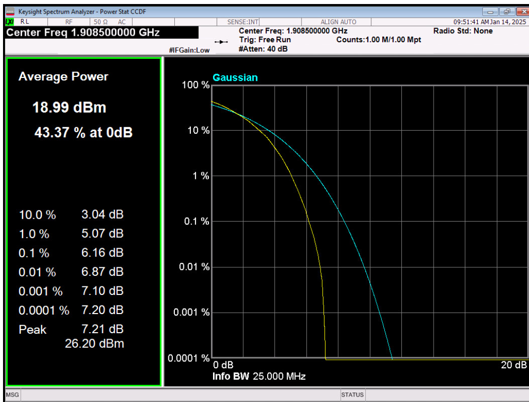
LTE Band2 64QAM BW=3MHz Channel=19185 RB Size=15 Position=#0
