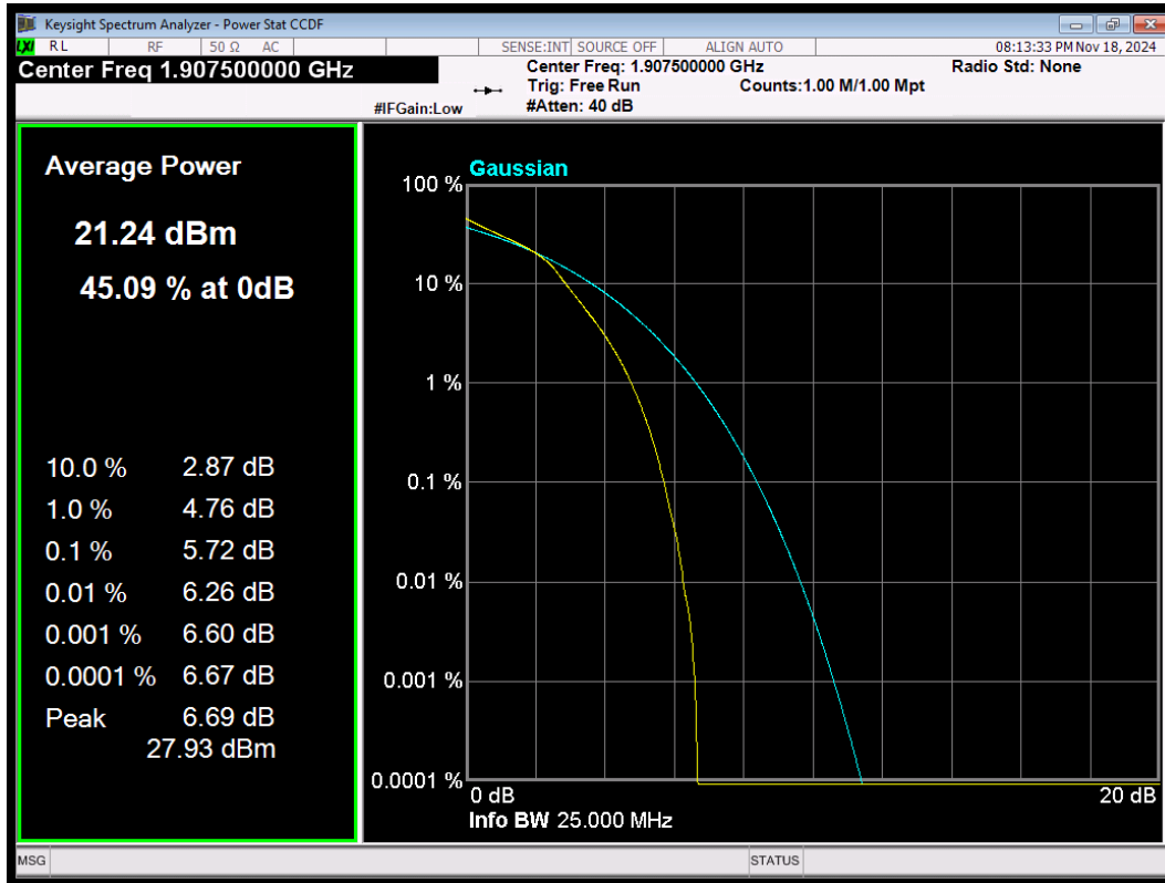
LTE Band2 16QAM BW=5MHz Channel=19175 RB Size=25 Position=#0
