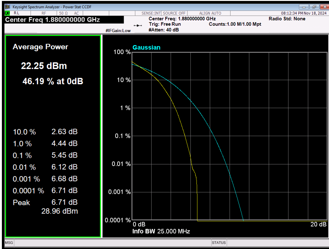
LTE Band2 QPSK BW=1.4MHz Channel=18900 RB Size=6 Position=#0
