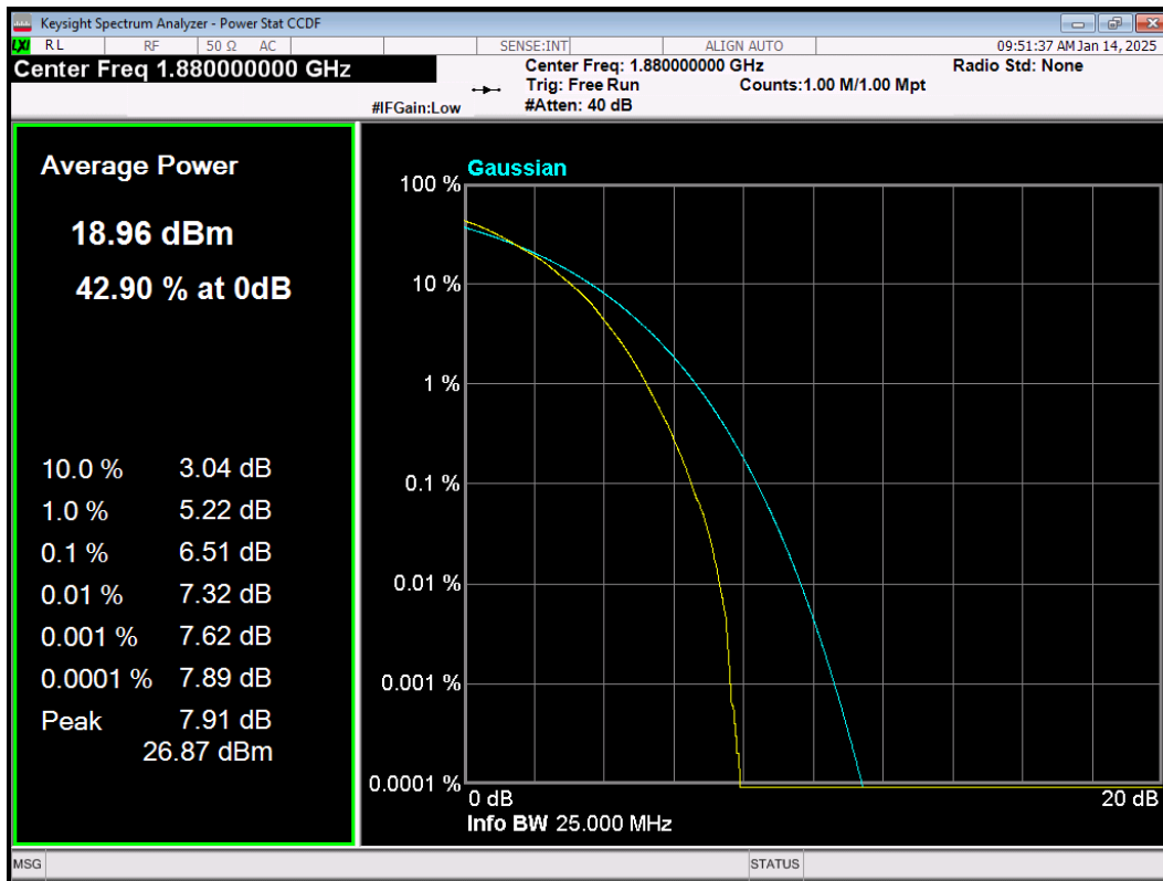
LTE Band2 64QAM BW=3MHz Channel=18900 RB Size=15 Position=#0
