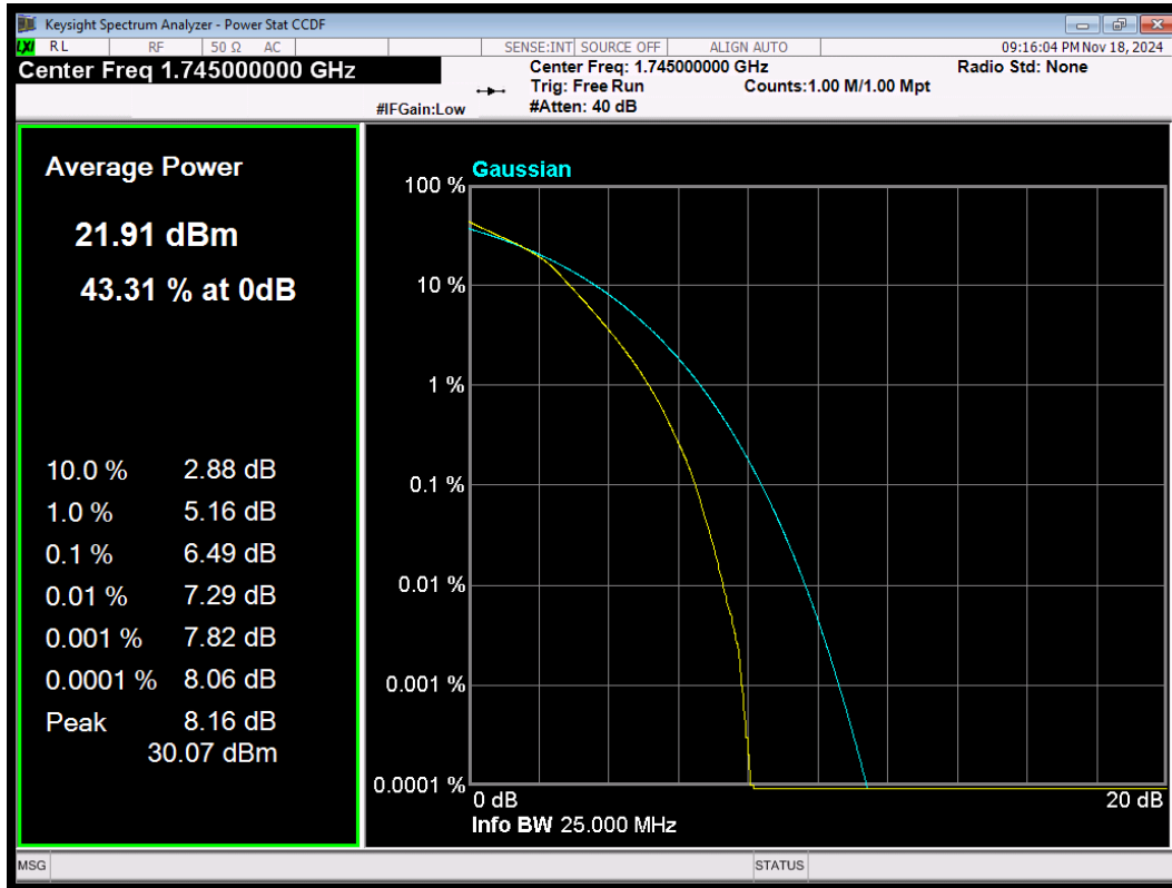
LTE Band4 16QAM BW=20MHz Channel=20300 RB Size=100 Position=#0
