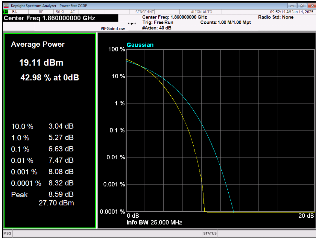
LTE Band2 64QAM BW=20MHz Channel=18700 RB Size=100 Position=#0
