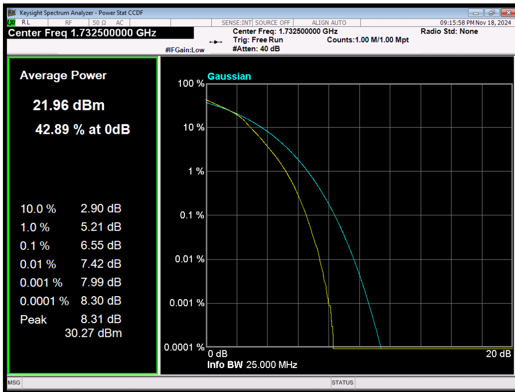
LTE Band4 16QAM BW=20MHz Channel=20175 RB Size=100 Position=#0
