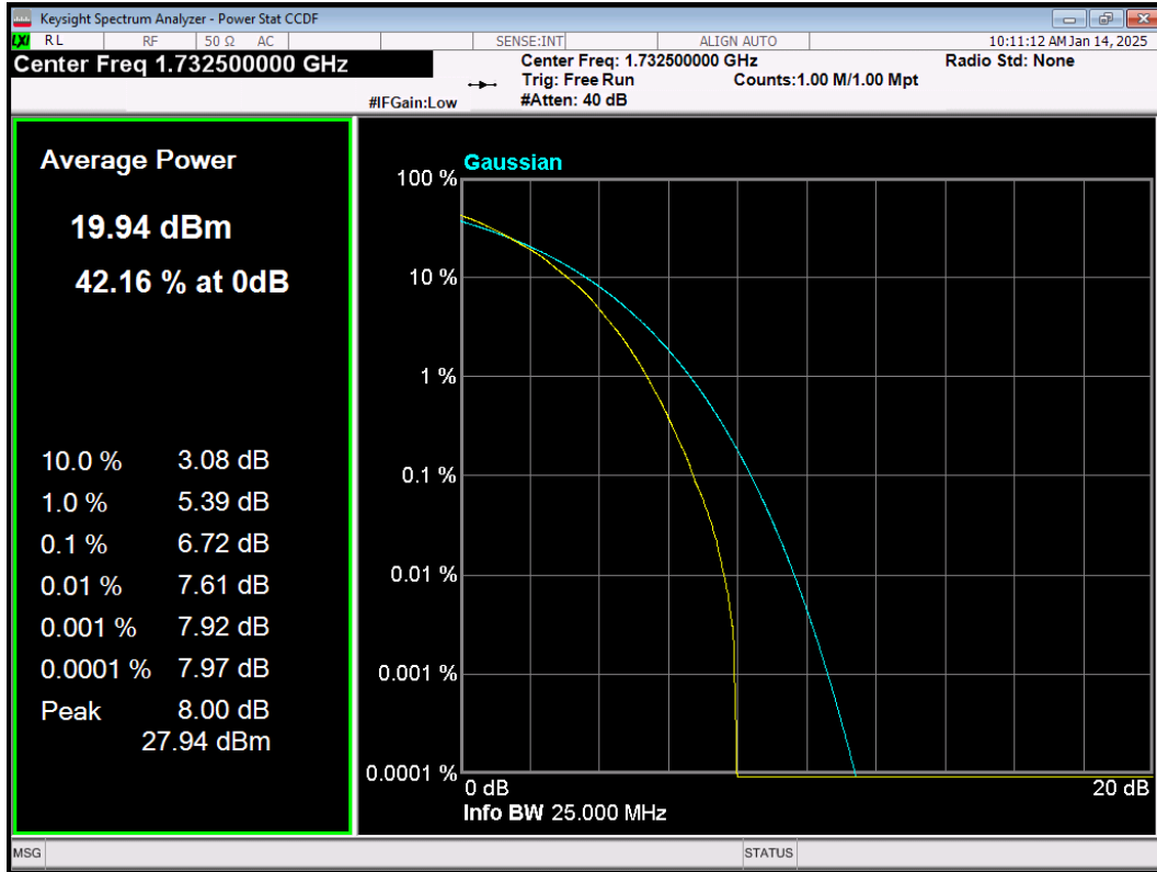
LTE Band4 64QAM BW=3MHz Channel=20175 RB Size=15 Position=#0
