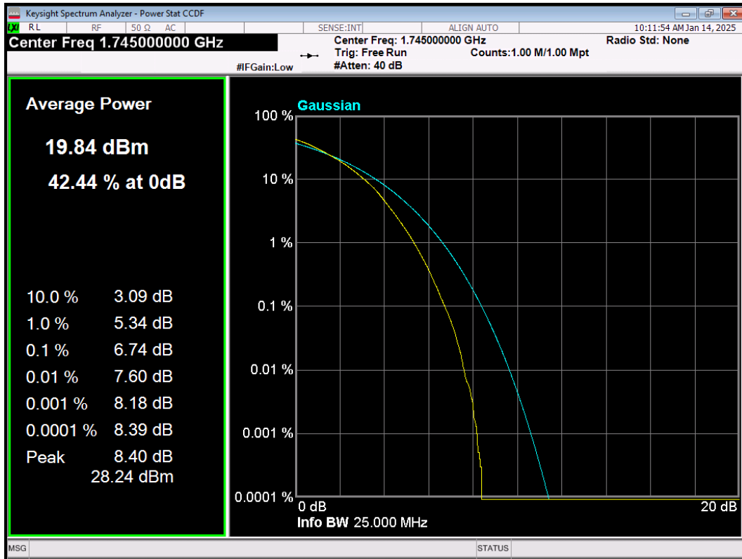
LTE Band4 64QAM BW=20MHz Channel=20300 RB Size=100 Position=#0
