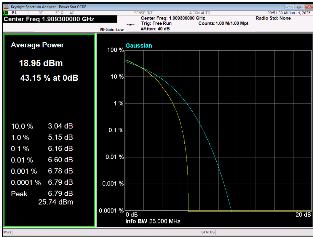
LTE Band2 64QAM BW=1.4MHz Channel=19193 RB Size=6 Position=#0
