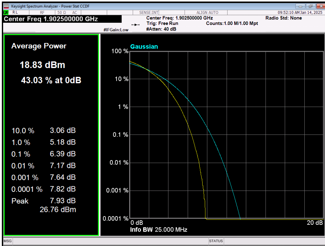
LTE Band2 64QAM BW=15MHz Channel=19125 RB Size=75 Position=#0
