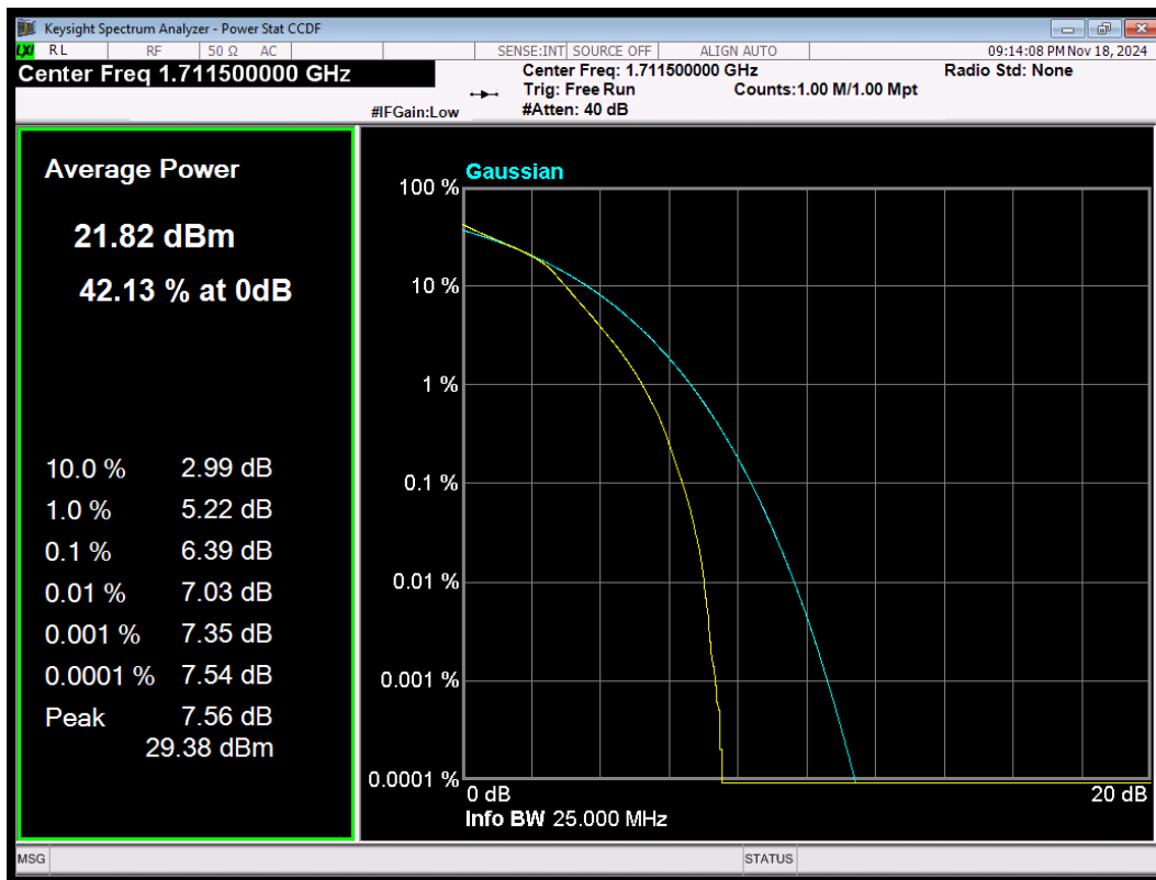
LTE Band4 16QAM BW=3MHz Channel=19965 RB Size=15 Position=#0
