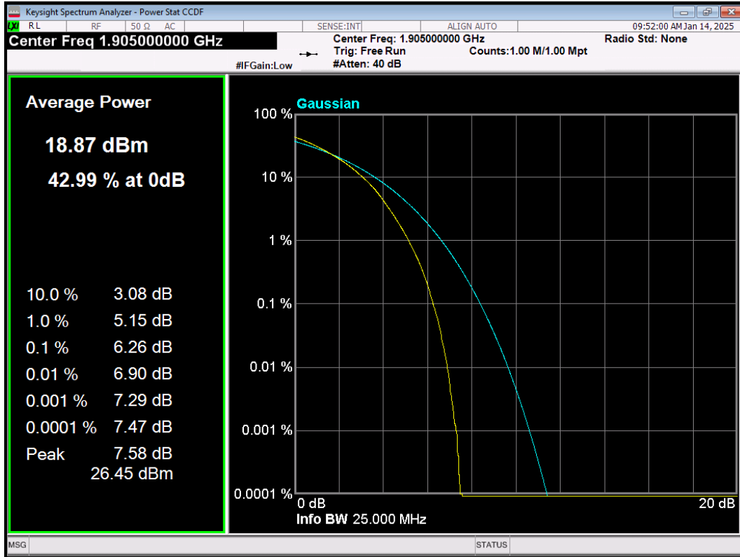
LTE Band2 64QAM BW=10MHz Channel=19150 RB Size=50 Position=#0
