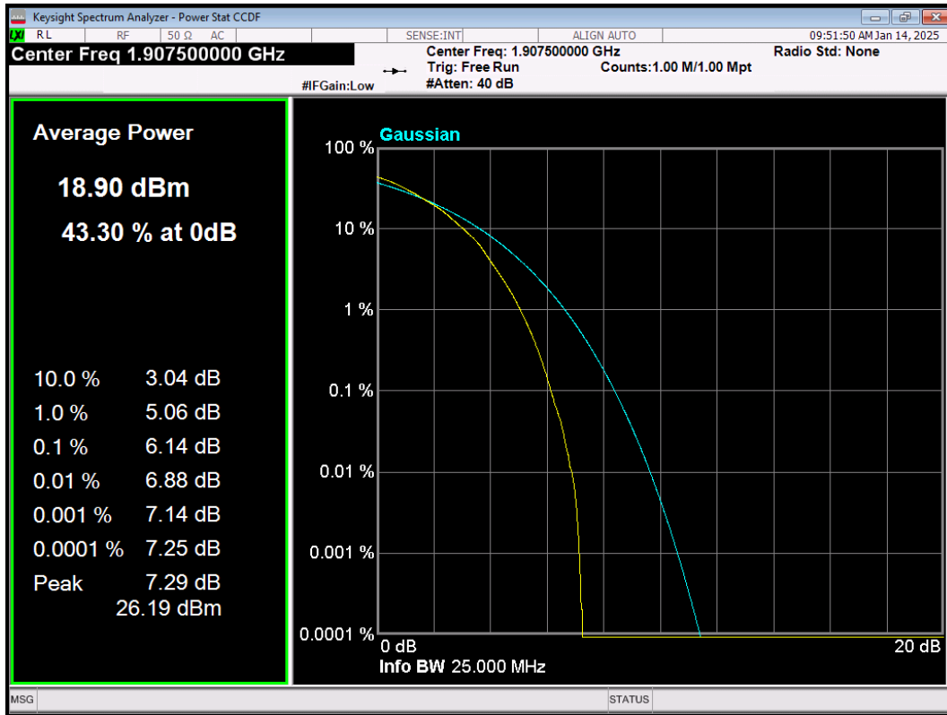
LTE Band2 64QAM BW=5MHz Channel=19175 RB Size=25 Position=#0
