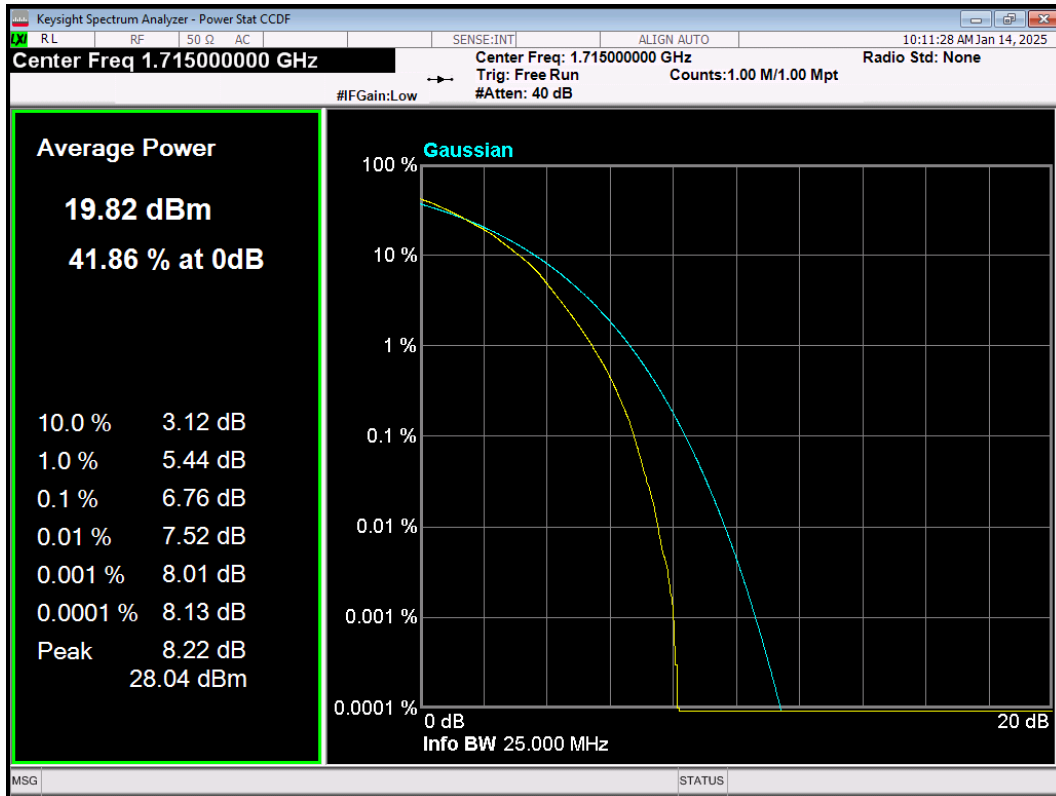
LTE Band4 64QAM BW=10MHz Channel=20000 RB Size=50 Position=#0
