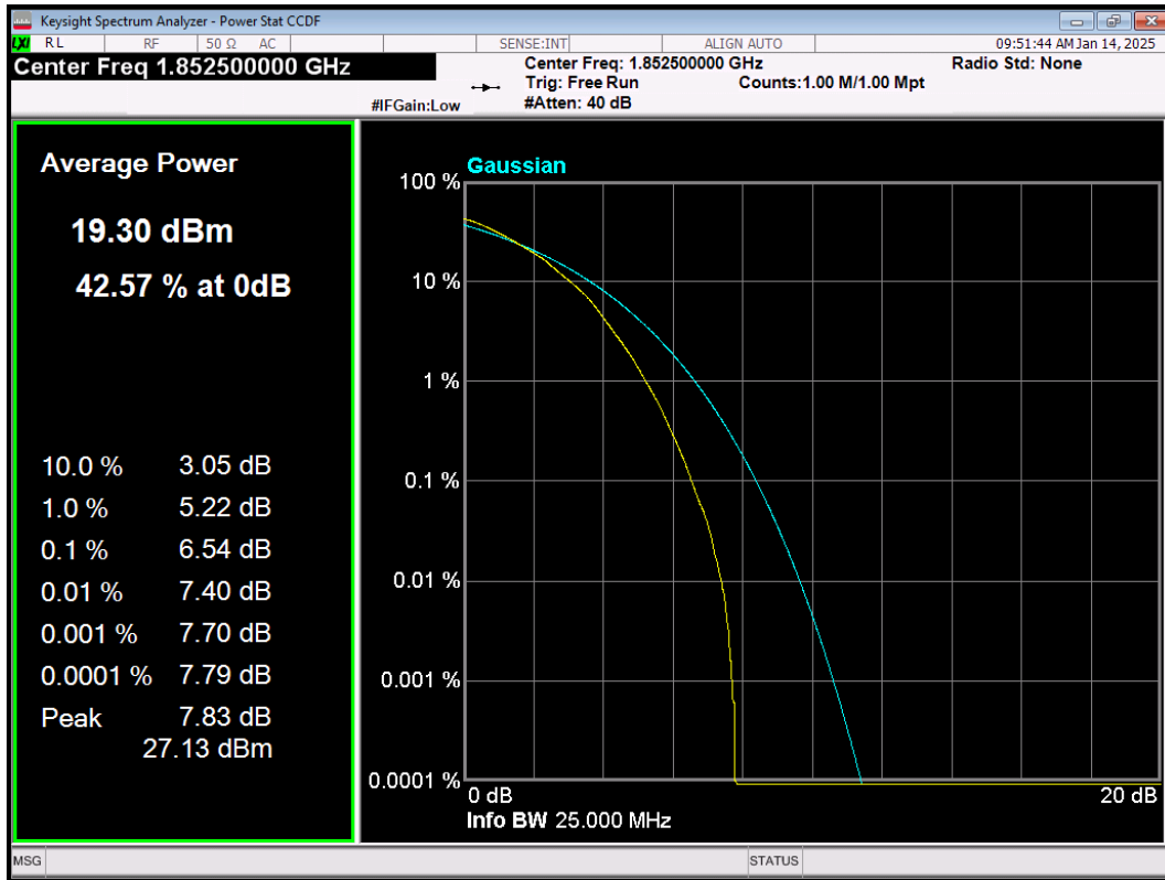
LTE Band2 64QAM BW=5MHz Channel=18625 RB Size=25 Position=#0
