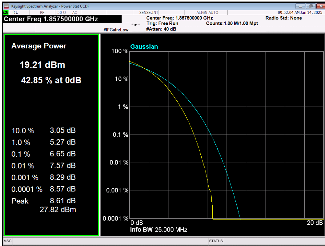
LTE Band2 64QAM BW=15MHz Channel=18675 RB Size=75 Position=#0
