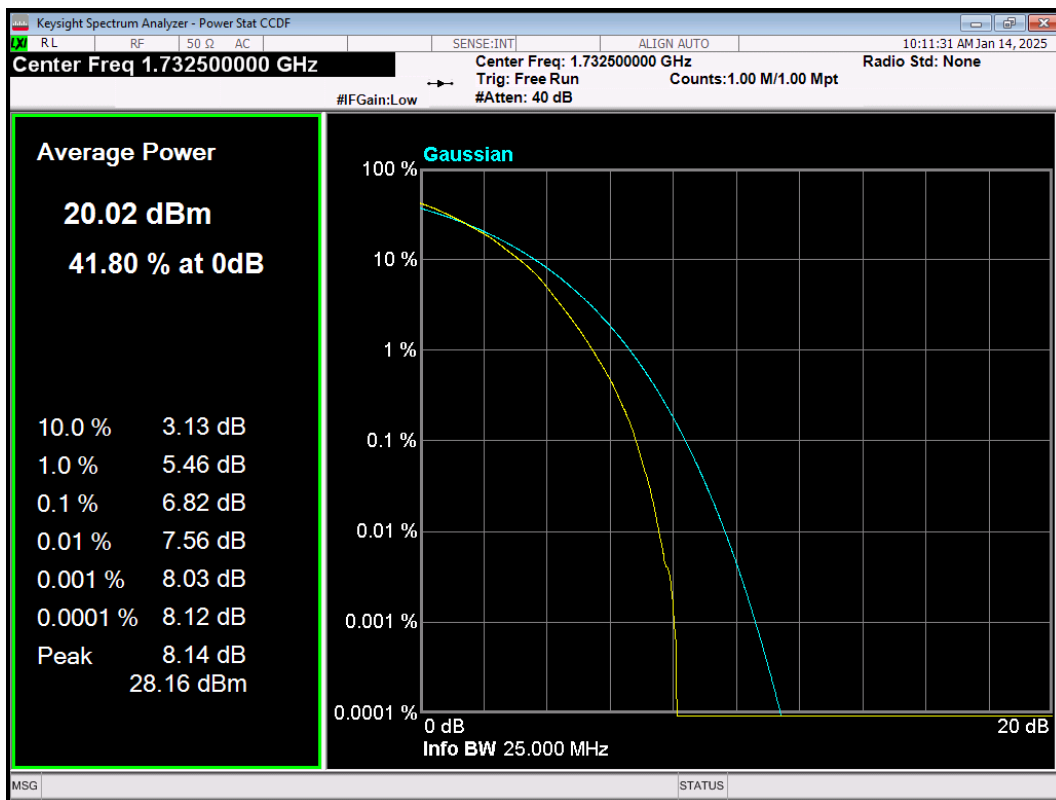
LTE Band4 64QAM BW=10MHz Channel=20175 RB Size=50 Position=#0
