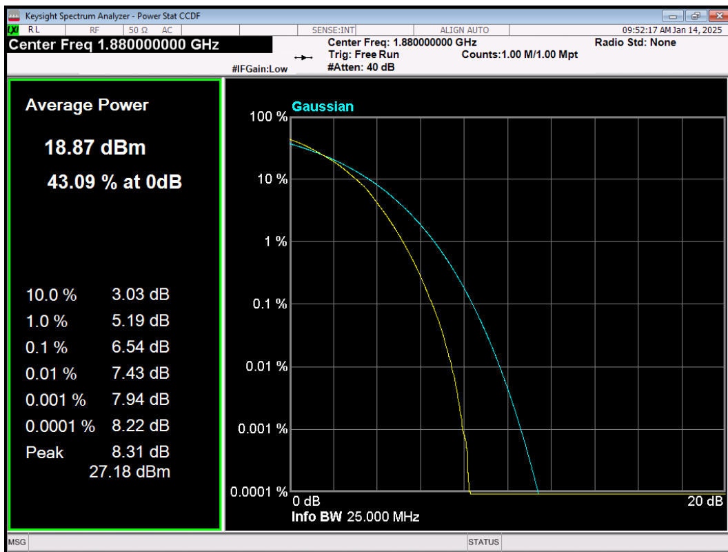
LTE Band2 64QAM BW=20MHz Channel=18900 RB Size=100 Position=#0
