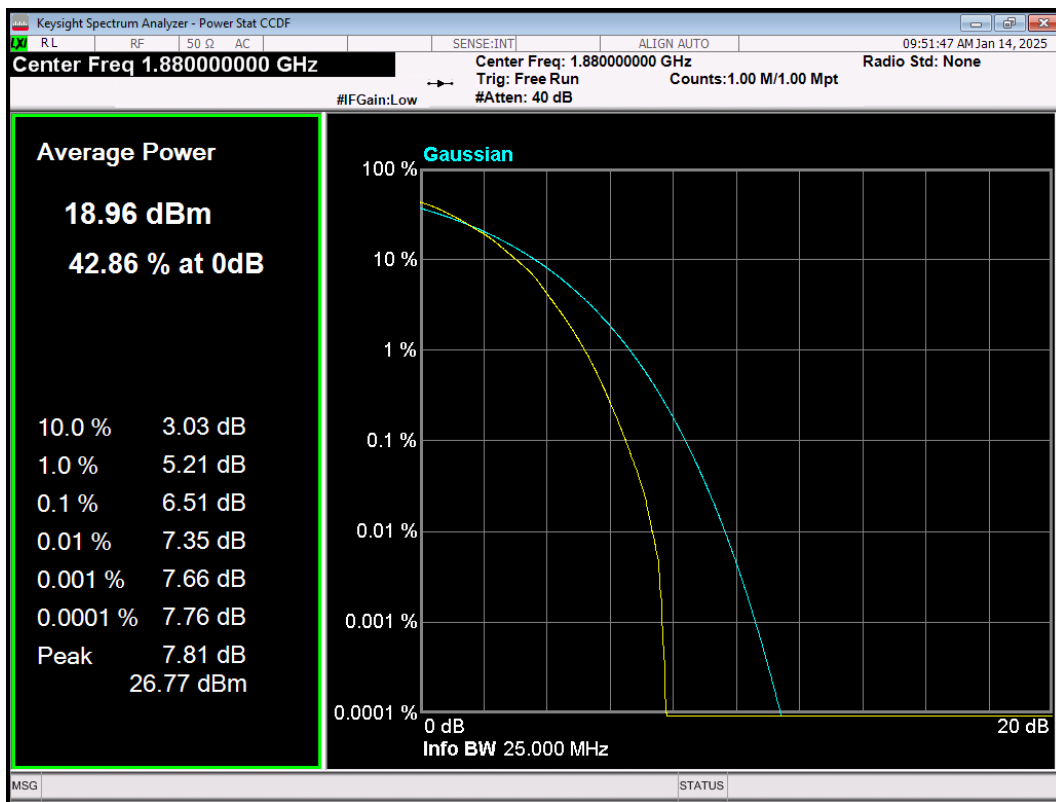
LTE Band2 64QAM BW=5MHz Channel=18900 RB Size=25 Position=#0
