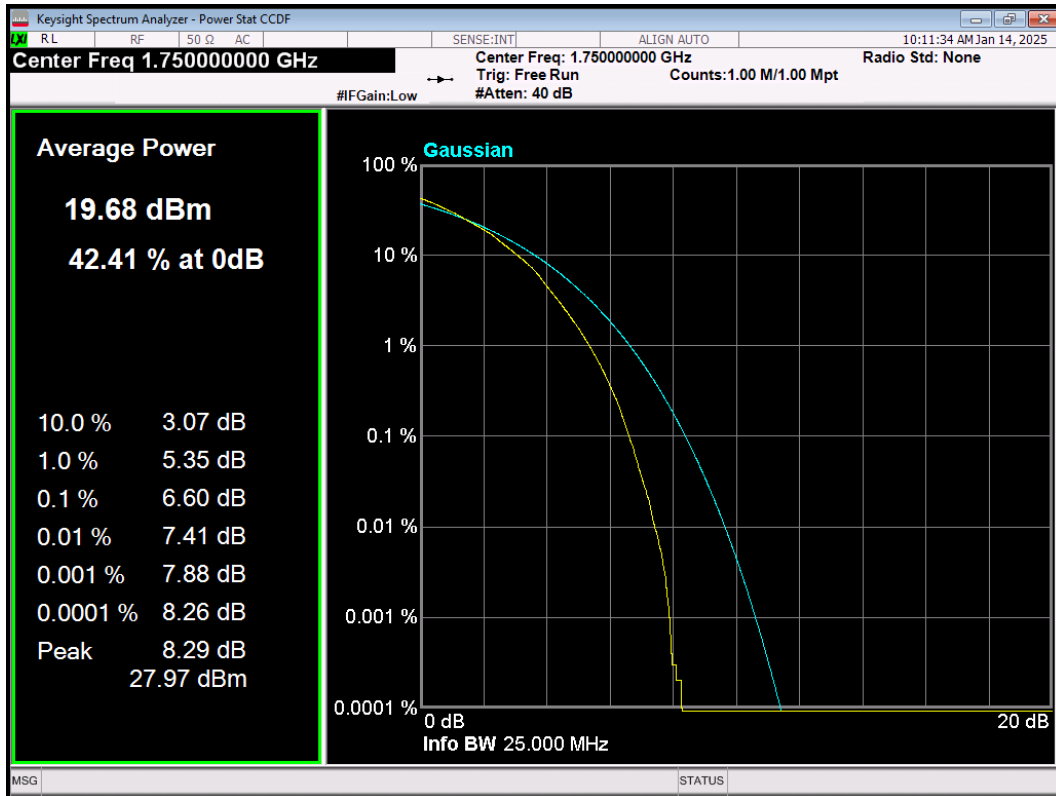
LTE Band4 64QAM BW=10MHz Channel=20350 RB Size=50 Position=#0
