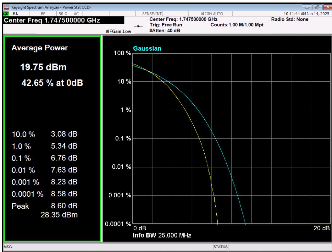
LTE Band4 64QAM BW=15MHz Channel=20325 RB Size=75 Position=#0
