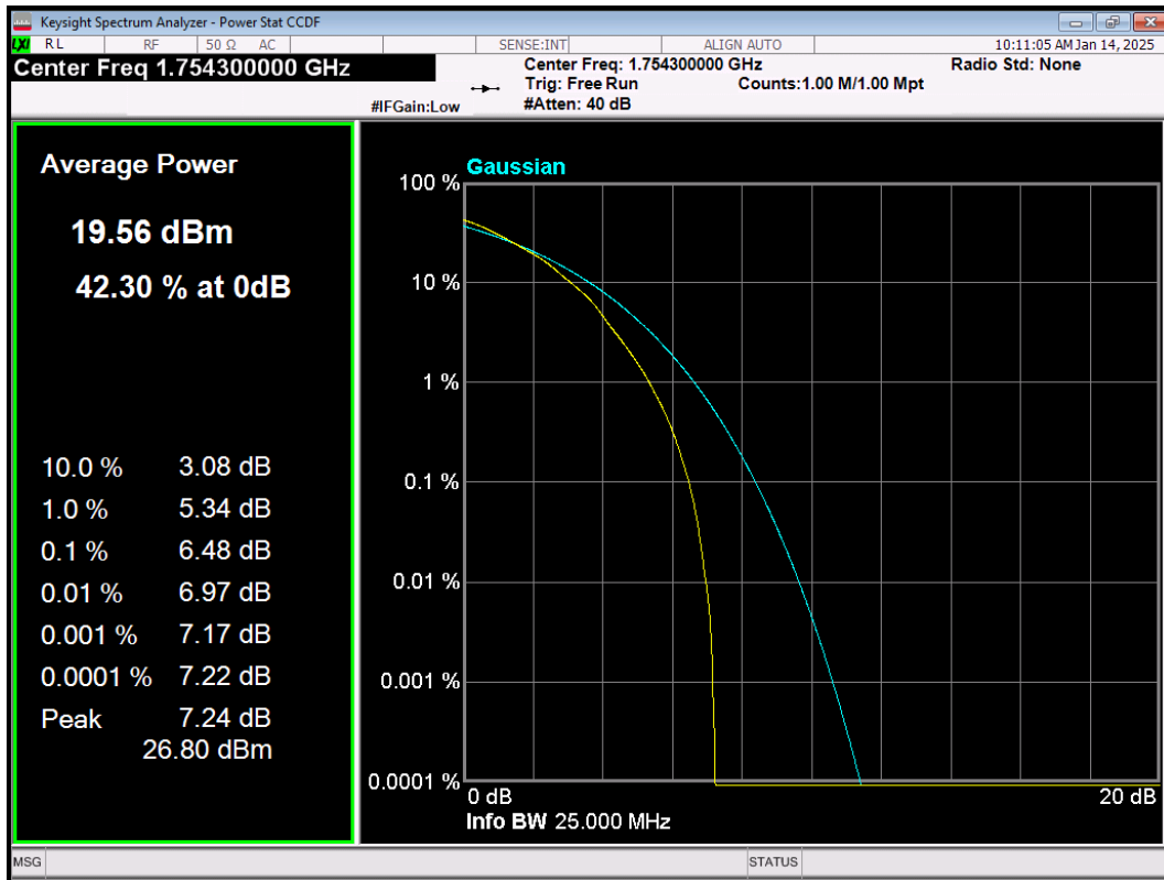
LTE Band4 64QAM BW=1.4MHz Channel=20393 RB Size=6 Position=#0
