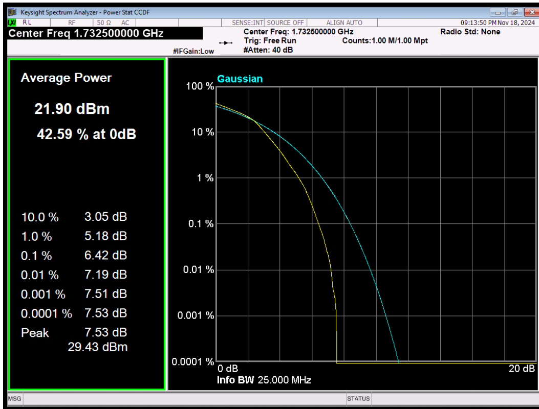
LTE Band4 16QAM BW=1.4MHz Channel=20175 RB Size=6 Position=#0
