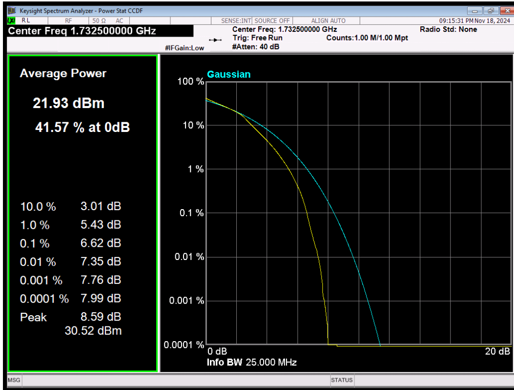
LTE Band4 16QAM BW=15MHz Channel=20175 RB Size=75 Position=#0
