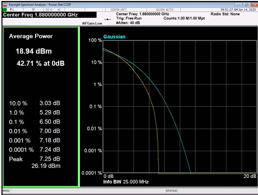
LTE Band2 64QAM BW=1.4MHz Channel=18900 RB Size=6 Position=#0
