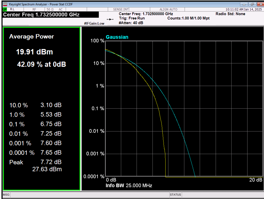
LTE Band4 64QAM BW=1.4MHz Channel=20175 RB Size=6 Position=#0
