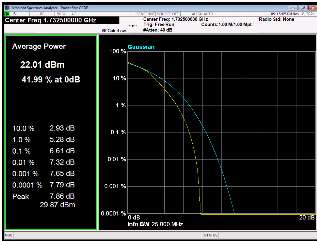
LTE Band4 16QAM BW=10MHz Channel=20175 RB Size=50 Position=#0
