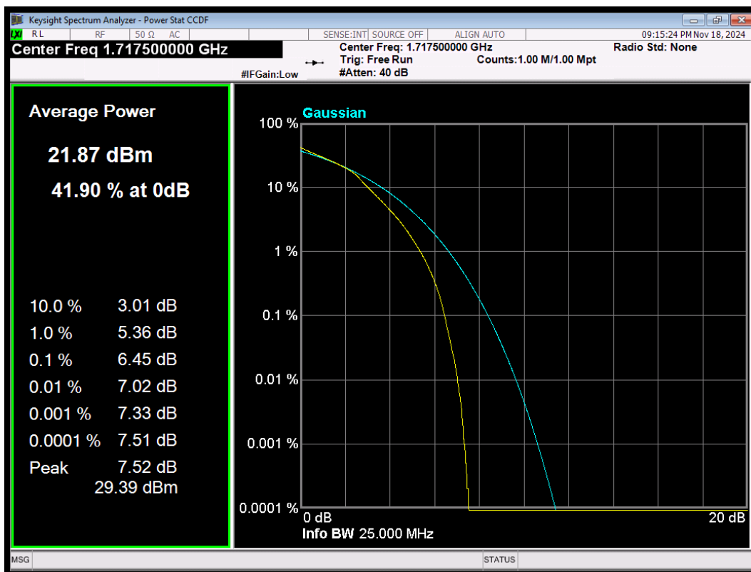
LTE Band4 16QAM BW=15MHz Channel=20025 RB Size=75 Position=#0
