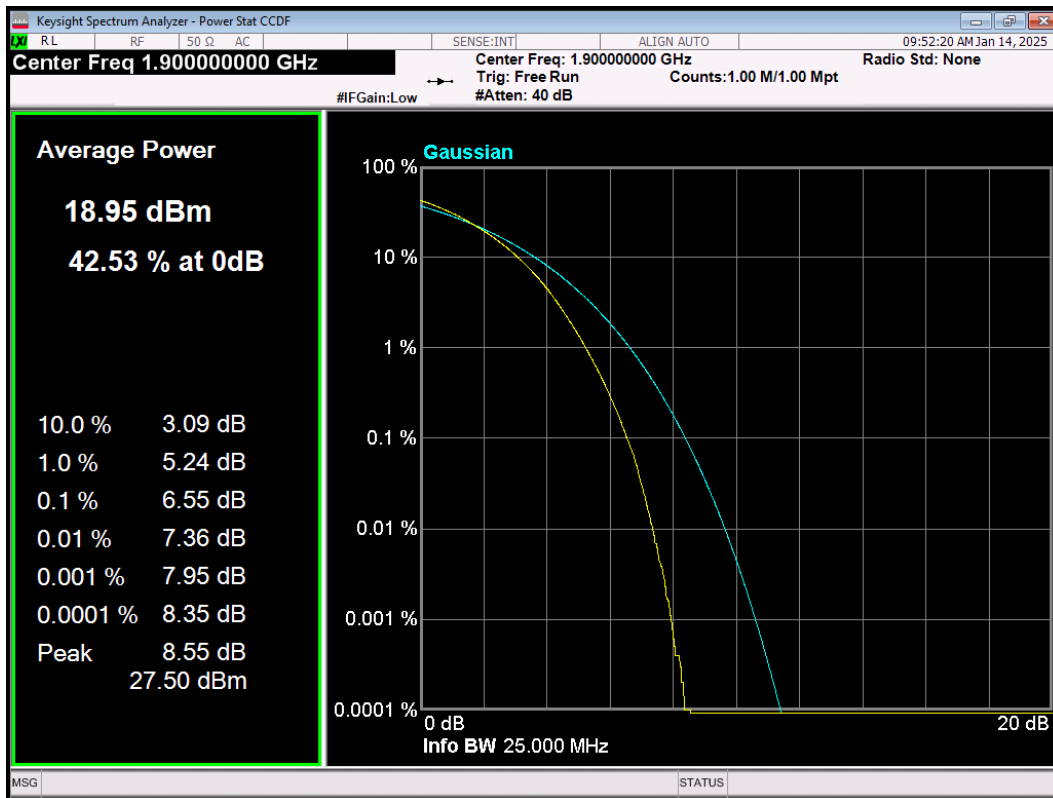
LTE Band2 64QAM BW=20MHz Channel=19100 RB Size=100 Position=#0
