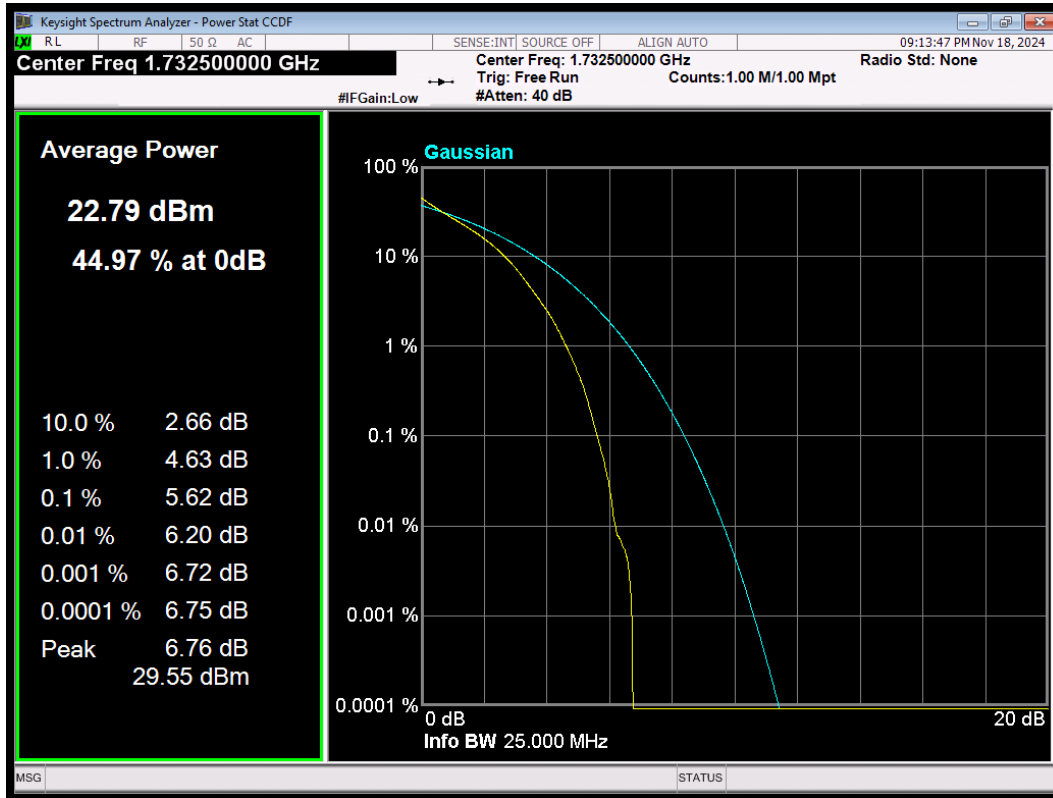
LTE Band4 QPSK BW=1.4MHz Channel=20175 RB Size=6 Position=#0
