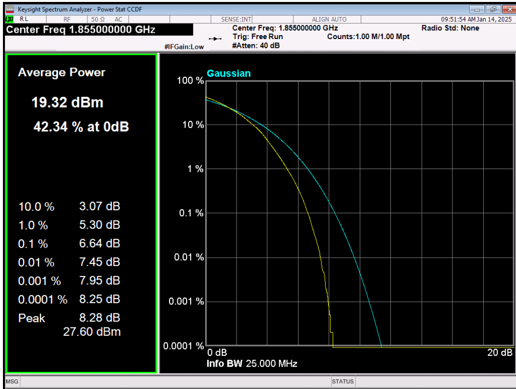
LTE Band2 64QAM BW=10MHz Channel=18650 RB Size=50 Position=#0
