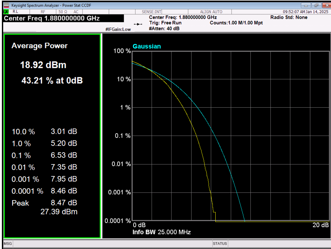
LTE Band2 64QAM BW=15MHz Channel=18900 RB Size=75 Position=#0
