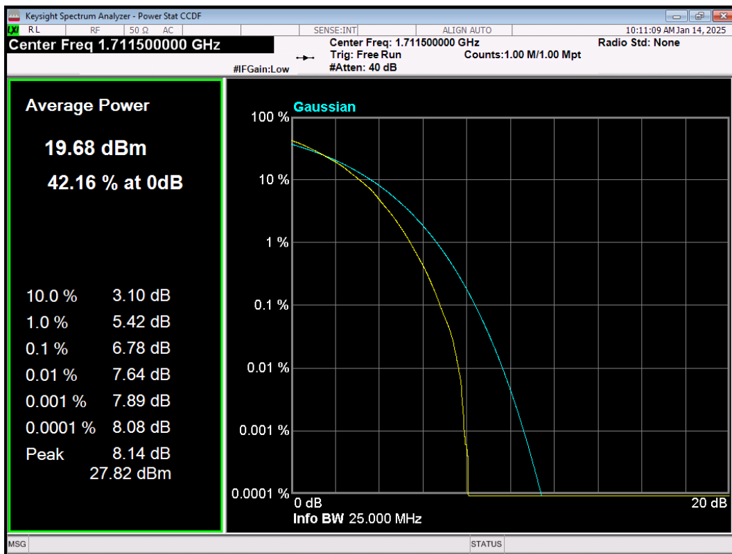
LTE Band4 64QAM BW=3MHz Channel=19965 RB Size=15 Position=#0
