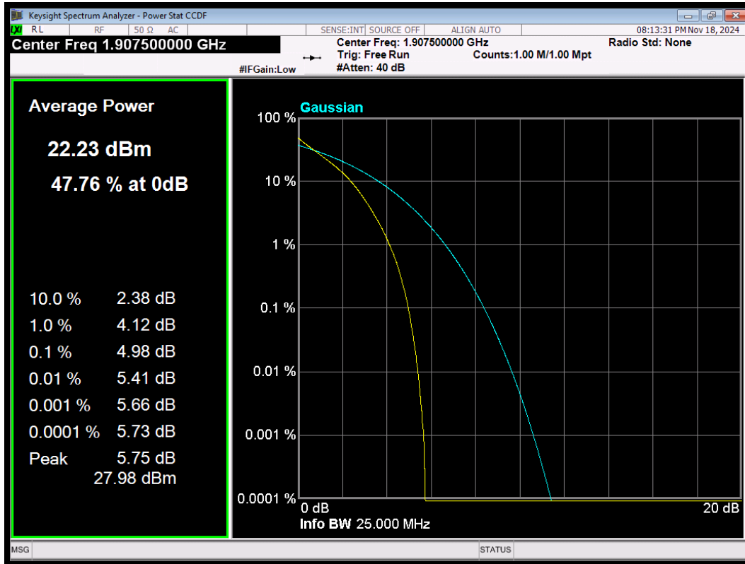
LTE Band2 QPSK BW=5MHz Channel=19175 RB Size=25 Position=#0
