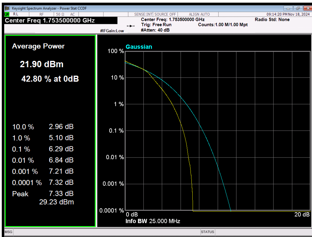
LTE Band4 16QAM BW=3MHz Channel=20385 RB Size=15 Position=#0
