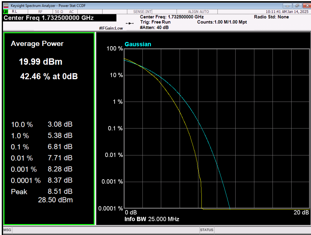
LTE Band4 64QAM BW=15MHz Channel=20175 RB Size=75 Position=#0
