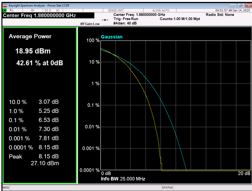
LTE Band2 64QAM BW=10MHz Channel=18900 RB Size=50 Position=#0
