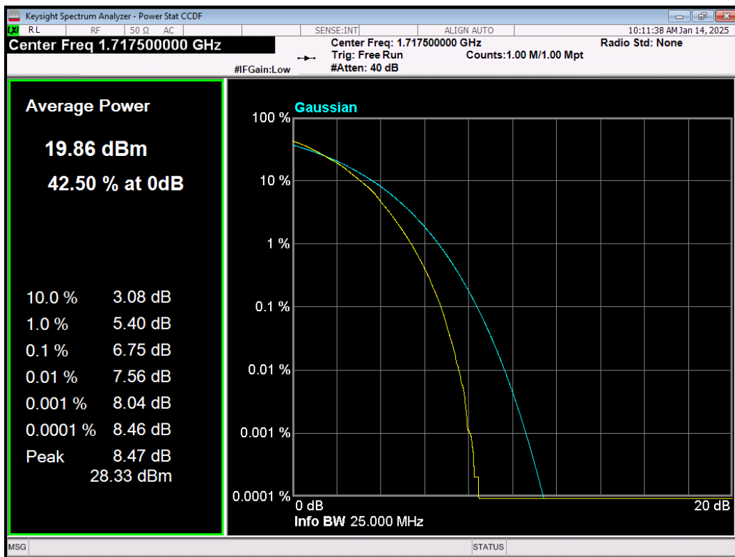
LTE Band4 64QAM BW=15MHz Channel=20025 RB Size=75 Position=#0
