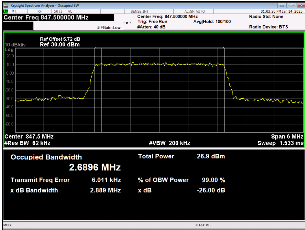
LTE Band26(824-849) 64QAM BW=3MHz Channel=27025 RB Size=15 Position=#0
