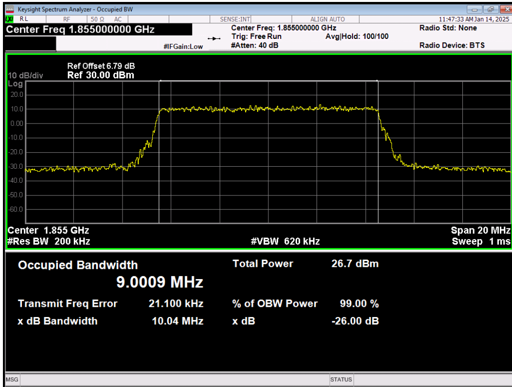
LTE Band25 64QAM BW=10MHz Channel=26090 RB Size=50 Position=#0
