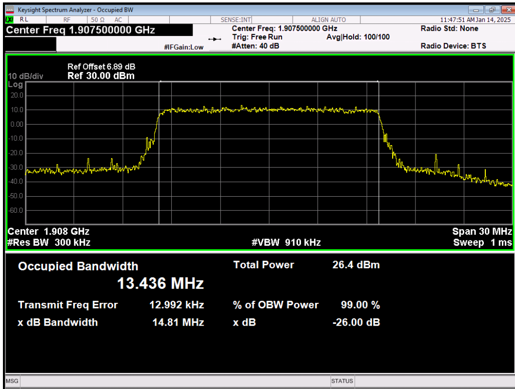
LTE Band25 64QAM BW=15MHz Channel=26615 RB Size=75 Position=#0
