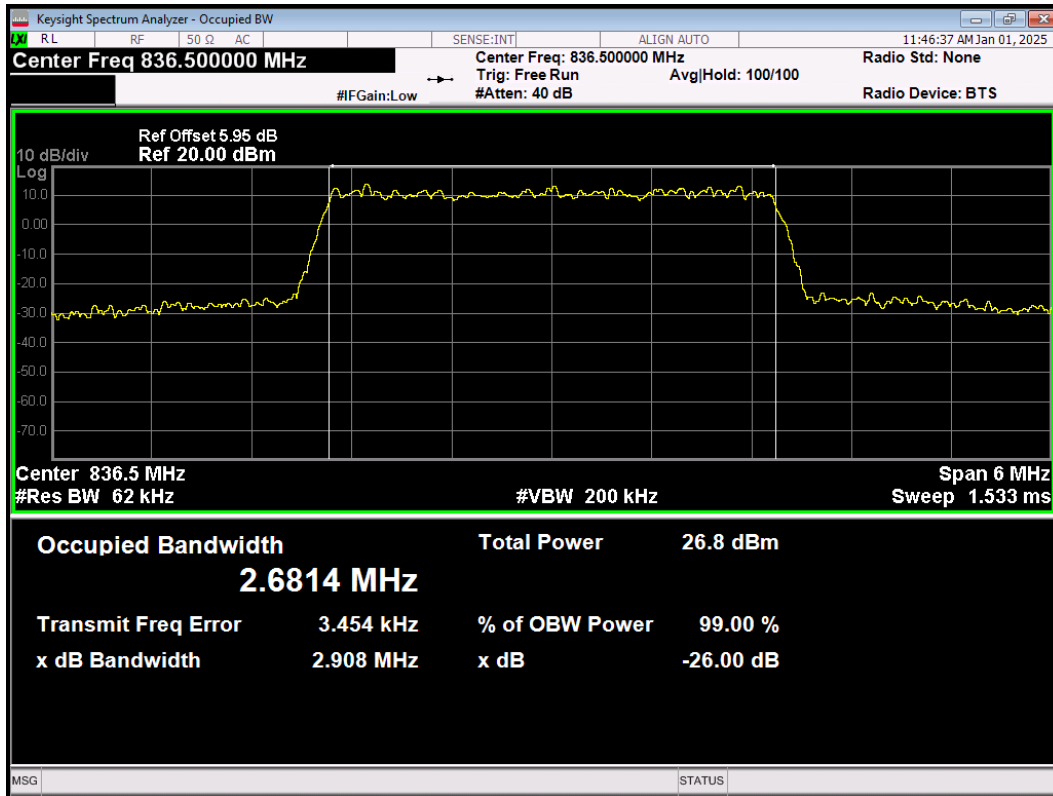
LTE Band26(824-849) 16QAM BW=3MHz Channel=26915 RB Size=15 Position=#0
