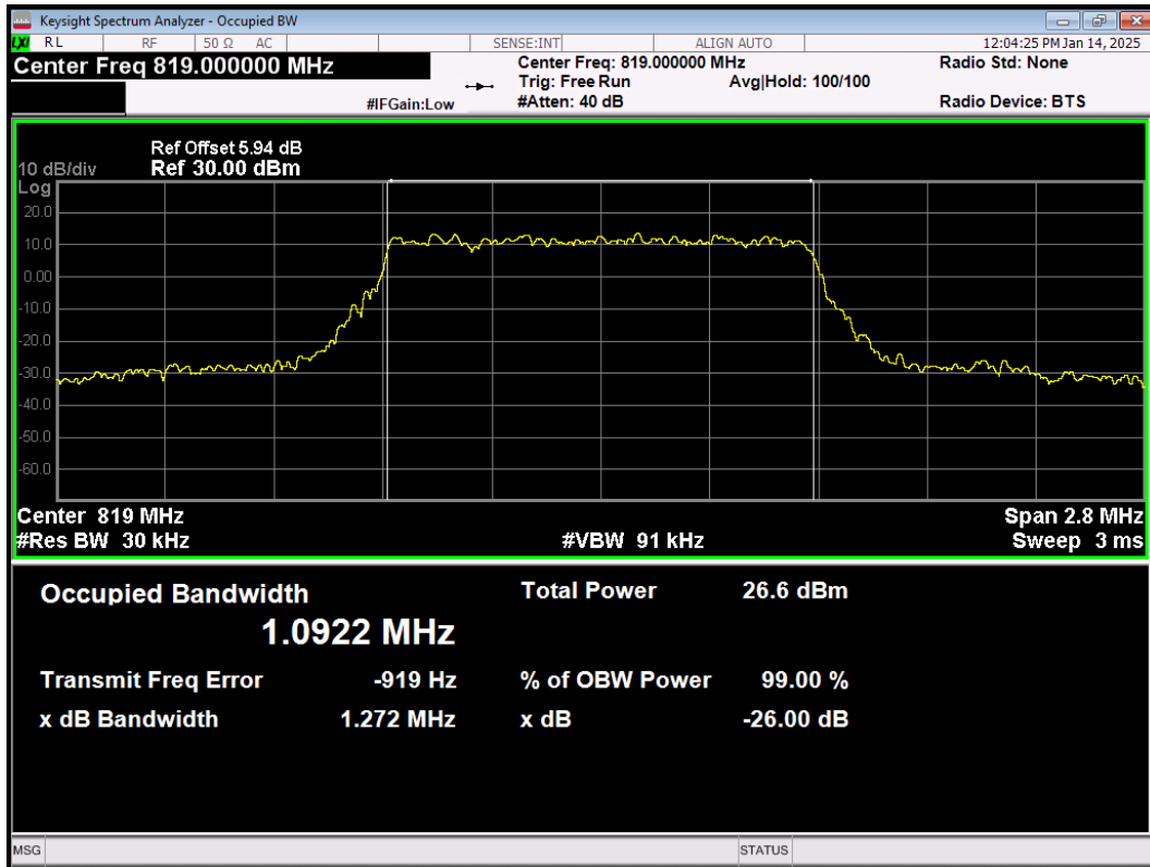
LTE Band26(814-824) 64QAM BW=1.4MHz Channel=26740 RB Size=6 Position=#0
