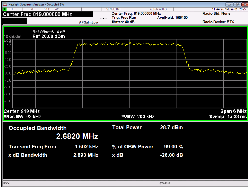
LTE Band26(814-824) 16QAM BW=3MHz Channel=26740 RB Size=15 Position=#0
