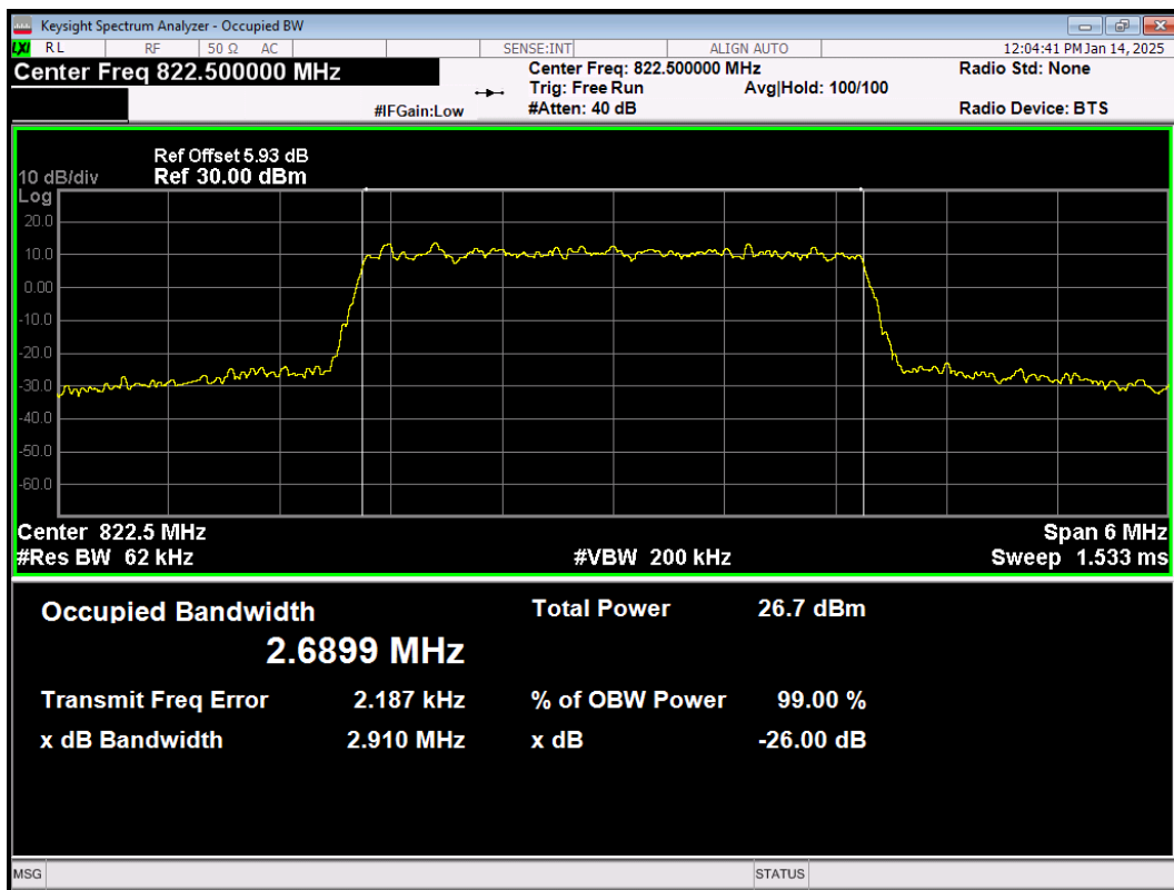
LTE Band26(814-824) 64QAM BW=3MHz Channel=26775 RB Size=15 Position=#0
