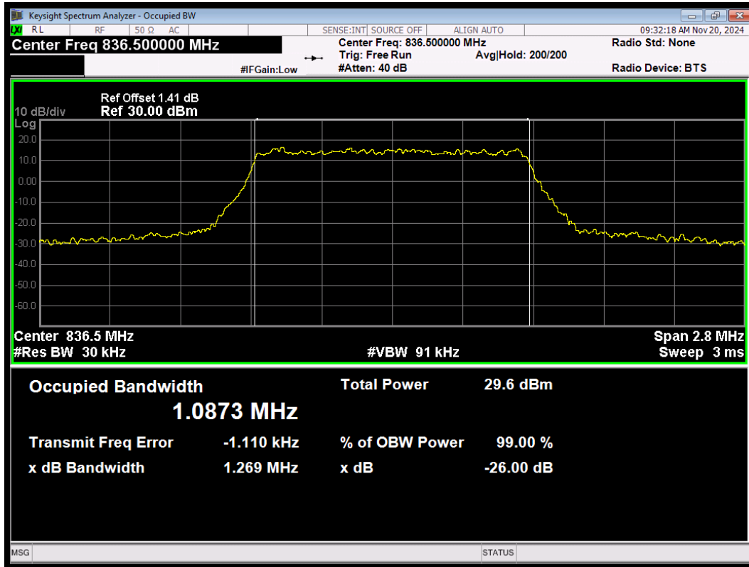
LTE Band26 (824-849) 16QAM BW=1.4MHz Channel=26915 RB Size=6 Position=#0
