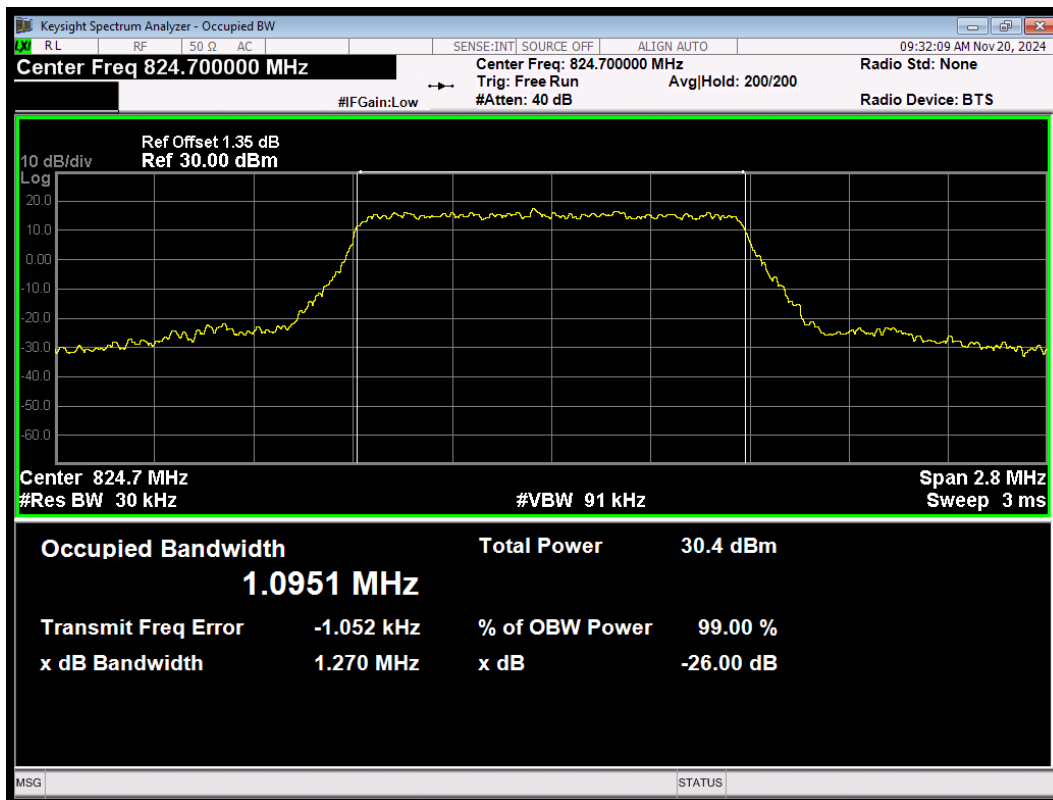
LTE Band26 (824-849) QPSK BW=1.4MHz Channel=26797 RB Size=6 Position=#0
