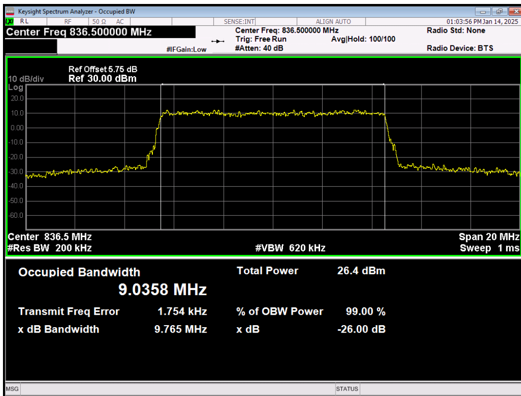
LTE Band26(824-849) 64QAM BW=10MHz Channel=26915 RB Size=50 Position=#0
