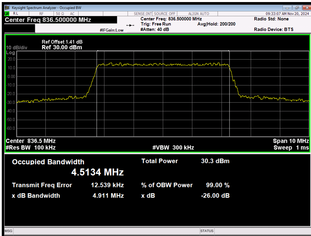
LTE Band26 (824-849) QPSK BW=5MHz Channel=26915 RB Size=25 Position=#0
