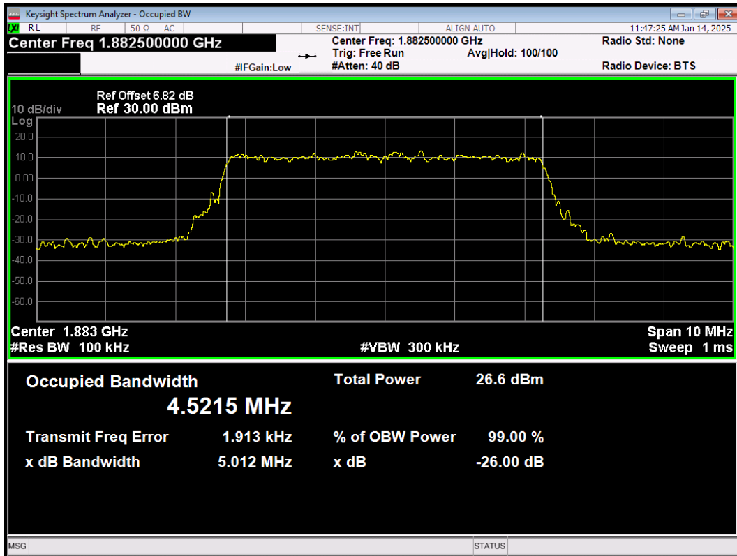
LTE Band25 64QAM BW=5MHz Channel=26365 RB Size=25 Position=#0
