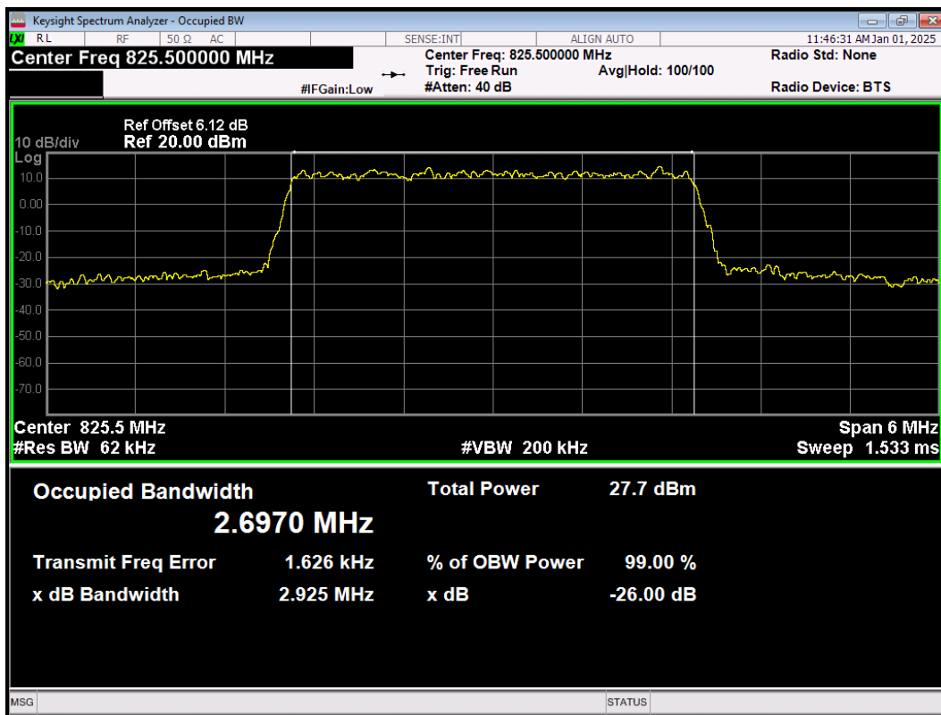
LTE Band26(824-849) 16QAM BW=3MHz Channel=26805 RB Size=15 Position=#0
