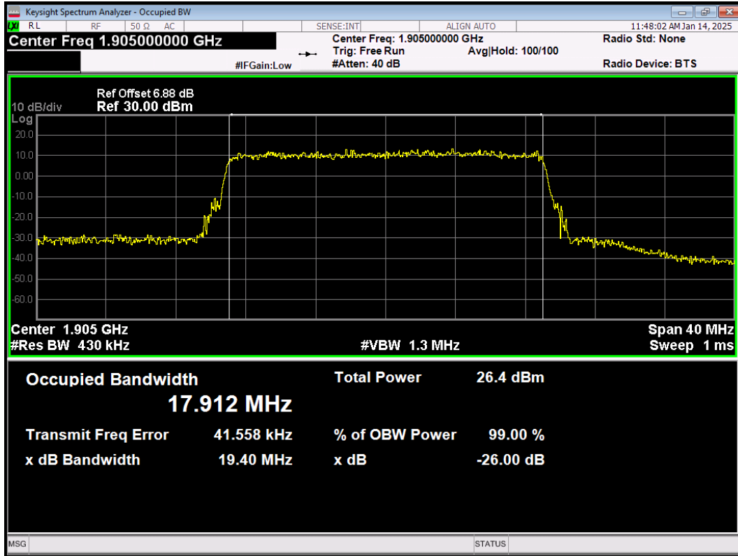
LTE Band25 64QAM BW=20MHz Channel=26590 RB Size=100 Position=#0
