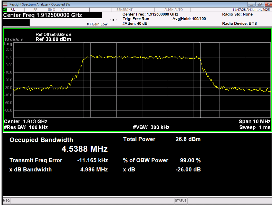
LTE Band25 64QAM BW=5MHz Channel=26665 RB Size=25 Position=#0
