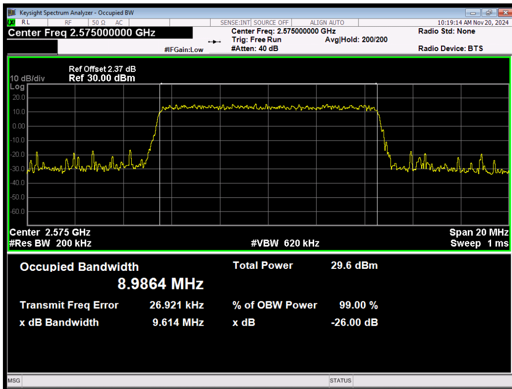
LTE Band38 QPSK BW=10MHz Channel=37800 RB Size=50 Position=#0
