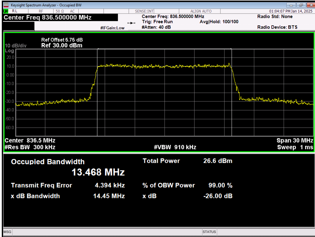
LTE Band26(824-849) 64QAM BW=15MHz Channel=26915 RB Size=75 Position=#0
