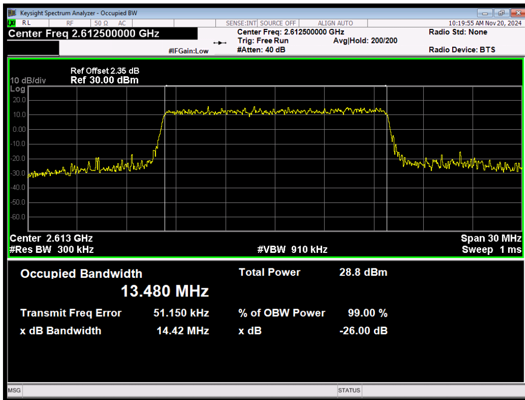
LTE Band38 16QAM BW=15MHz Channel=38175 RB Size=75 Position=#0
