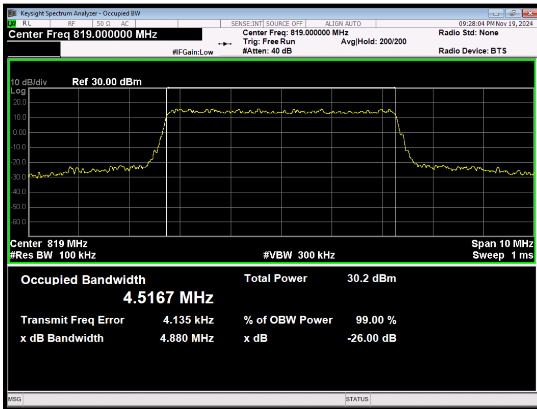
LTE Band26 (814-824) QPSK BW=5MHz Channel=26740 RB Size=25 Position=#0
