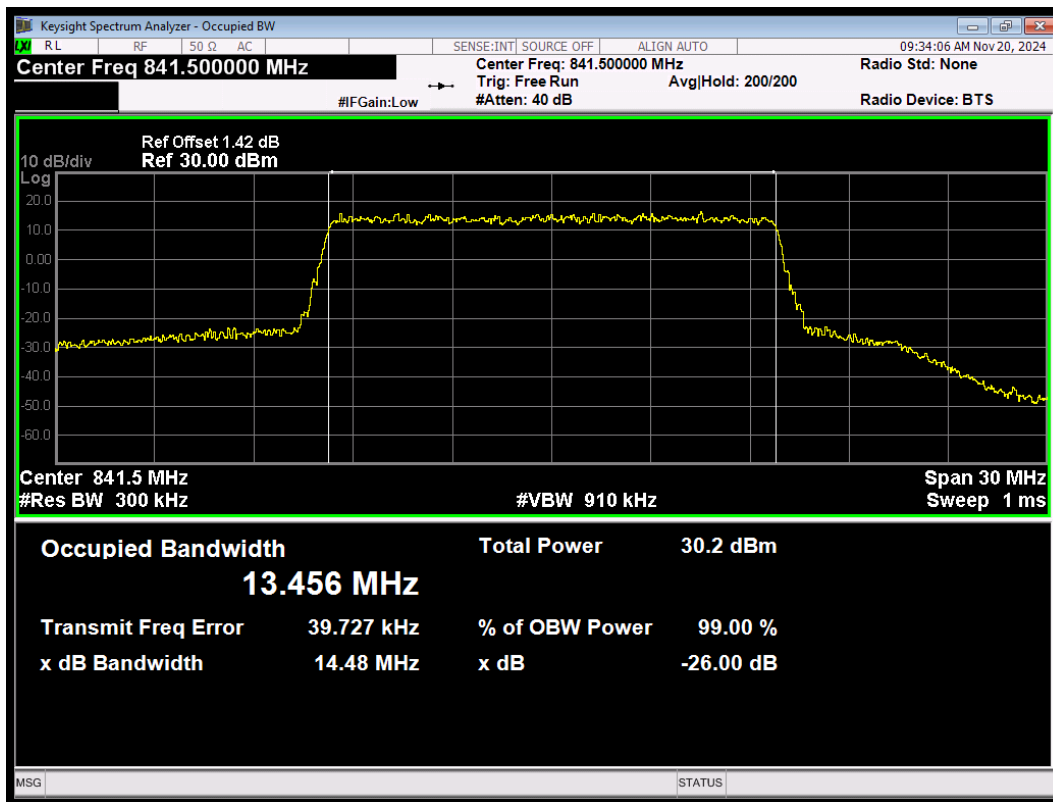
LTE Band26 (824-849) QPSK BW=15MHz Channel=26965 RB Size=75 Position=#0
