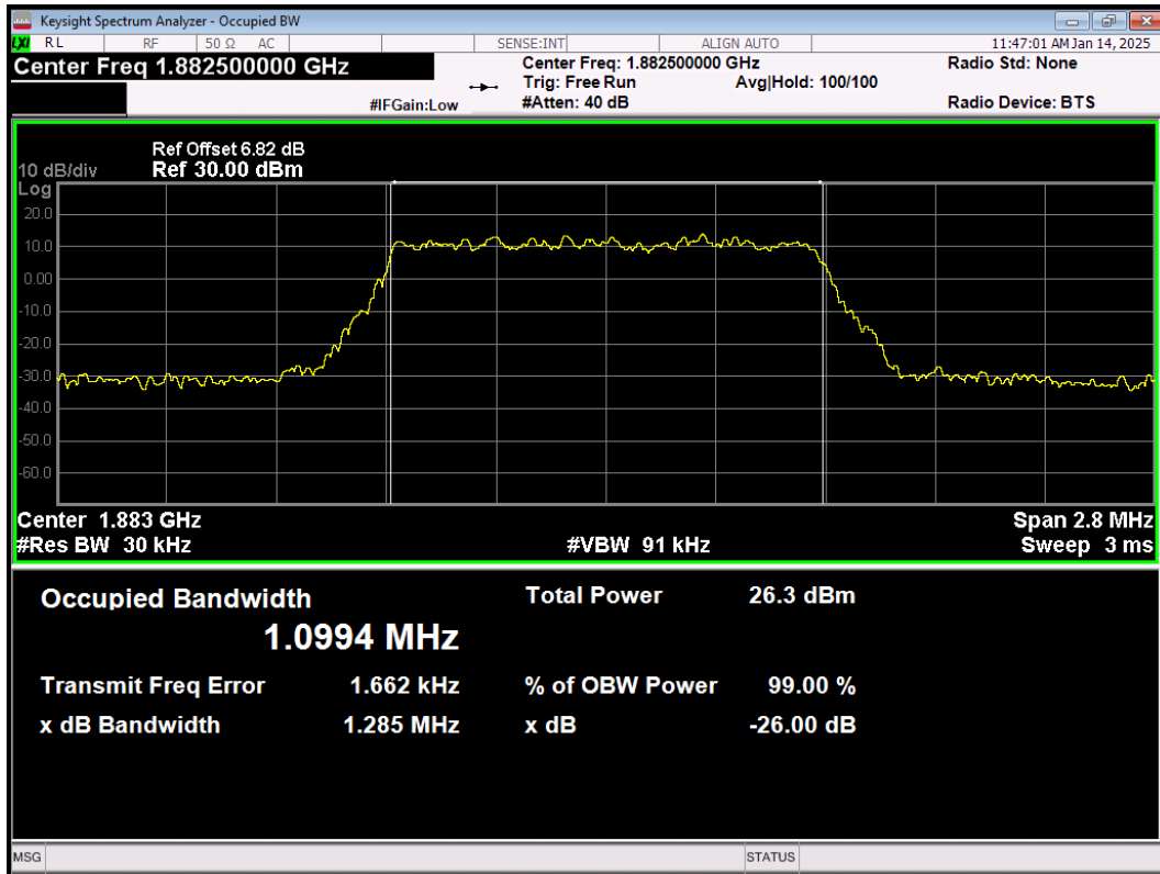
LTE Band25 64QAM BW=1.4MHz Channel=26365 RB Size=6 Position=#0
