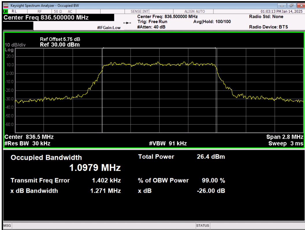
LTE Band26(824-849) 64QAM BW=1.4MHz Channel=26915 RB Size=6 Position=#0
