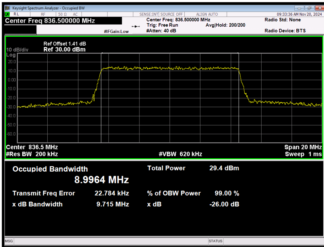
LTE Band26 (824-849) 16QAM BW=10MHz Channel=26915 RB Size=50 Position=#0
