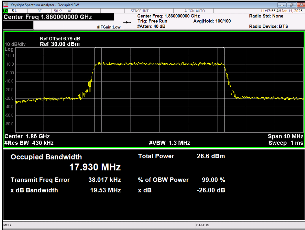
LTE Band25 64QAM BW=20MHz Channel=26140 RB Size=100 Position=#0
