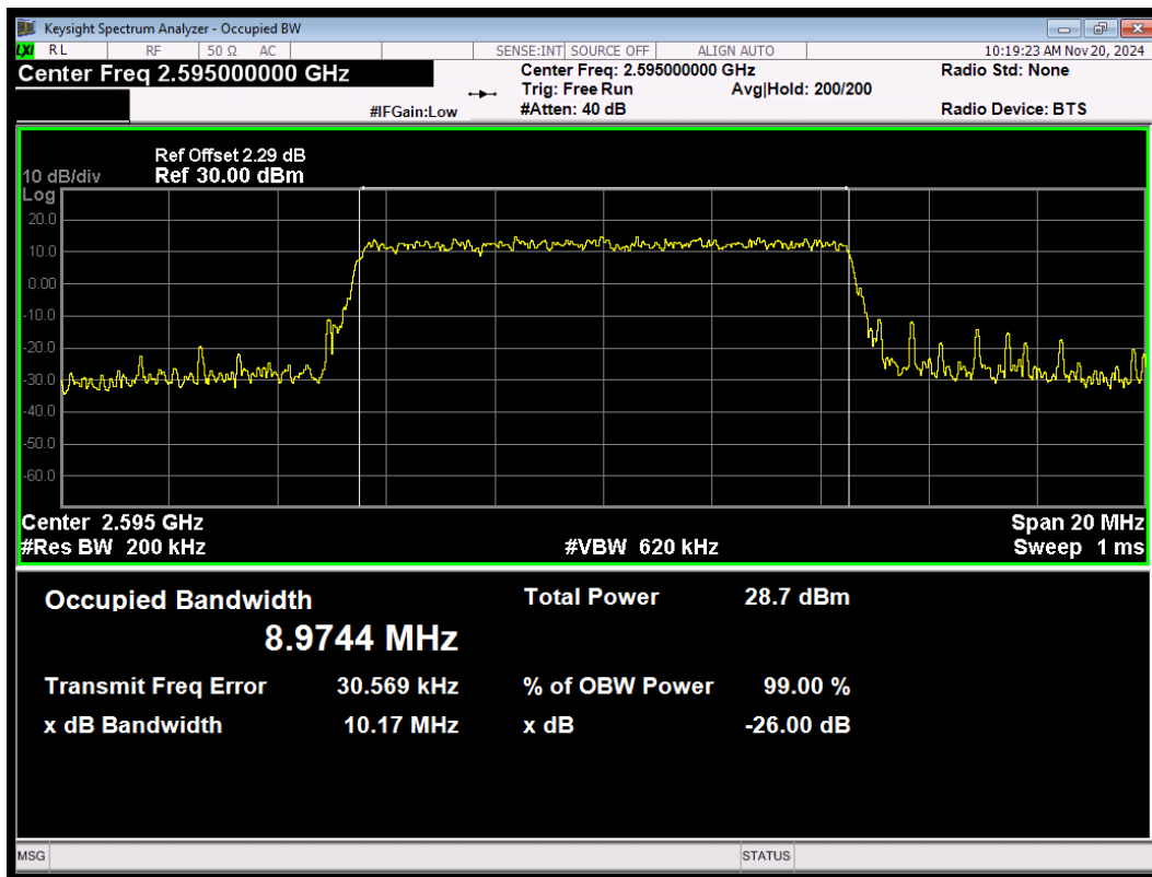
LTE Band38 16QAM BW=10MHz Channel=38000 RB Size=50 Position=#0
