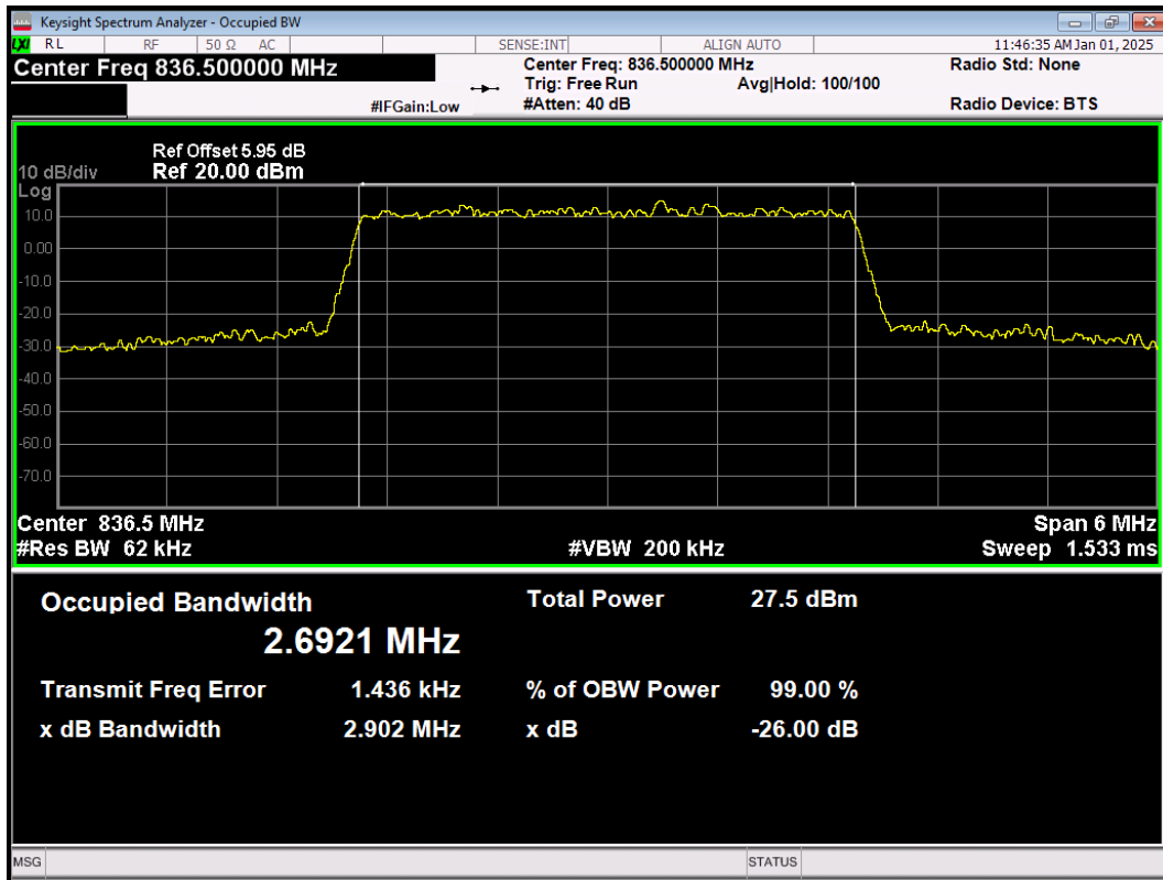
LTE Band26(824-849) QPSK BW=3MHz Channel=26915 RB Size=15 Position=#0
