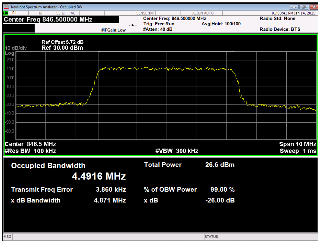
LTE Band26(824-849) 64QAM BW=5MHz Channel=27015 RB Size=25 Position=#0
