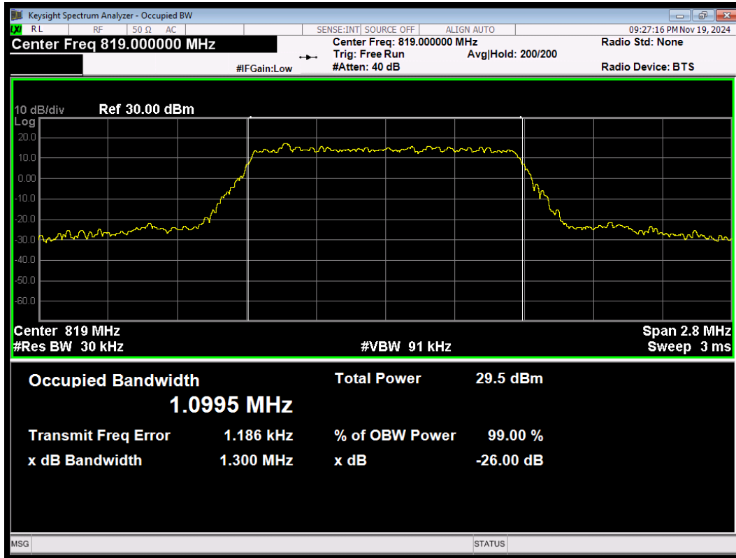
LTE Band26 (814-824) 16QAM BW=1.4MHz Channel=26740 RB Size=6 Position=#0
