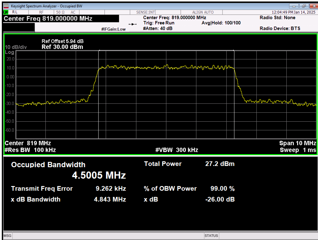
LTE Band26(814-824) 64QAM BW=5MHz Channel=26740 RB Size=25 Position=#0
