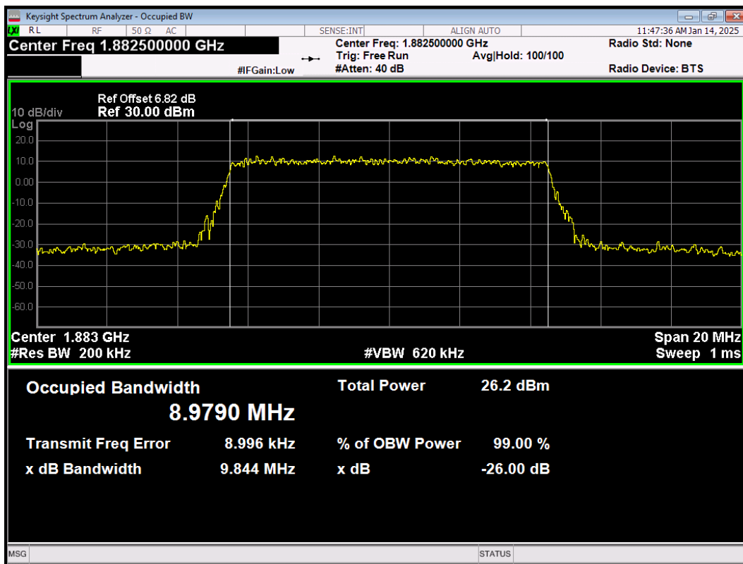
LTE Band25 64QAM BW=10MHz Channel=26365 RB Size=50 Position=#0
