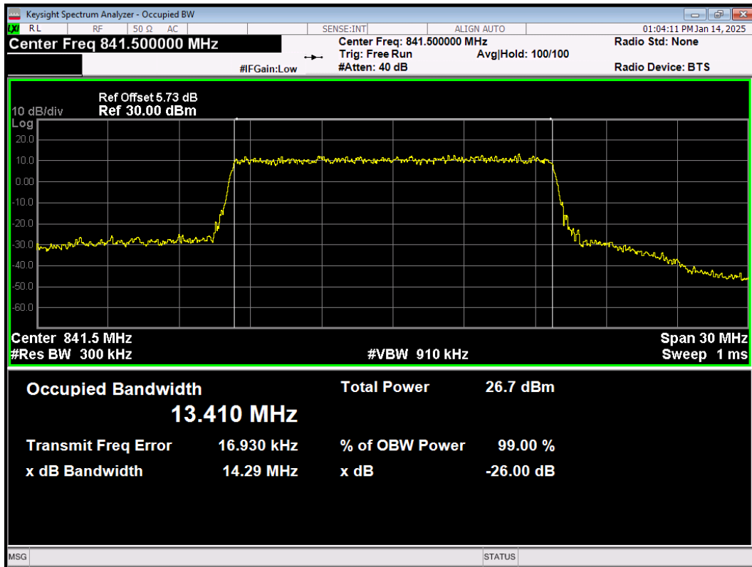
LTE Band26(824-849) 64QAM BW=15MHz Channel=26965 RB Size=75 Position=#0
