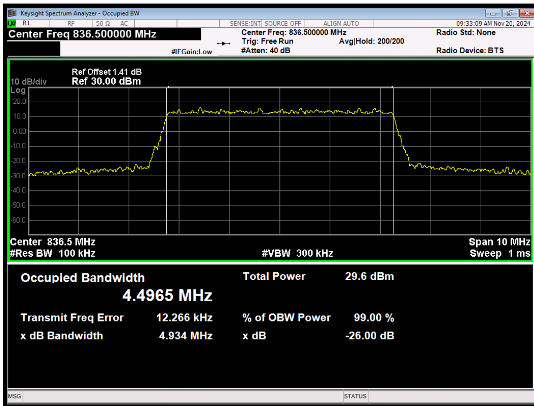
LTE Band26 (824-849) 16QAM BW=5MHz Channel=26915 RB Size=25 Position=#0
