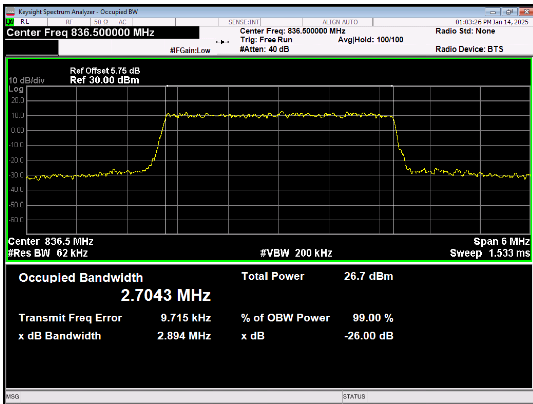
LTE Band26(824-849) 64QAM BW=3MHz Channel=26915 RB Size=15 Position=#0
