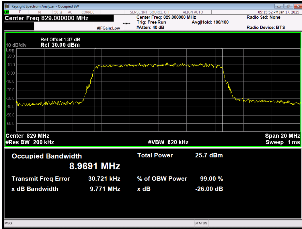
LTE Band26(824-849) 64QAM BW=10MHz Channel=26840 RB Size=50 Position=#0
