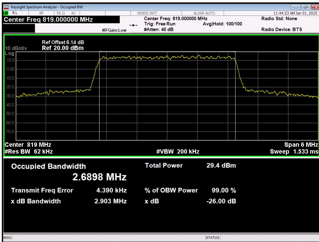
LTE Band26(814-824) QPSK BW=3MHz Channel=26740 RB Size=15 Position=#0
