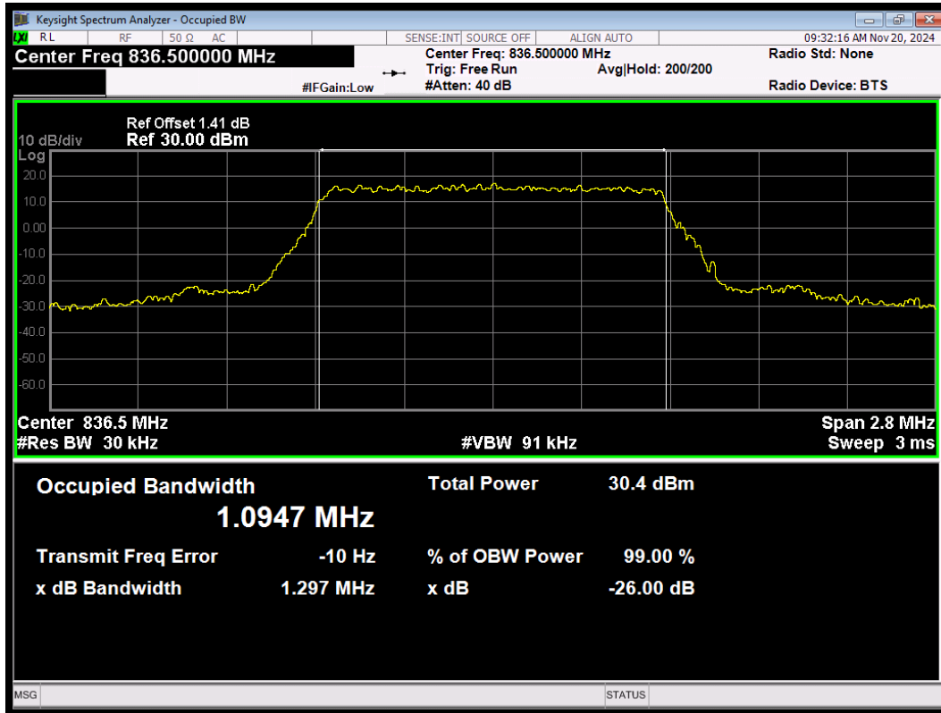
LTE Band26 (824-849) QPSK BW=1.4MHz Channel=26915 RB Size=6 Position=#0
