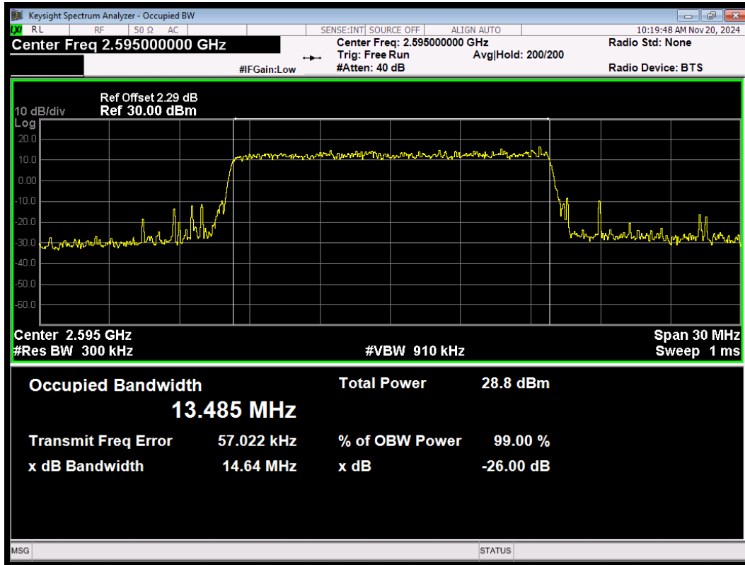
LTE Band38 16QAM BW=15MHz Channel=38000 RB Size=75 Position=#0
