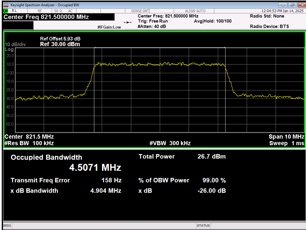
LTE Band26(814-824) 64QAM BW=5MHz Channel=26765 RB Size=25 Position=#0
