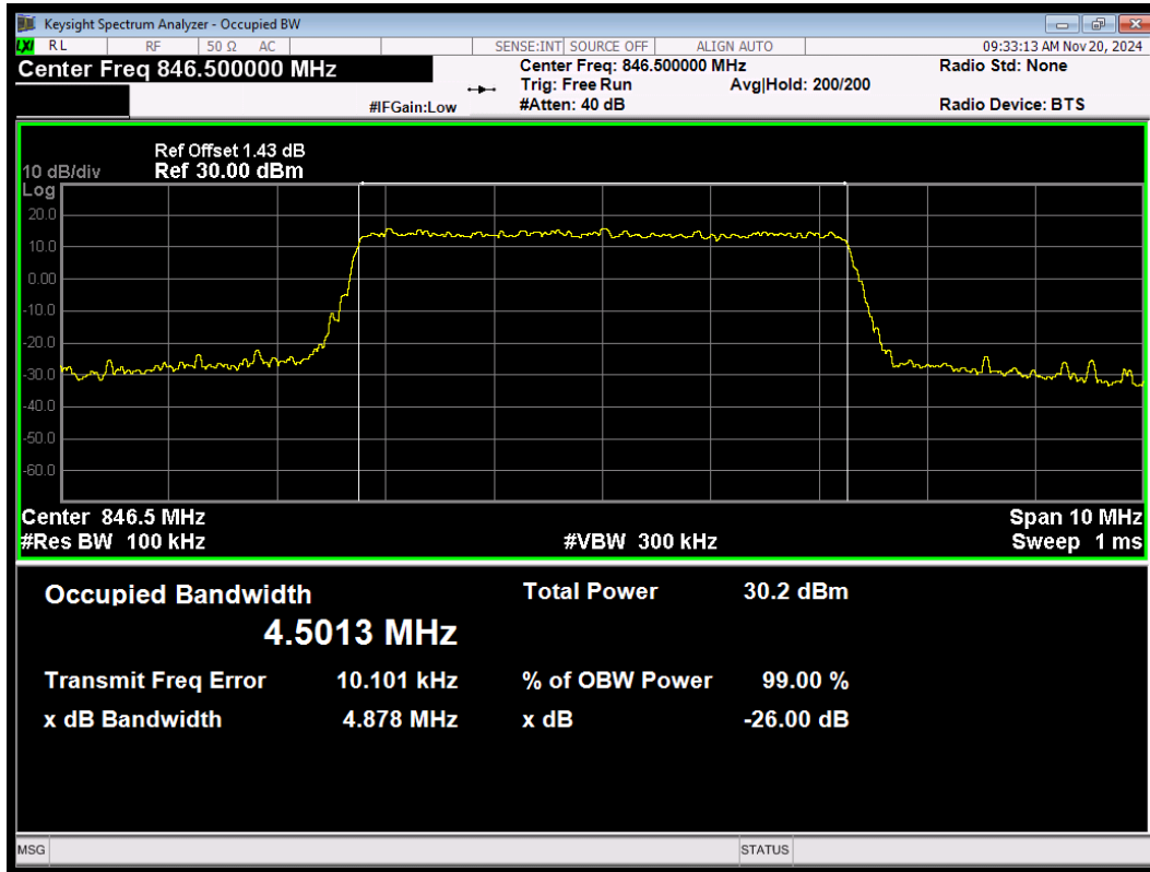
LTE Band26 (824-849) QPSK BW=5MHz Channel=27015 RB Size=25 Position=#0
