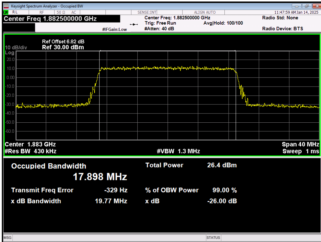
LTE Band25 64QAM BW=20MHz Channel=26365 RB Size=100 Position=#0
