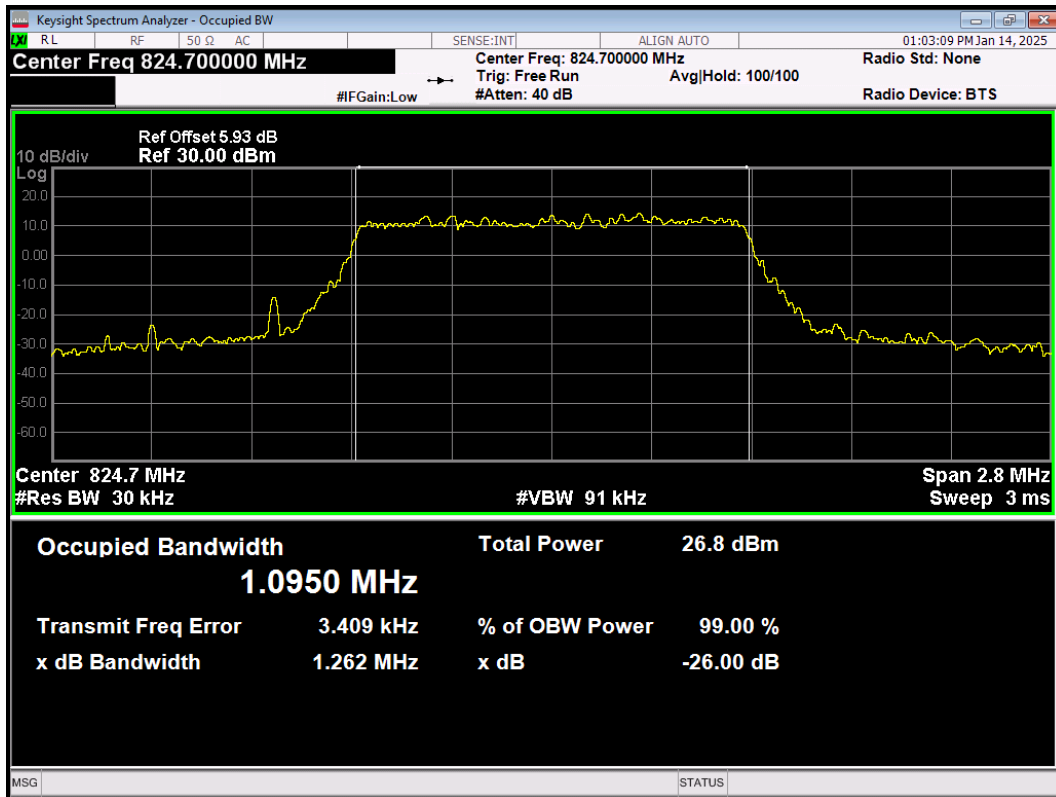
LTE Band26(824-849) 64QAM BW=1.4MHz Channel=26797 RB Size=6 Position=#0
