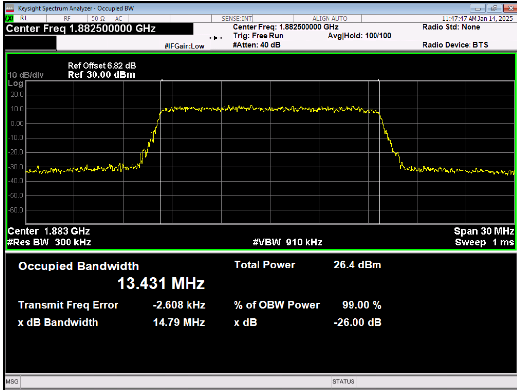
LTE Band25 64QAM BW=15MHz Channel=26365 RB Size=75 Position=#0
