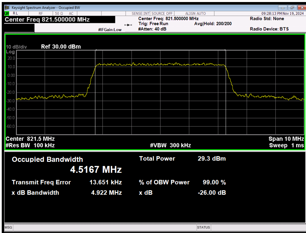
LTE Band26 (814-824) 16QAM BW=5MHz Channel=26765 RB Size=25 Position=#0
