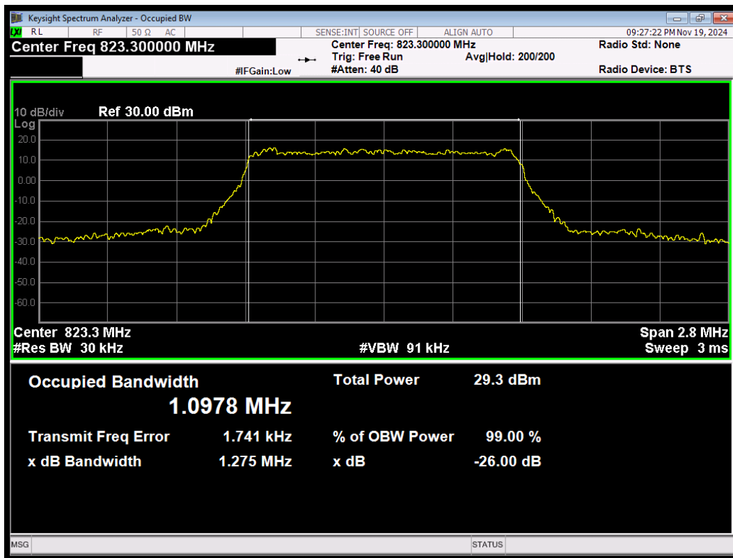
LTE Band26 (814-824) 16QAM BW=1.4MHz Channel=26783 RB Size=6 Position=#0
