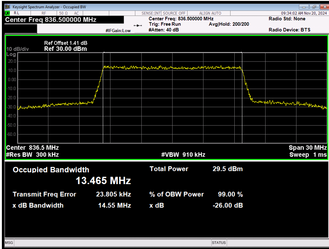
LTE Band26 (824-849) 16QAM BW=15MHz Channel=26915 RB Size=75 Position=#0
