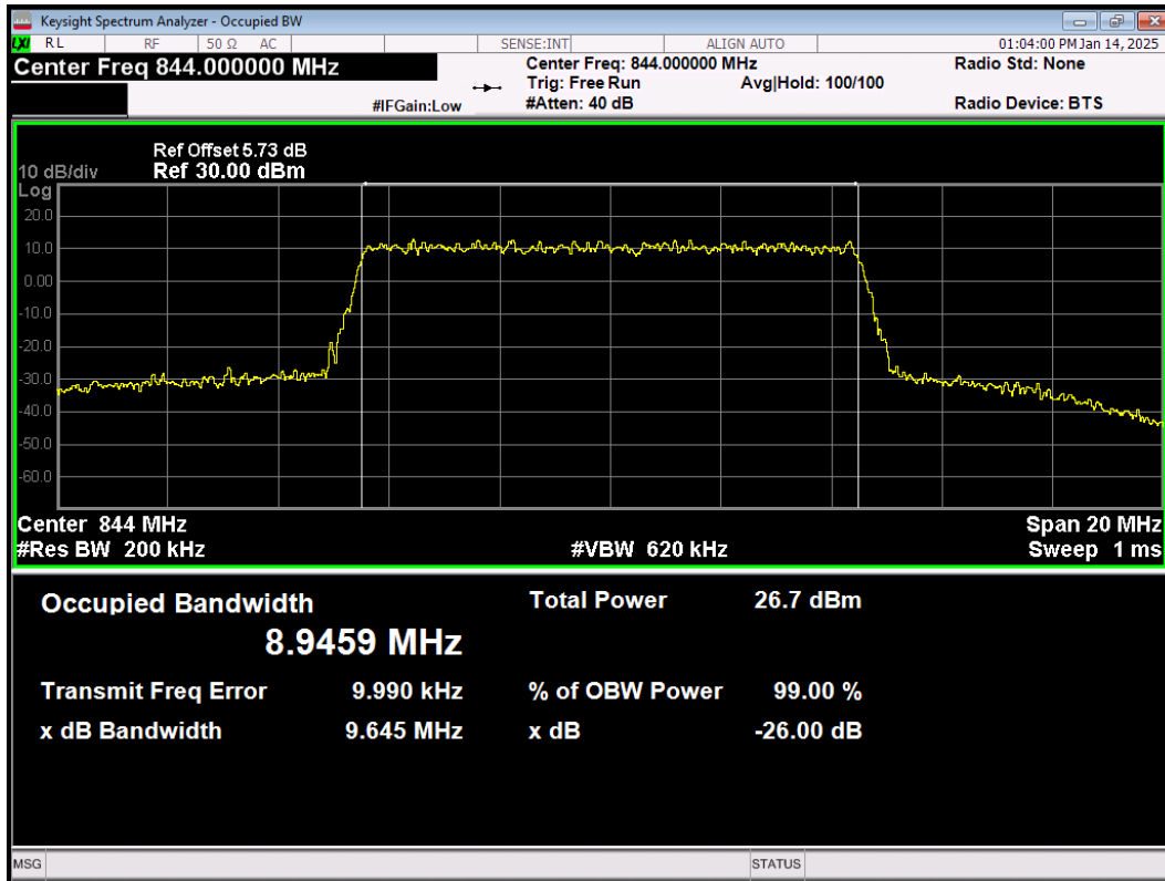
LTE Band26(824-849) 64QAM BW=10MHz Channel=26990 RB Size=50 Position=#0
