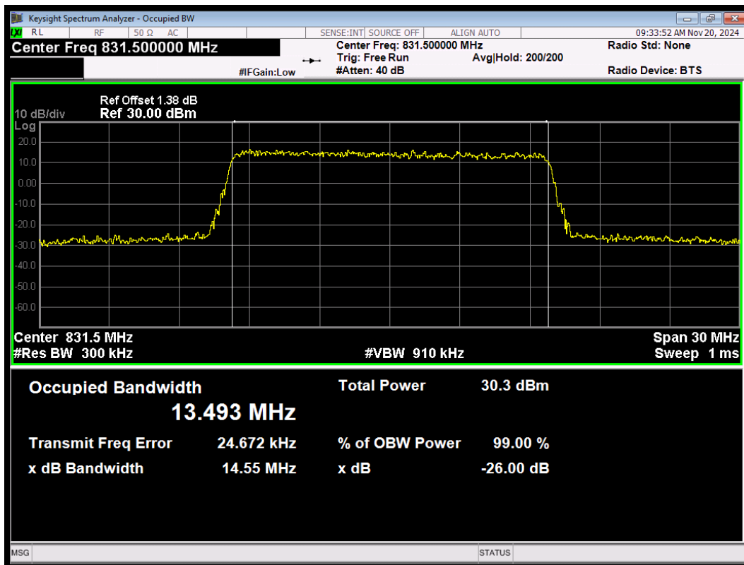
LTE Band26 (824-849) QPSK BW=15MHz Channel=26865 RB Size=75 Position=#0
