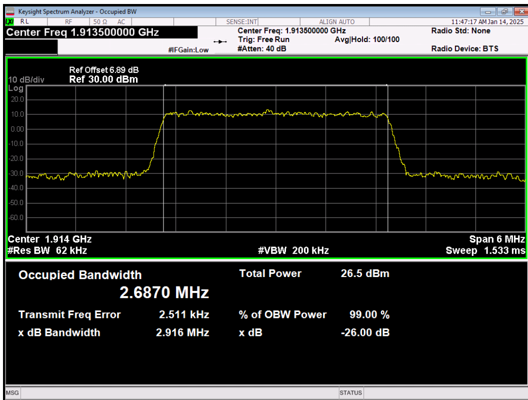
LTE Band25 64QAM BW=3MHz Channel=26675 RB Size=15 Position=#0
