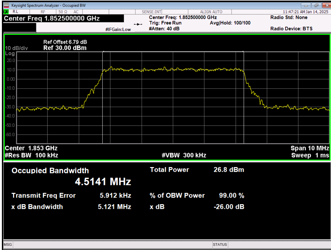
LTE Band25 64QAM BW=5MHz Channel=26065 RB Size=25 Position=#0
