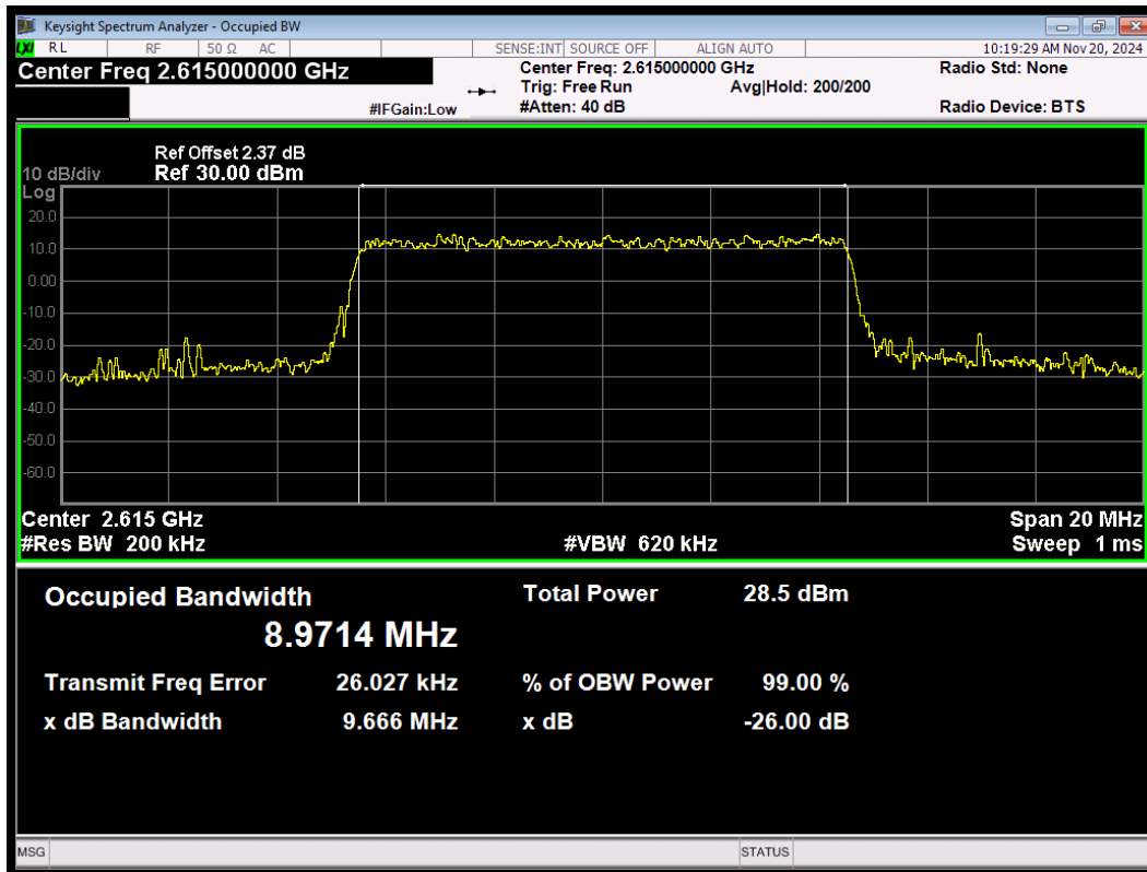
LTE Band38 16QAM BW=10MHz Channel=38200 RB Size=50 Position=#0
