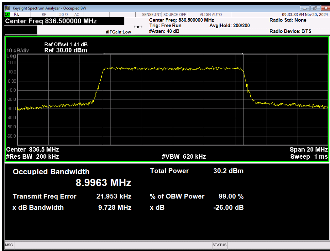
LTE Band26 (824-849) QPSK BW=10MHz Channel=26915 RB Size=50 Position=#0
