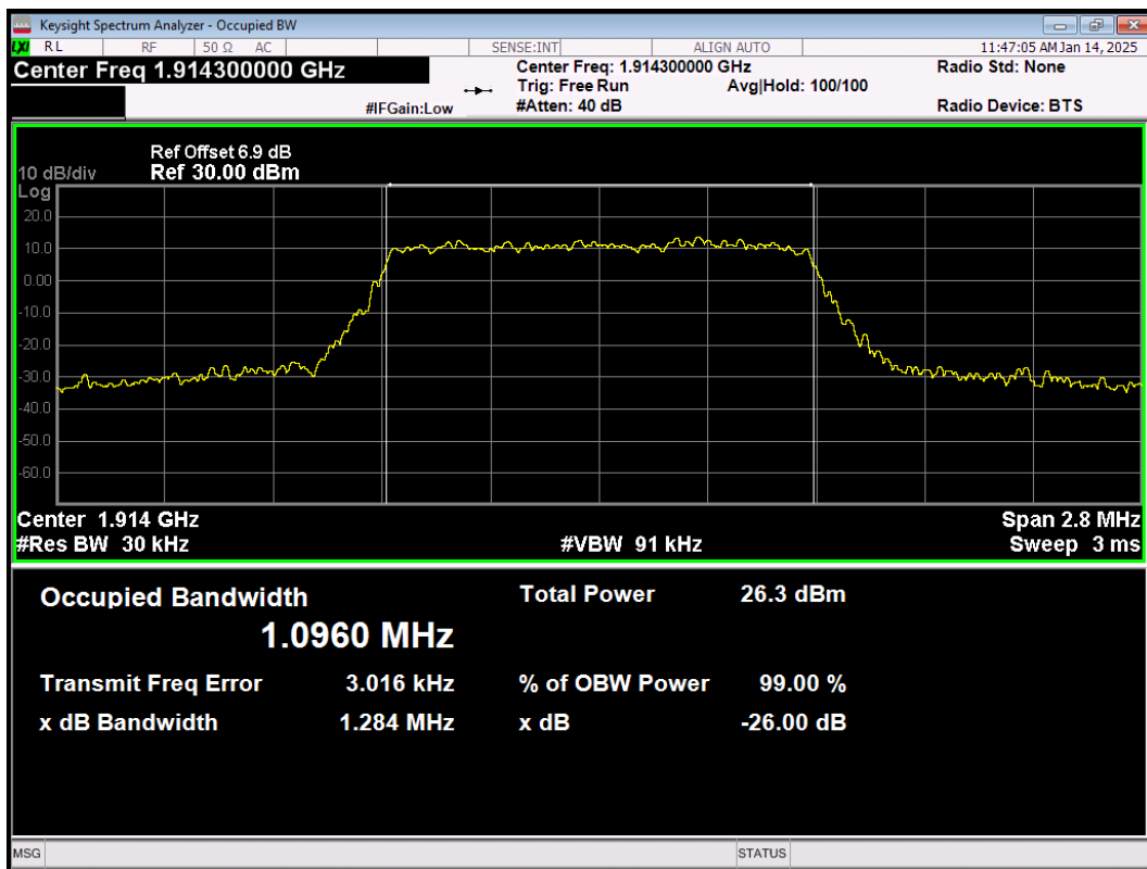
LTE Band25 64QAM BW=1.4MHz Channel=26683 RB Size=6 Position=#0
