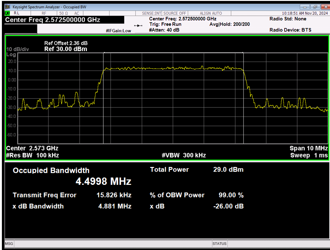
LTE Band38 16QAM BW=5MHz Channel=37775 RB Size=25 Position=#0
