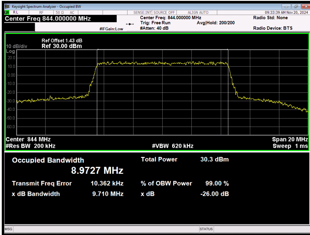
LTE Band26 (824-849) QPSK BW=10MHz Channel=26990 RB Size=50 Position=#0
