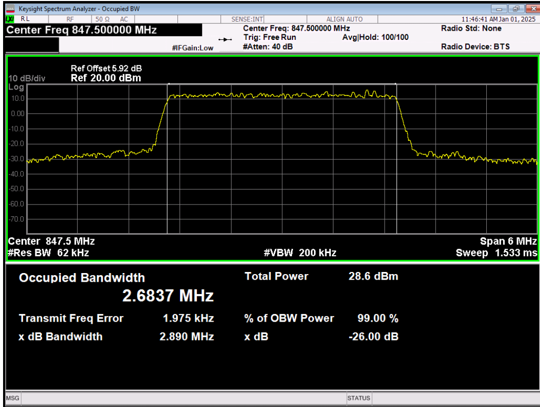
LTE Band26(824-849) QPSK BW=3MHz Channel=27025 RB Size=15 Position=#0
