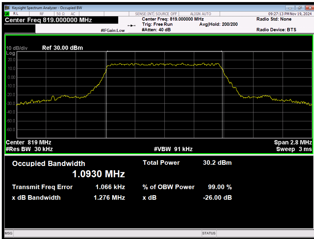
LTE Band26 (814-824) QPSK BW=1.4MHz Channel=26740 RB Size=6 Position=#0
