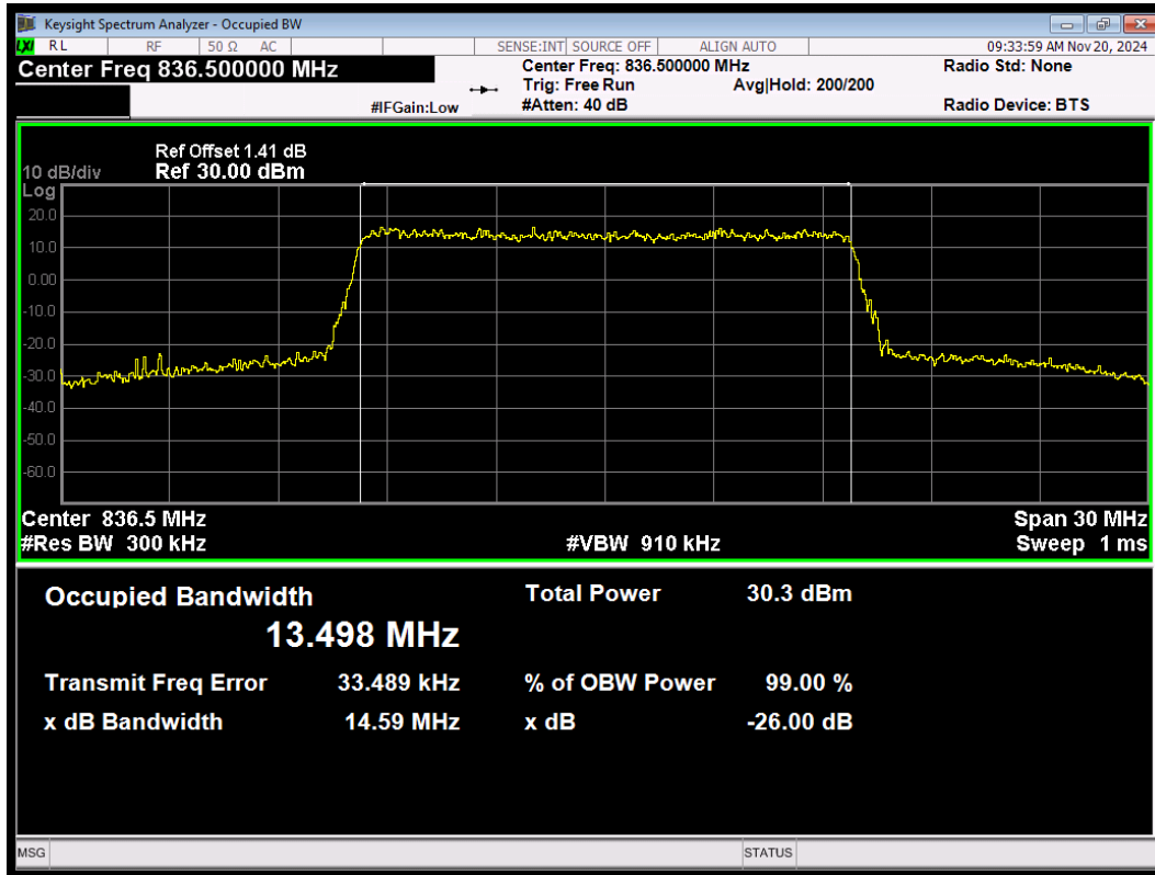
LTE Band26 (824-849) QPSK BW=15MHz Channel=26915 RB Size=75 Position=#0
