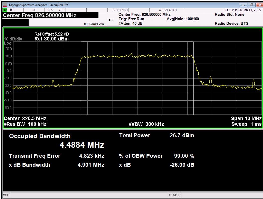
LTE Band26(824-849) 64QAM BW=5MHz Channel=26815 RB Size=25 Position=#0
