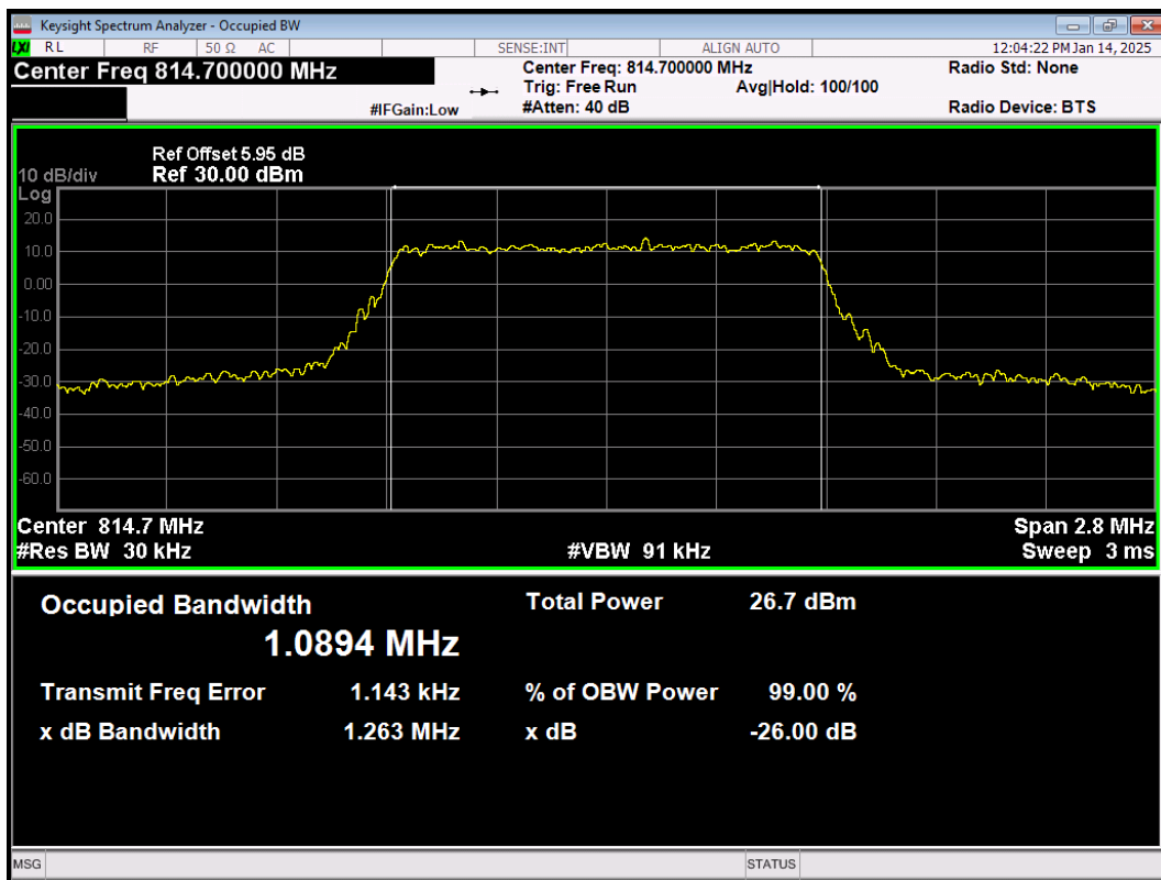
LTE Band26(814-824) 64QAM BW=1.4MHz Channel=26697 RB Size=6 Position=#0
