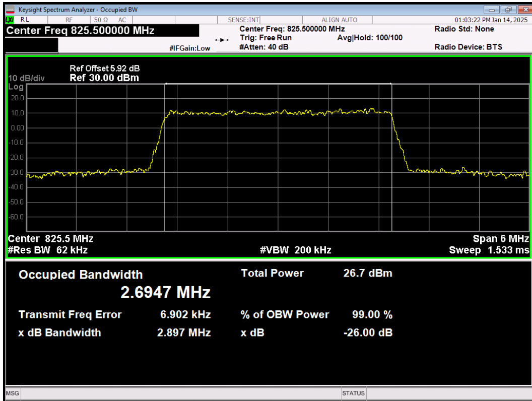
LTE Band26(824-849) 64QAM BW=3MHz Channel=26805 RB Size=15 Position=#0
