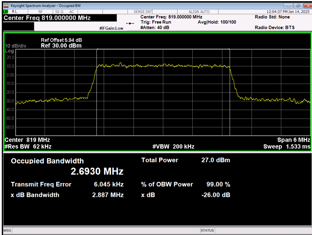
LTE Band26(814-824) 64QAM BW=3MHz Channel=26740 RB Size=15 Position=#0
