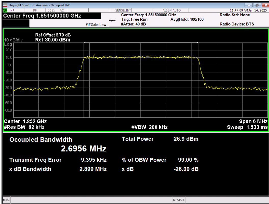
LTE Band25 64QAM BW=3MHz Channel=26055 RB Size=15 Position=#0
