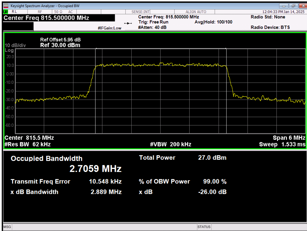
LTE Band26(814-824) 64QAM BW=3MHz Channel=26705 RB Size=15 Position=#0
