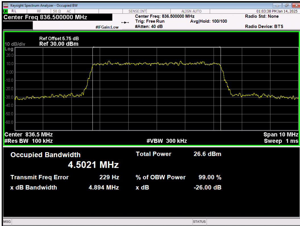
LTE Band26(824-849) 64QAM BW=5MHz Channel=26915 RB Size=25 Position=#0
