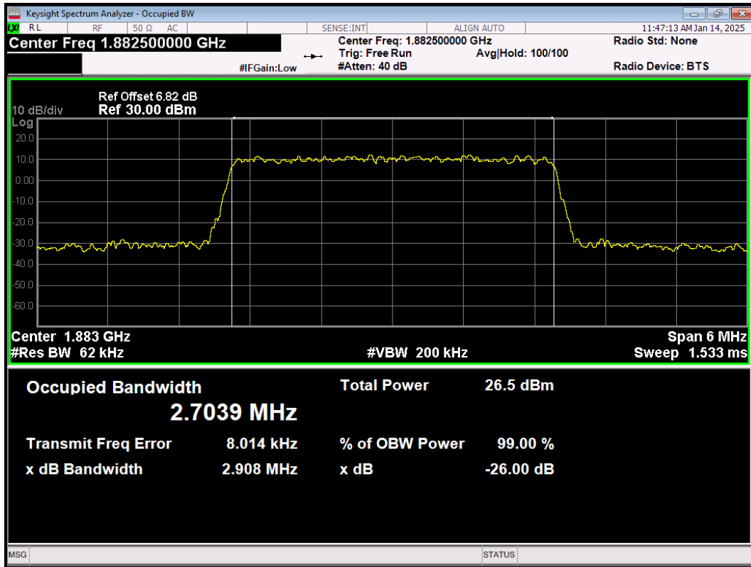
LTE Band25 64QAM BW=3MHz Channel=26365 RB Size=15 Position=#0
