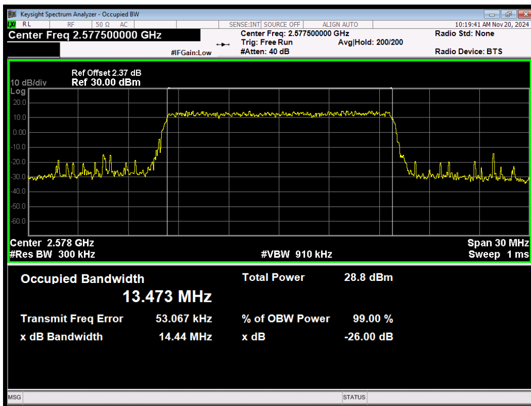
LTE Band38 16QAM BW=15MHz Channel=37825 RB Size=75 Position=#0
