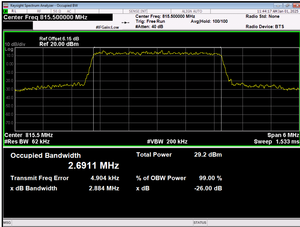
LTE Band26(814-824) QPSK BW=3MHz Channel=26705 RB Size=15 Position=#0
