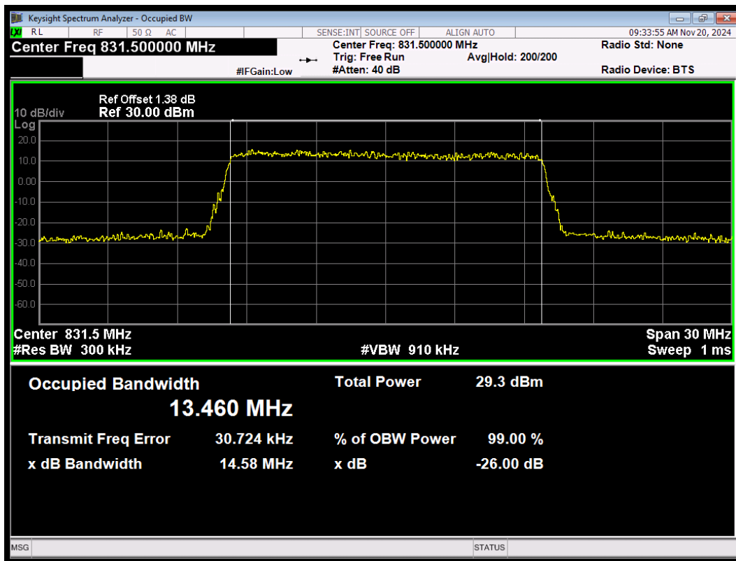
LTE Band26 (824-849) 16QAM BW=15MHz Channel=26865 RB Size=75 Position=#0
