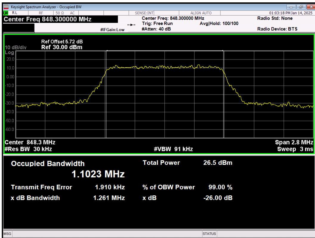
LTE Band26(824-849) 64QAM BW=1.4MHz Channel=27033 RB Size=6 Position=#0
