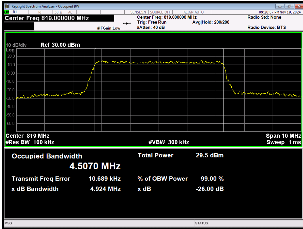
LTE Band26 (814-824) 16QAM BW=5MHz Channel=26740 RB Size=25 Position=#0
