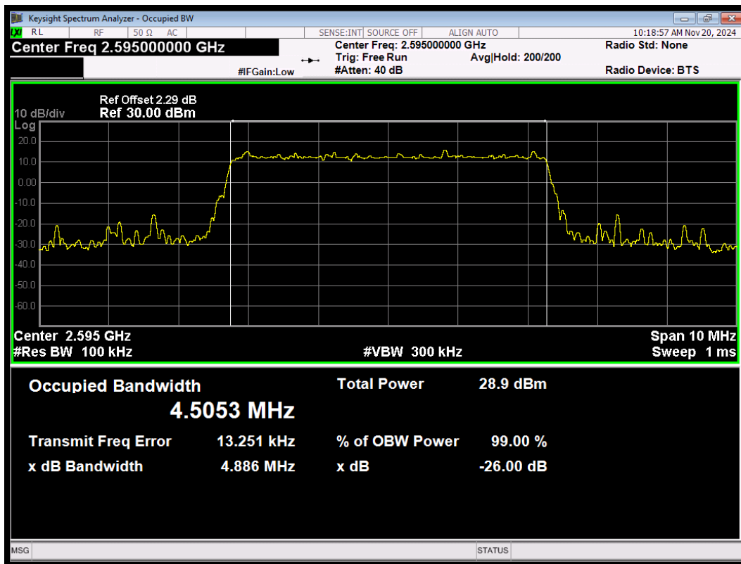
LTE Band38 16QAM BW=5MHz Channel=38000 RB Size=25 Position=#0
