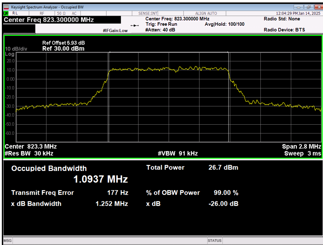
LTE Band26(814-824) 64QAM BW=1.4MHz Channel=26783 RB Size=6 Position=#0
