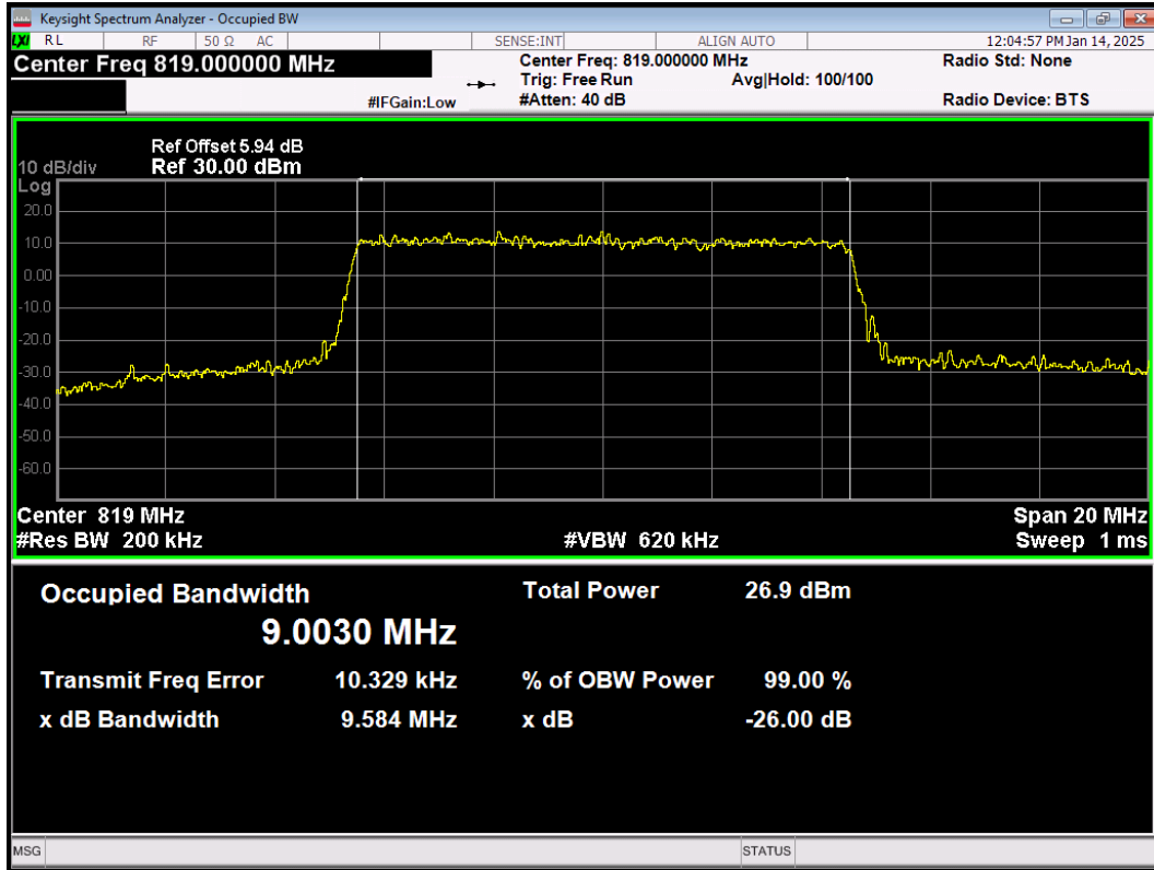
LTE Band26(814-824) 64QAM BW=10MHz Channel=26740 RB Size=50 Position=#0
