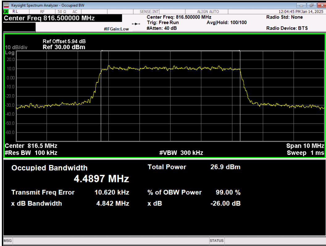
LTE Band26(814-824) 64QAM BW=5MHz Channel=26715 RB Size=25 Position=#0
