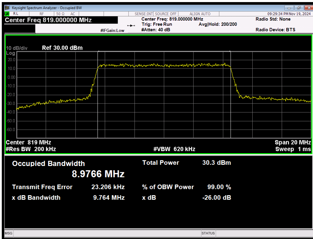
LTE Band26 (814-824) QPSK BW=10MHz Channel=26740 RB Size=50 Position=#0
