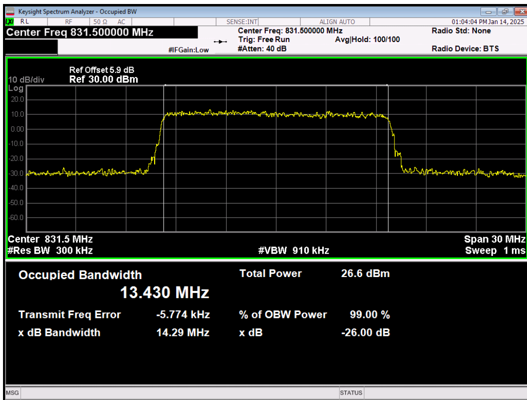
LTE Band26(824-849) 64QAM BW=15MHz Channel=26865 RB Size=75 Position=#0
