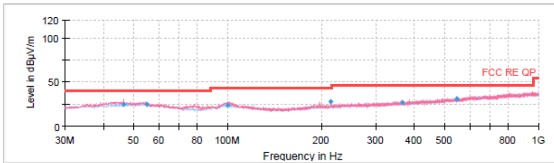
Radiates Emission from 30MHz to 1GHz
