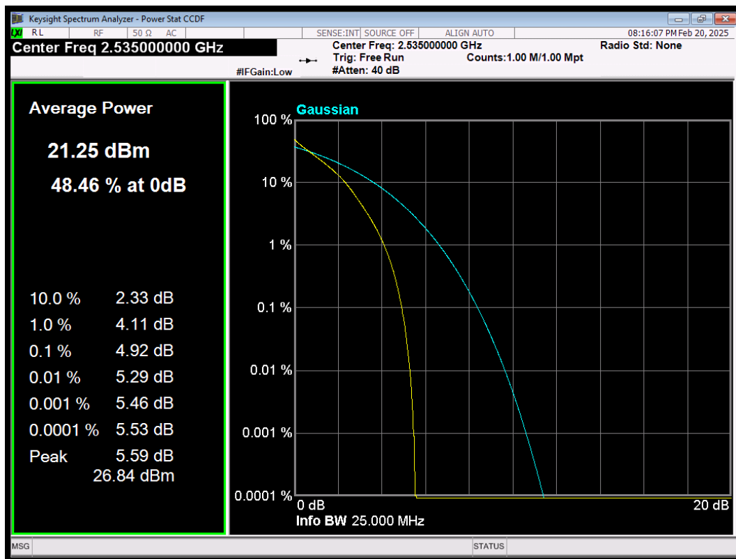
LTE Band7 QPSK BW=5MHz Channel=21100 RB Size=25 Position=#0
