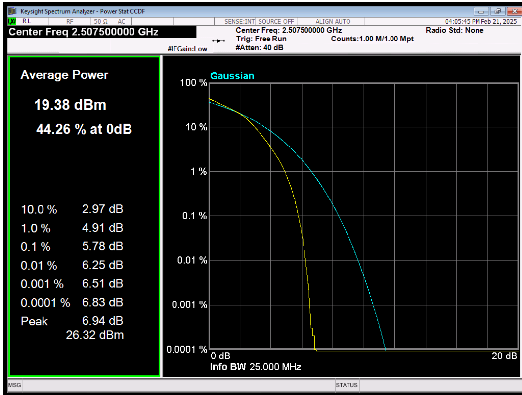
LTE Band7 QAM64 BW=15MHz Channel=20825 RB Size=75 Position=#0
