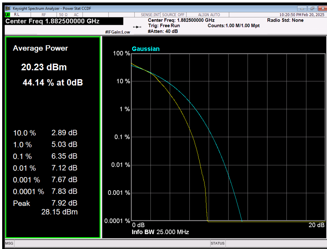
LTE Band25 QAM16 BW=10MHz Channel=26365 RB Size=50 Position=#0
