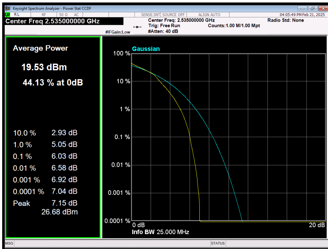
LTE Band7 QAM64 BW=15MHz Channel=21100 RB Size=75 Position=#0
