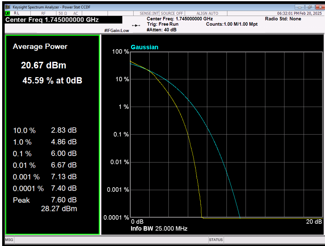
LTE Band4 QAM16 BW=20MHz Channel=20300 RB Size=100 Position=#0
