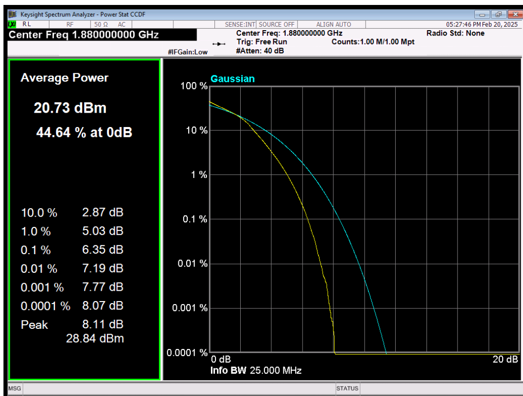
LTE Band2 QAM16 BW=20MHz Channel=18900 RB Size=100 Position=#0
