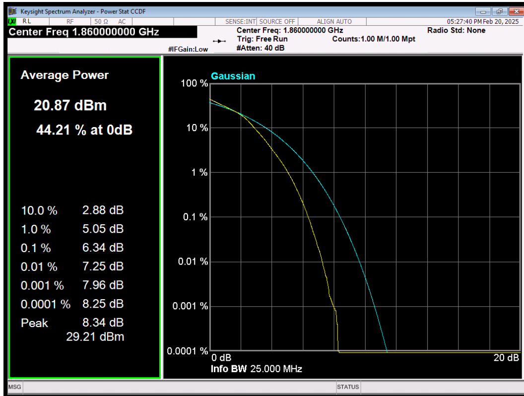
LTE Band2 QAM16 BW=20MHz Channel=18700 RB Size=100 Position=#0
