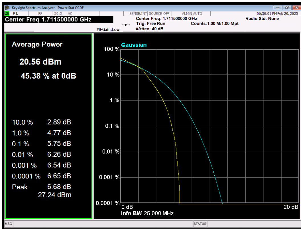
LTE Band4 QAM16 BW=3MHz Channel=19965 RB Size=15 Position=#0
