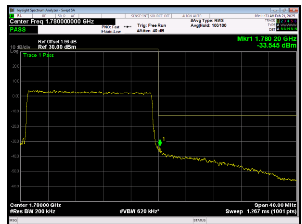
H\LTE Band66 QPSK BW=20MHz Channel=132572 RB Size=100 Position=#0
