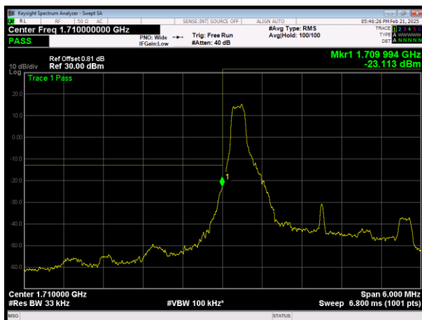
LLTE Band66 QAM64 BW=3MHz Channel=131987 RB Size=1 Position=#0
