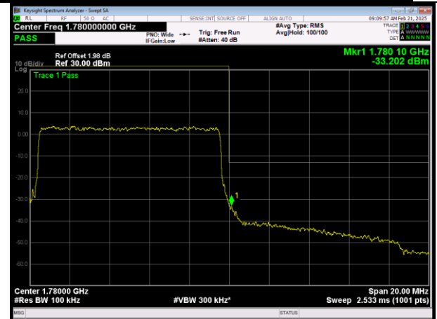
H\LTE Band66 QPSK BW=10MHz Channel=132622 RB Size=50 Position=#0
