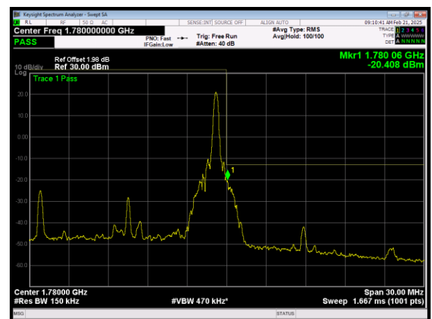
H\LTE Band66 QPSK BW=15MHz Channel=132597 RB Size=1 Position=#Max
