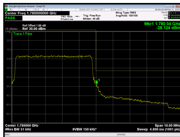
H\LTE Band66 QPSK BW=5MHz Channel=132647 RB Size=25 Position=#0
