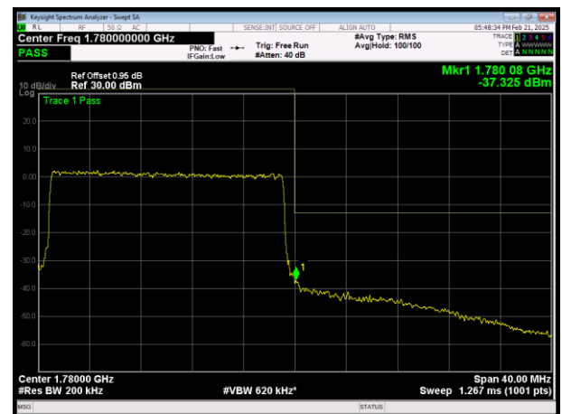
HLTE Band66 QAM64 BW=20MHz Channel=132572 RB Size=100 Position=#0
