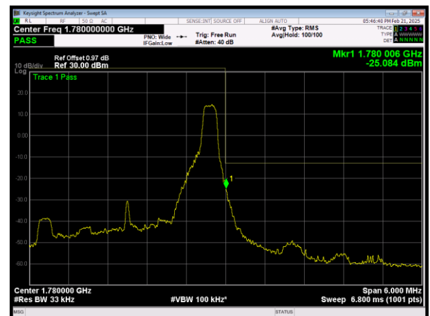
HLTE Band66 QAM64 BW=3MHz Channel=132657 RB Size=1 Position=#Max
