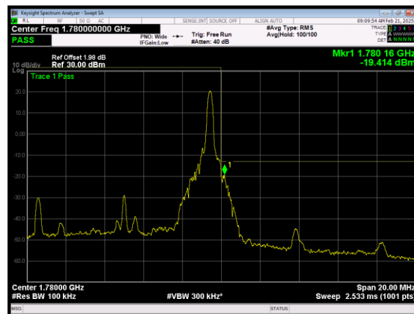
H/LTE Band66 QPSK BW=10MHz Channel=132622 RB Size=1 Position=#Max
