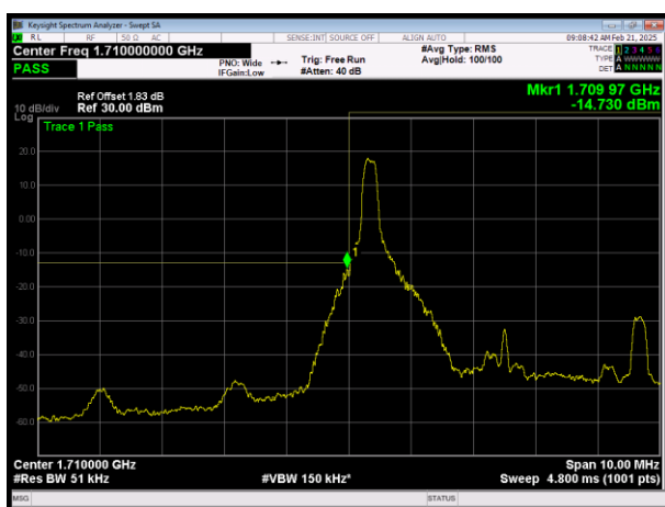
L\LTE Band66 QPSK BW=5MHz Channel=131997 RB Size=1 Position=#0
