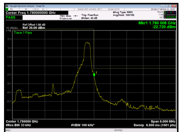
H\LTE Band66 QPSK BW=3MHz Channel=132657 RB Size=1 Position=#Max
