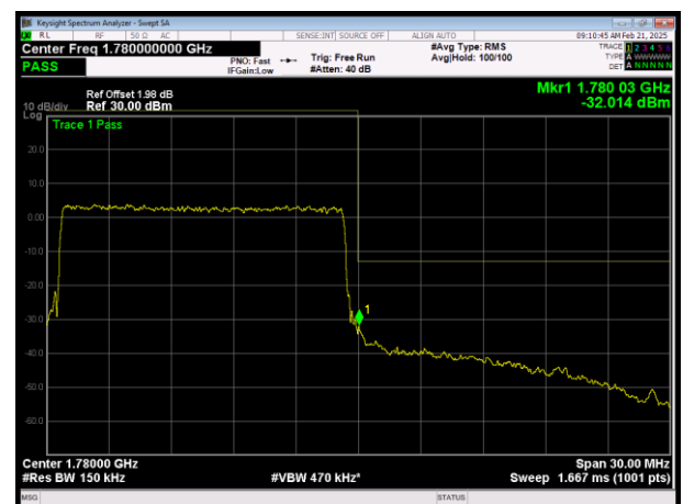
H\LTE Band66 QPSK BW=15MHz Channel=132597 RB Size=75 Position=#0
