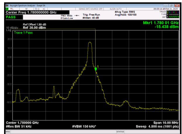
H\LTE Band66 QAM16 BW=5MHz Channel=132647 RB Size=1 Position=#Max
