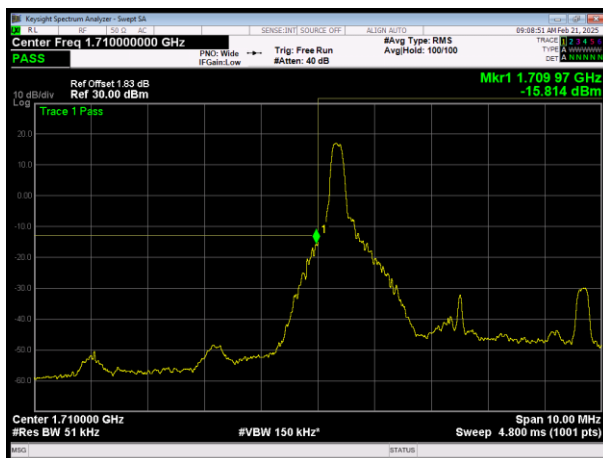
L\LTE Band66 QAM16 BW=5MHz Channel=131997 RB Size=1 Position=#0
