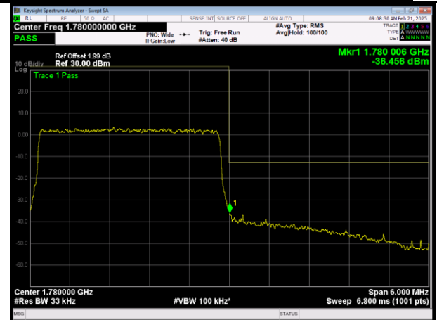
H\LTE Band66 QAM16 BW=3MHz Channel=132657 RB Size=15 Position=#0
