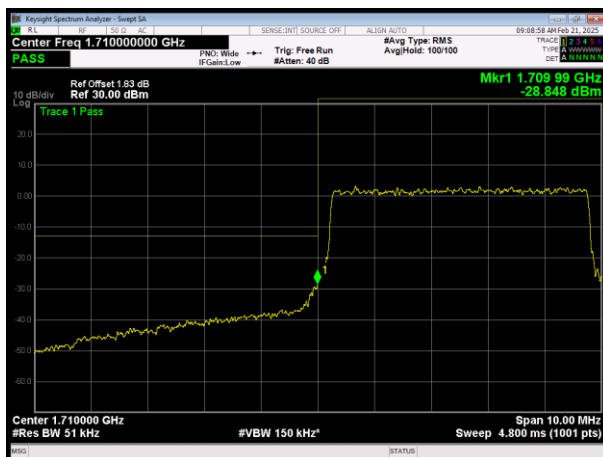
L\LTE Band66 QAM16 BW=5MHz Channel=131997 RB Size=25 Position=#0
