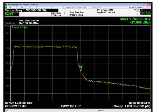
H\LTE Band66 QAM16 BW=5MHz Channel=132647 RB Size=25 Position=#0
