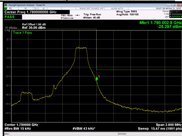
H\LTE Band66 QAM16 BW=1.4MHz Channel=132665 RB Size=1 Position=#Max
