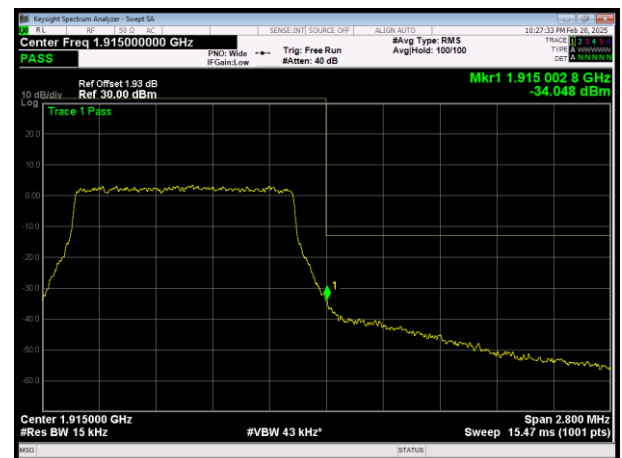
H/LTE Band25 QAM16 BW=1.4MHz Channel=26683 RB Size=6 Position=#0
