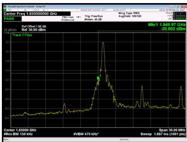
L\LTE Band25 QAM16 BW=15MHz Channel=26115 RB Size=1 Position=#0
