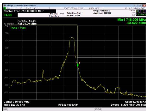
H\LTE Band12 QAM16 BW=3MHz Channel=23165 RB Size=1 Position=#Max
