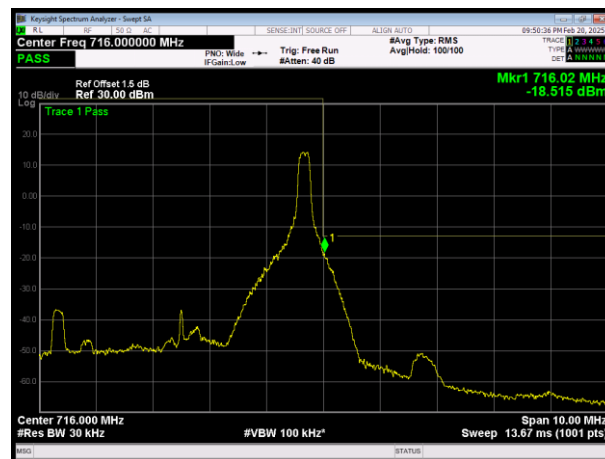
H\LTE Band17 QAM16 BW=5MHz Channel=23825 RB Size=1 Position=#Max
