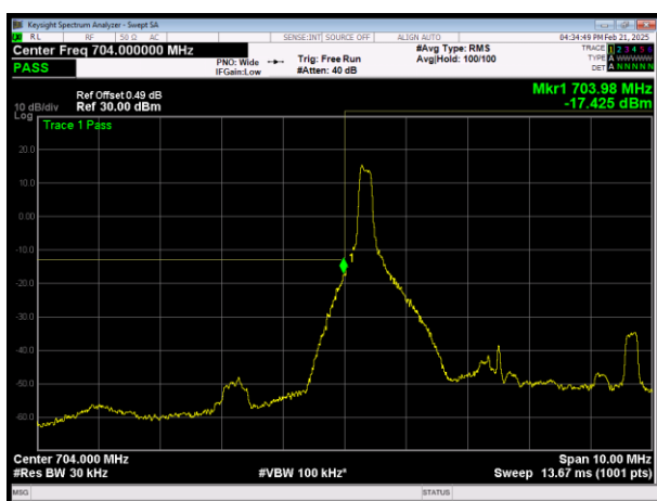
L\LTE Band17 QAM64 BW=5MHz Channel=23755 RB Size=1 Position=#0
