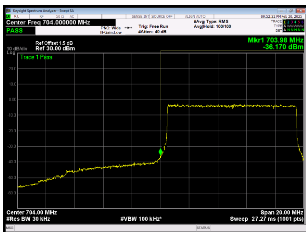
L\LTE Band17 QAM16 BW=10MHz Channel=23780 RB Size=50 Position=#0
