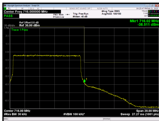
H\LTE Band12 QAM64 BW=10MHz Channel=23130 RB Size=50 Position=#0
