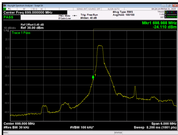
L\LTE Band12 QAM64 BW=3MHz Channel=23025 RB Size=1 Position=#0
