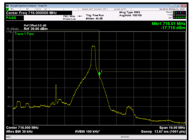
H\LTE Band12 QAM64 BW=5MHz Channel=23155 RB Size=1 Position=#Max
