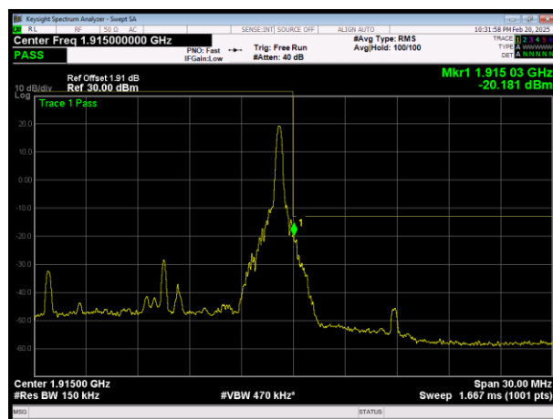
H\LTE Band25 QAM16 BW=15MHz Channel=26615 RB Size=1 Position=#Max
