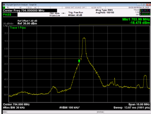
L\LTE Band17 QAM16 BW=5MHz Channel=23755 RB Size=1 Position=#0
