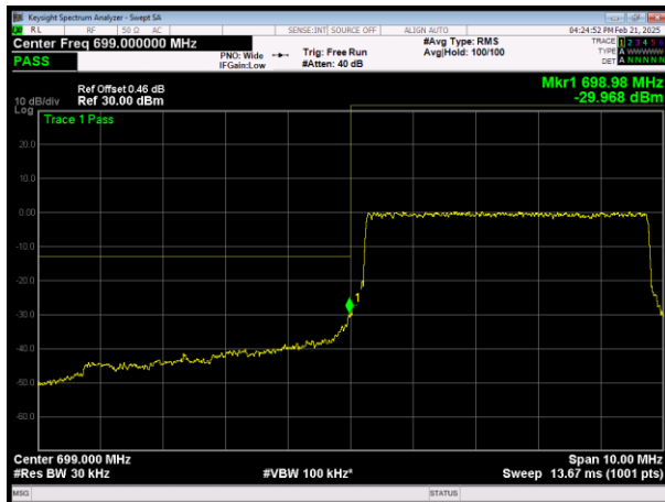
L\LTE Band12 QAM64 BW=5MHz Channel=23035 RB Size=25 Position=#0
