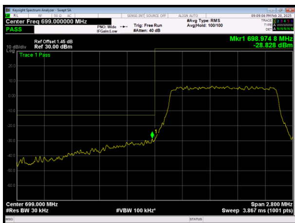
L/LTE Band12 QAM16 BW=1.4MHz Channel=23017 RB Size=6 Position=#0
