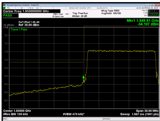
L\LTE Band25 QAM16 BW=15MHz Channel=26115 RB Size=75 Position=#0
