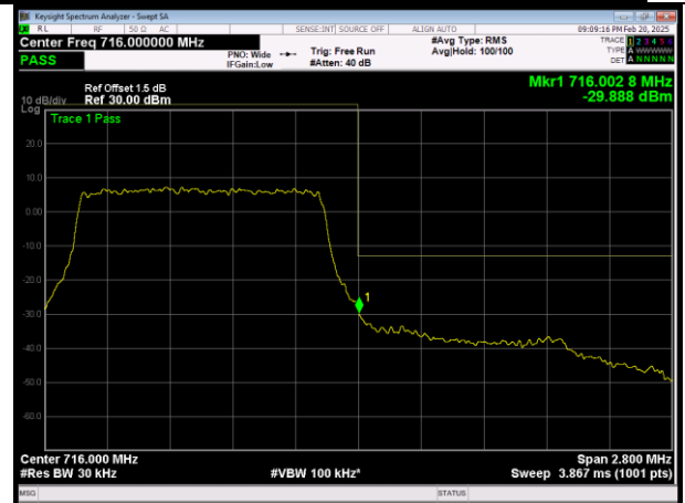
H\LTE Band12 QPSK BW=1.4MHz Channel=23173 RB Size=6 Position=#0
