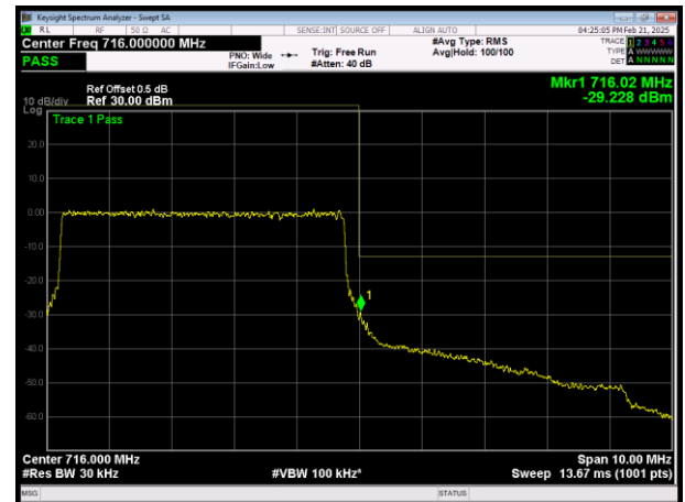
H\LTE Band12 QAM64 BW=5MHz Channel=23155 RB Size=25 Position=#0
