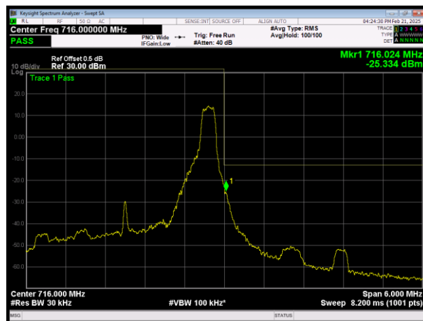
H\LTE Band12 QAM64 BW=3MHz Channel=23165 RB Size=1 Position=#Max
