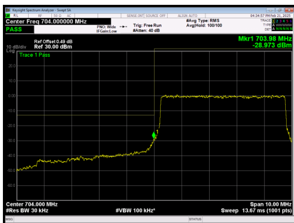
L\LTE Band17 QAM64 BW=5MHz Channel=23755 RB Size=25 Position=#0
