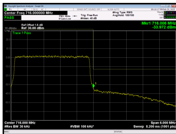
H\LTE Band12 QAM16 BW=3MHz Channel=23165 RB Size=15 Position=#0
