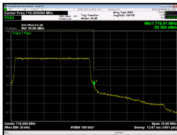
H\LTE Band17 QAM64 BW=5MHz Channel=23825 RB Size=25 Position=#0
