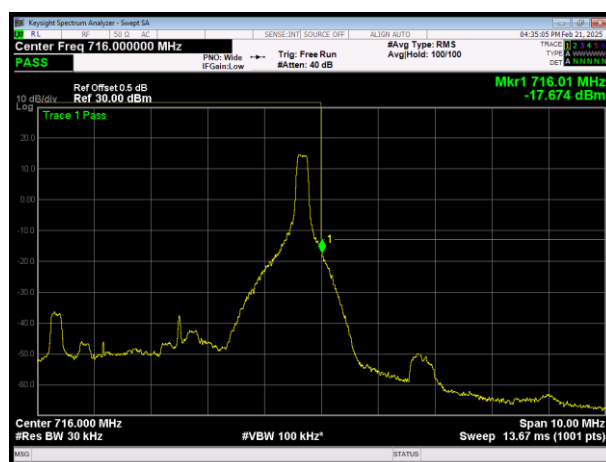
H\LTE Band17 QAM64 BW=5MHz Channel=23825 RB Size=1 Position=#Max
