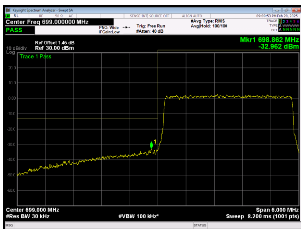
L\LTE Band12 QAM16 BW=3MHz Channel=23025 RB Size=15 Position=#0
