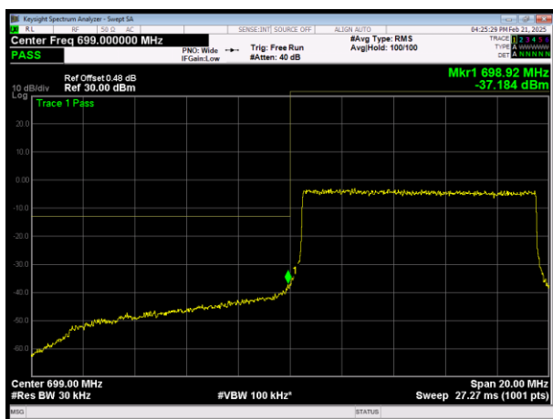
L\LTE Band12 QAM64 BW=10MHz Channel=23060 RB Size=50 Position=#0
