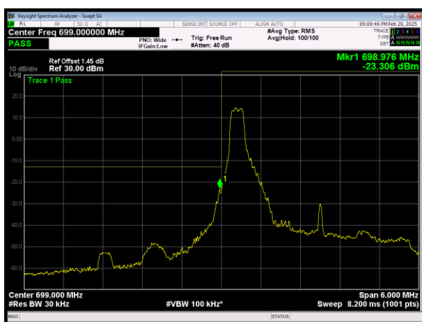
L\LTE Band12 QAM16 BW=3MHz Channel=23025 RB Size=1 Position=#0
