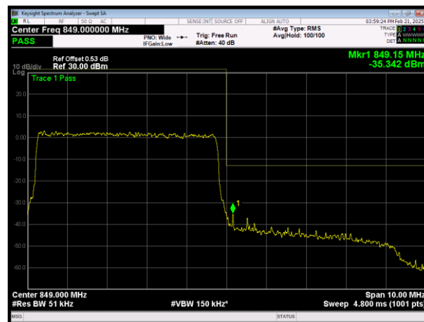
HLTE Band5 QAM64 BW=5MHz Channel=20625 RB Size=25 Position=#0
