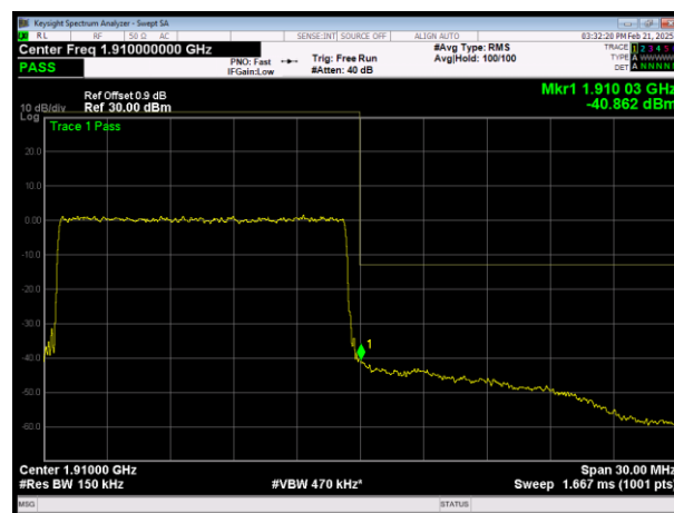
H\LTE Band2 QAM64 BW=15MHz Channel=19125 RB RB Size=75 Position=#0
