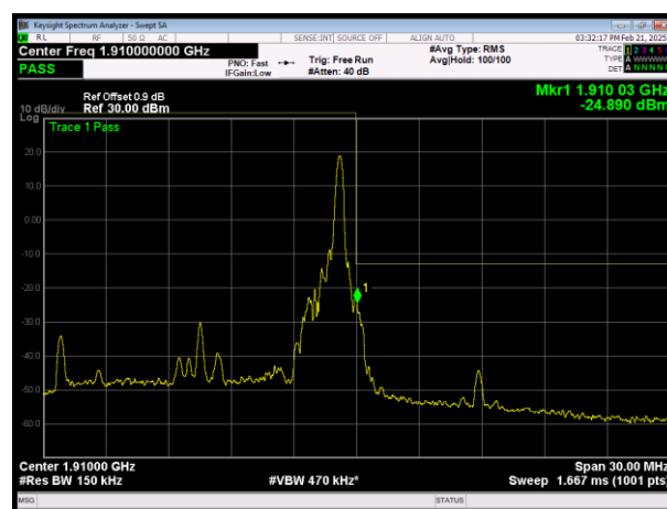
H\LTE Band2 QAM64 BW=15MHz Channel=19125 RB RB Size=1 Position=#Max
