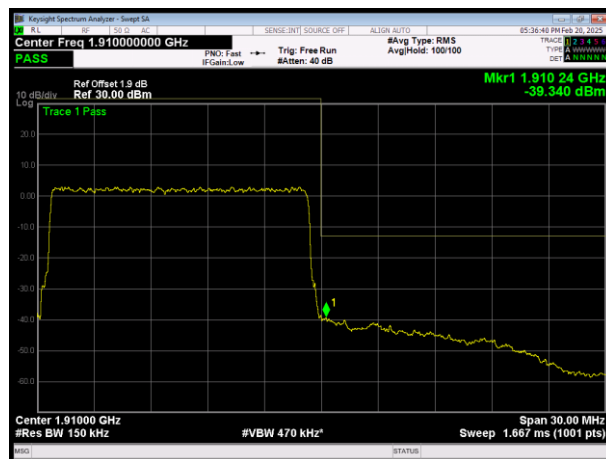
HLTE Band2 QPSK BW=15MHz Channel=19125 RB Size=75 Position=#0
