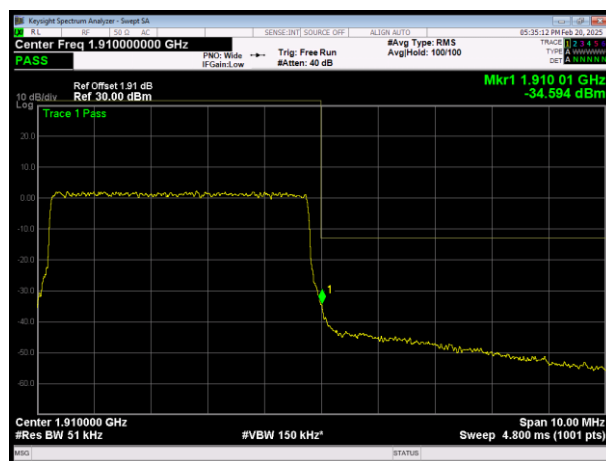
HLTE Band2 QAM16 BW=5MHz Channel=19175 RB Size=25 Position=#0
