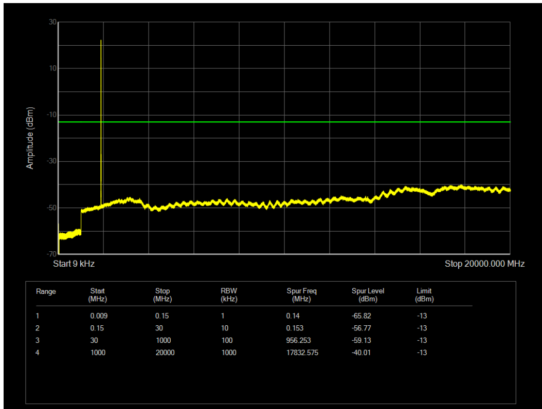
LTE Band25 QPSK BW=3MHz Channel=26365 RB Size=1 Position=#0
