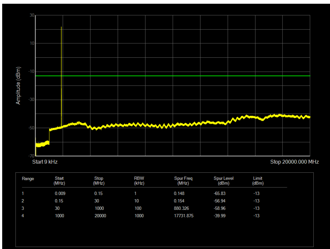
LTE Band2 QPSK BW=5MHz Channel=18900 RB Size=1 Position=#0
