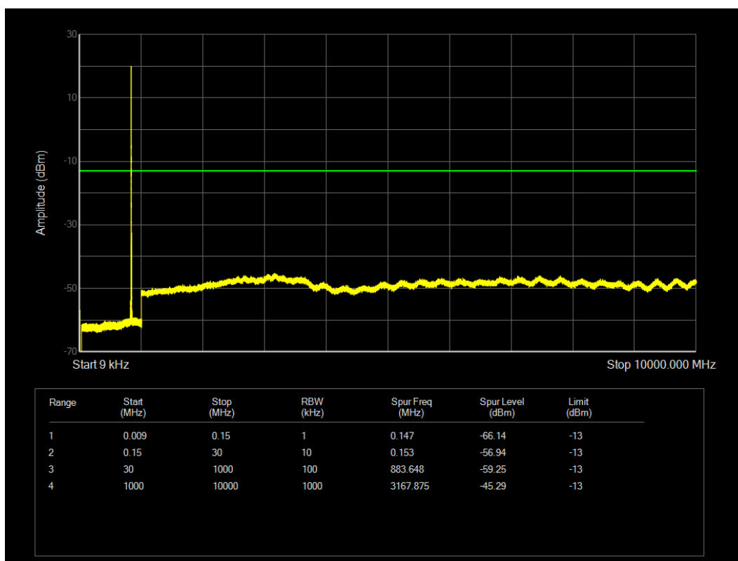
LTE Band5 QPSK BW=5MHz Channel=20525 RB Size=1 Position=#0
