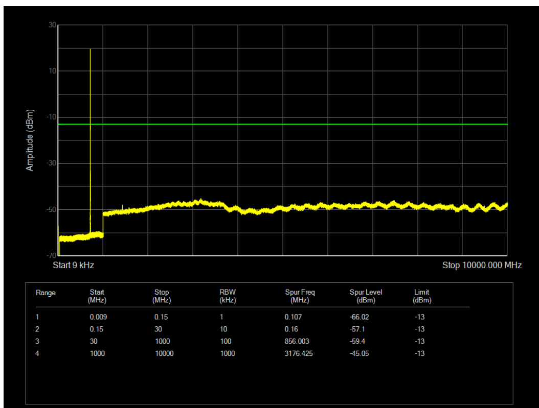
LTE Band12 QPSK BW=1.4MHz Channel=23173 RB Size=1 Position=#0
