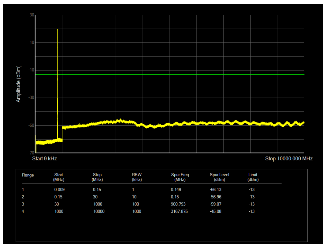
LTE Band26(814-824) QPSK BW=3MHz Channel=26775 RB Size=1 Position=#0
