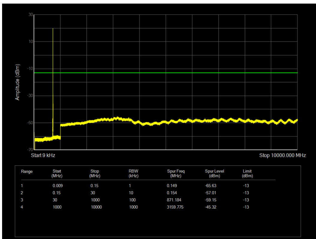
LTE Band12 QPSK BW=3MHz Channel=23165 RB Size=1 Position=#0
