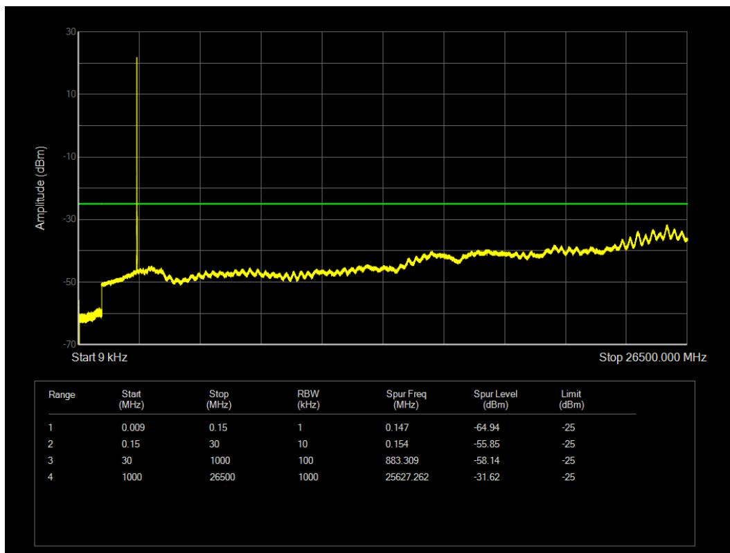
LTE Band7 QPSK BW=10MHz Channel=21100 RB Size=1 Position=#0
