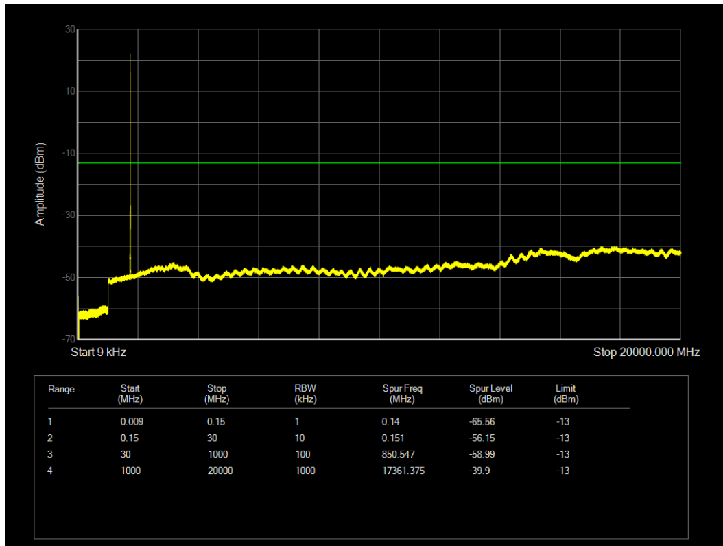
LTE Band4 QPSK BW=3MHz Channel=20175 RB Size=1 Position=#0
