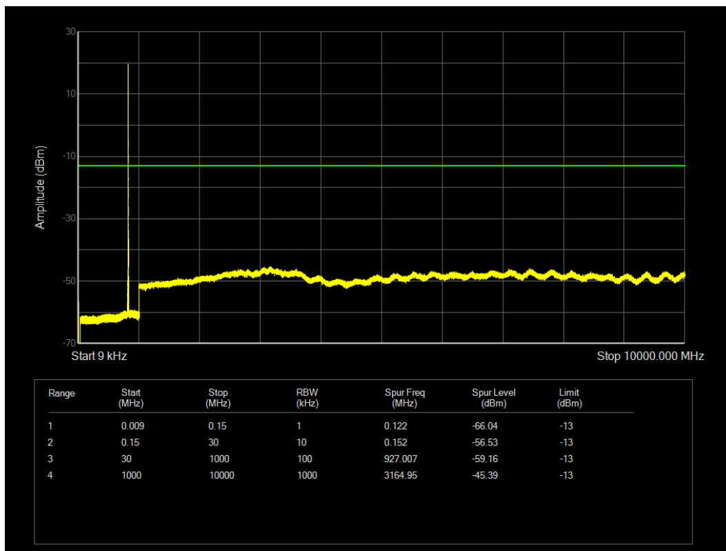
LTE Band26(814-824) QPSK BW=5MHz Channel=26765 RB Size=1 Position=#0
