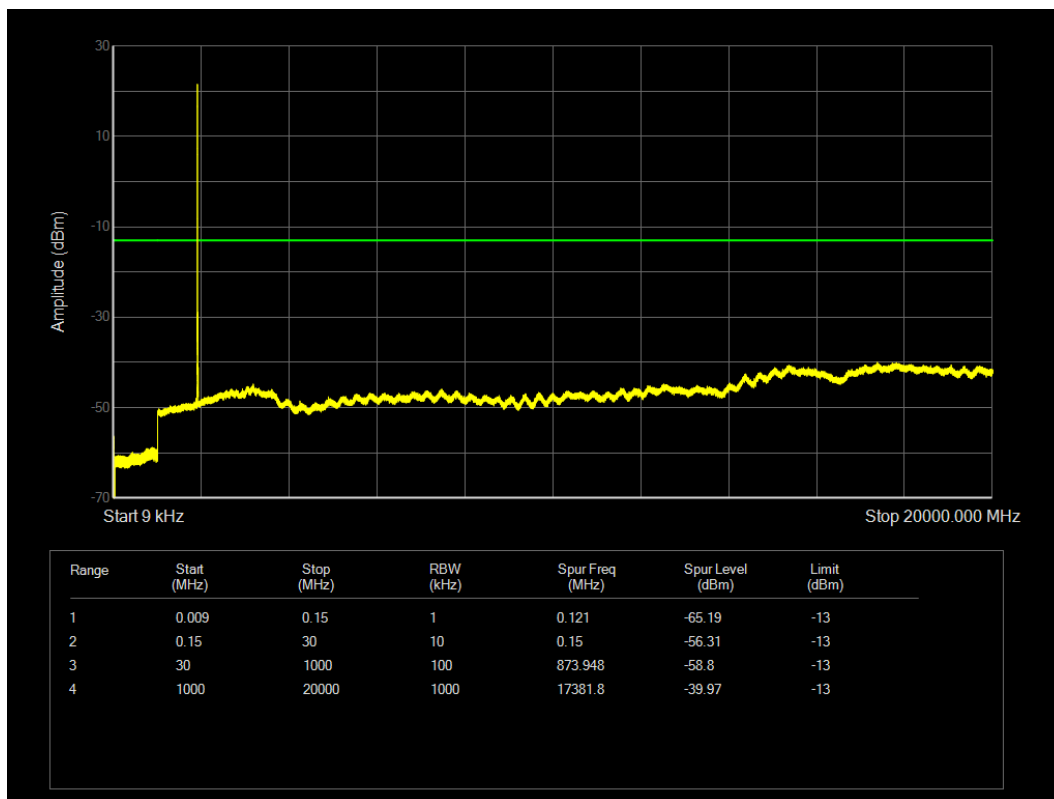
LTE Band25 QPSK BW=10MHz Channel=26640 RB Size=1 Position=#0
