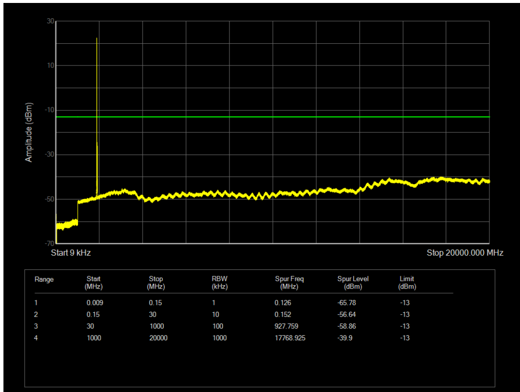
LTE Band25 QPSK BW=15MHz Channel=26365 RB Size=1 Position=#0
