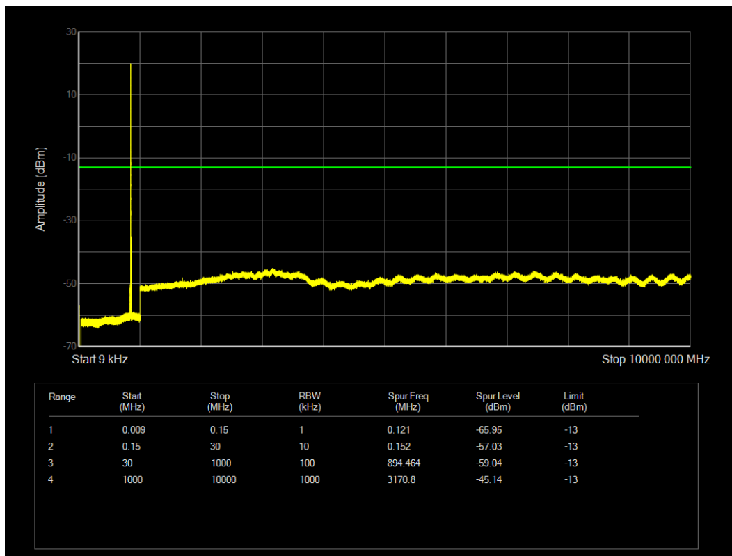
LTE Band5 QPSK BW=5MHz Channel=20625 RB Size=1 Position=#0
