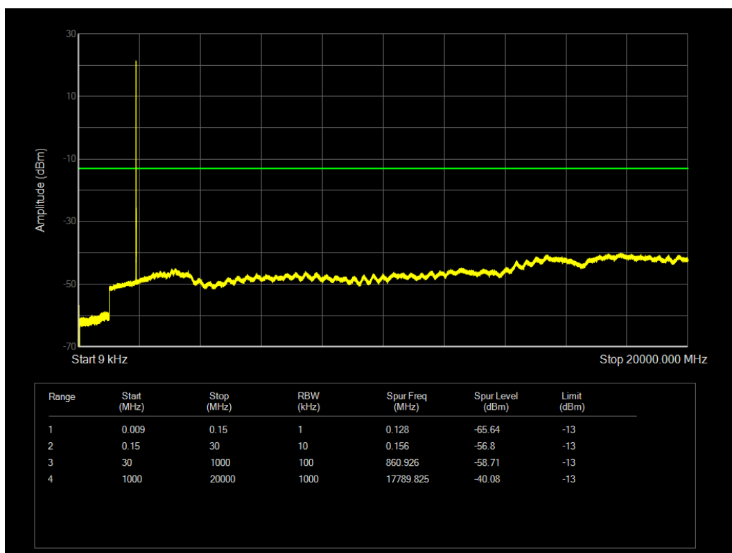
LTE Band25 QPSK BW=5MHz Channel=26365 RB Size=1 Position=#0
