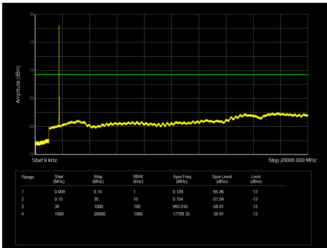
LTE Band4 QPSK BW=10MHz Channel=20350 RB Size=1 Position=#0
