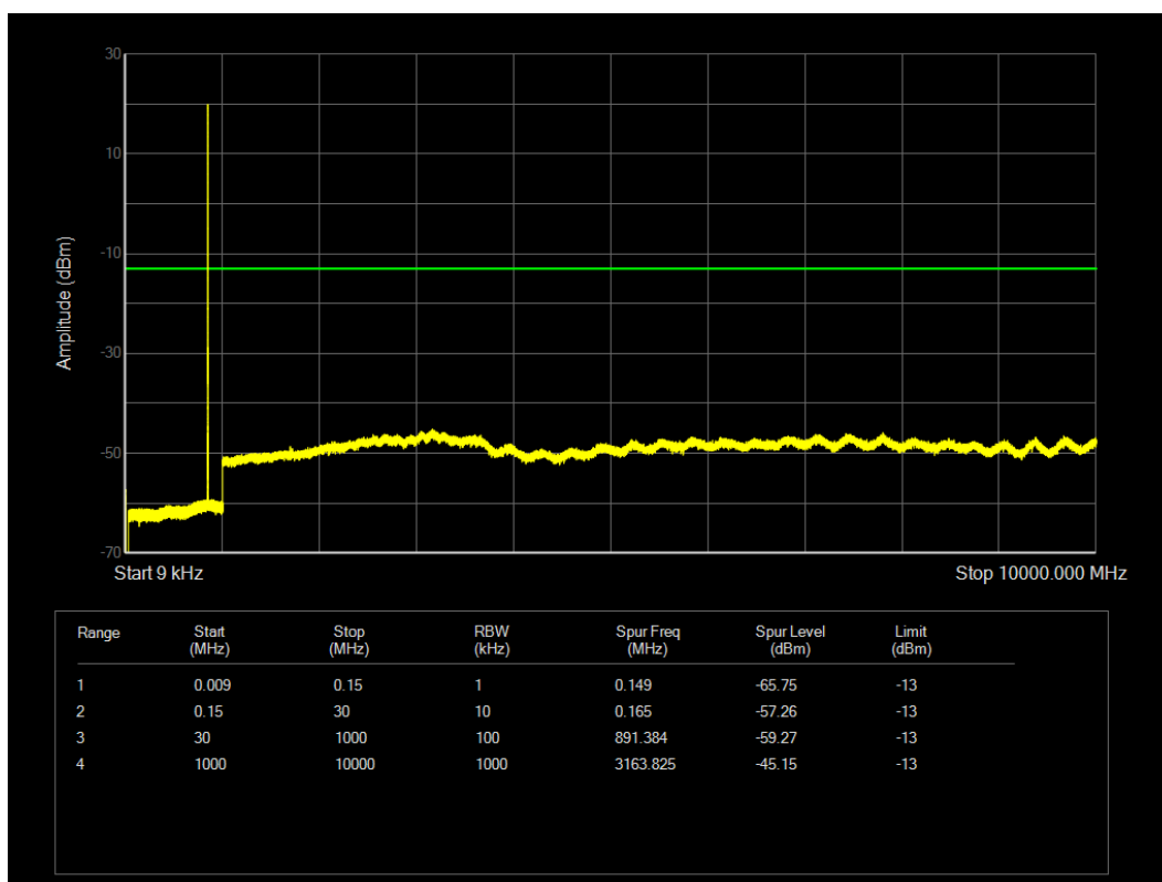
LTE Band26(824-849) QPSK BW=1.4MHz Channel=27033 RB Size=1 Position=#0
