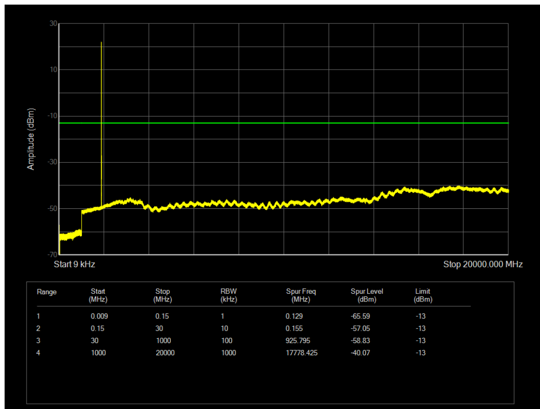
LTE Band2 QPSK BW=3MHz Channel=18900 RB Size=1 Position=#0
