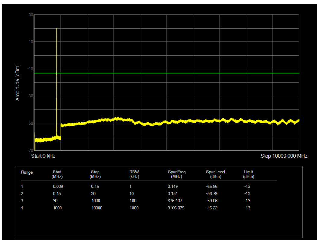
LTE Band5 QPSK BW=3MHz Channel=20635 RB Size=1 Position=#0
