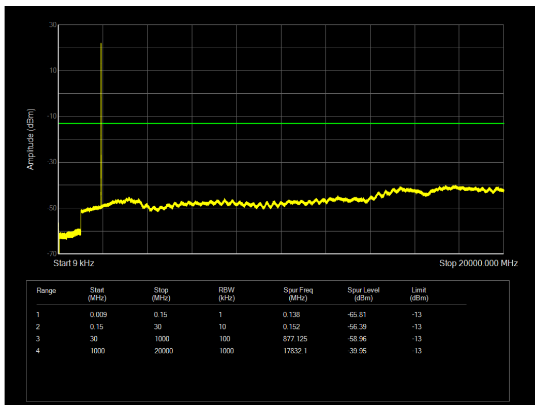
LTE Band2 QPSK BW=3MHz Channel=19185 RB Size=1 Position=#0
