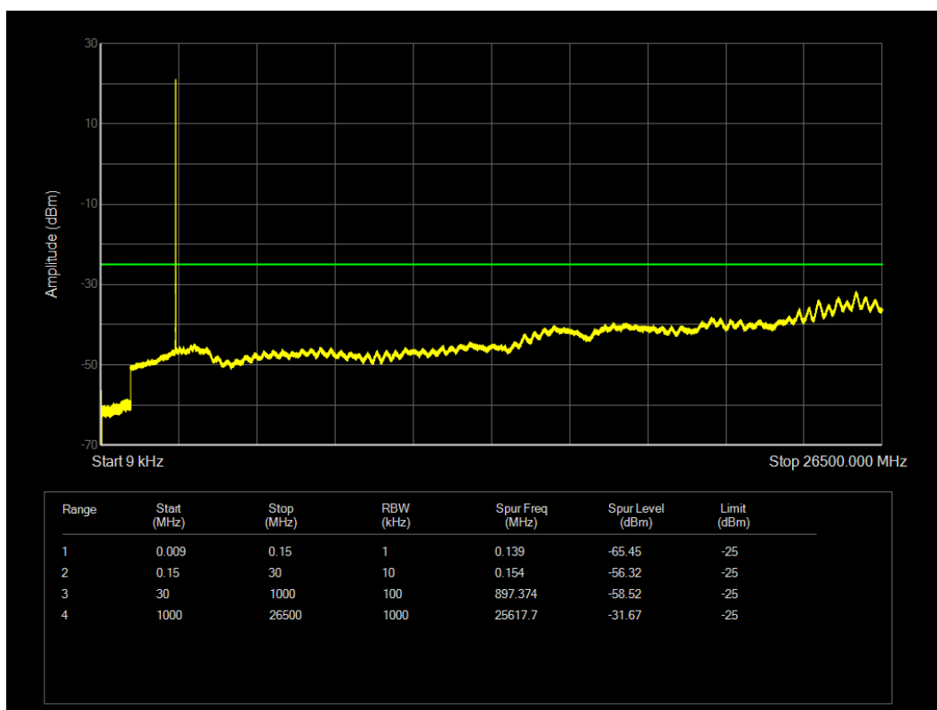
LTE Band7 QPSK BW=5MHz Channel=21100 RB Size=1 Position=#0
