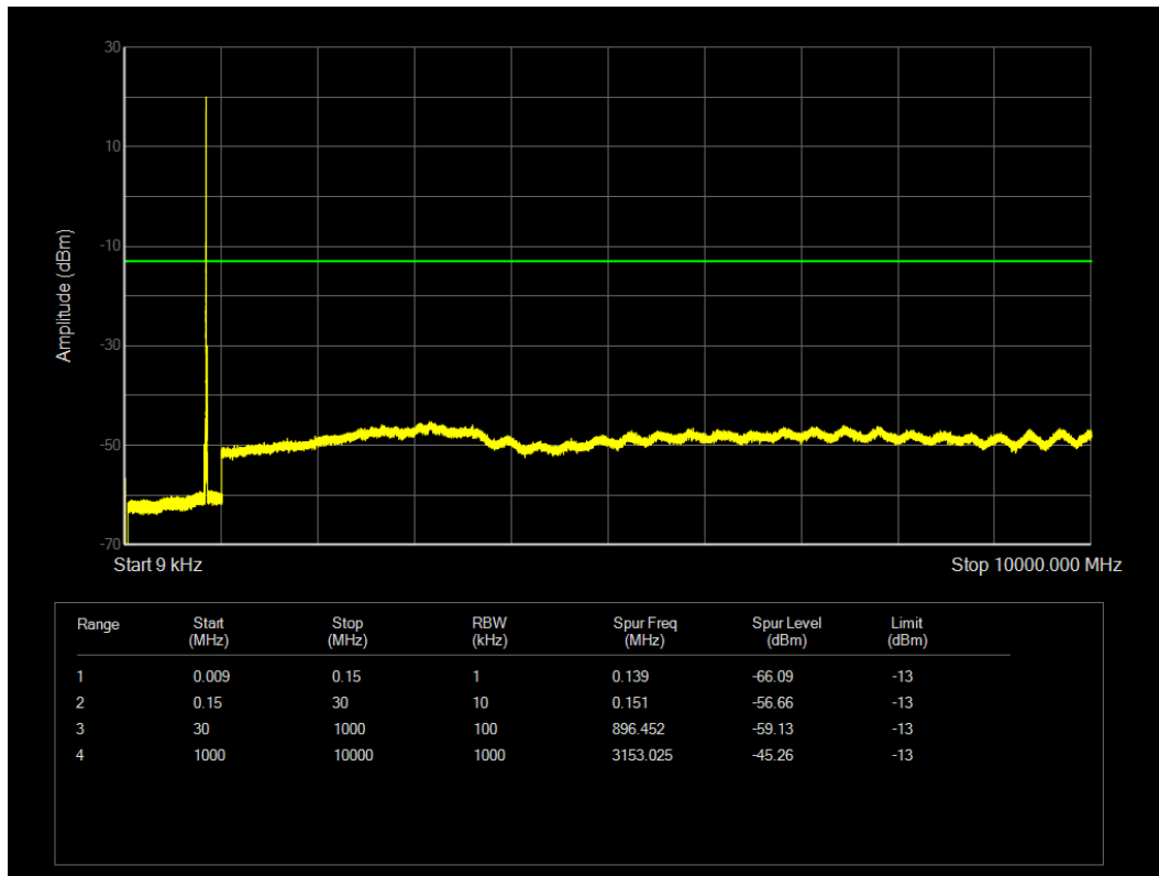
LTE Band5 QPSK BW=10MHz Channel=20600 RB Size=1 Position=#0
