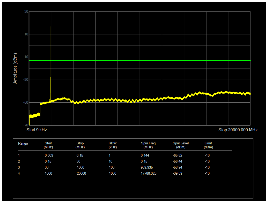
LTE Band25 QPSK BW=20MHz Channel=26590 RB Size=1 Position=#0
