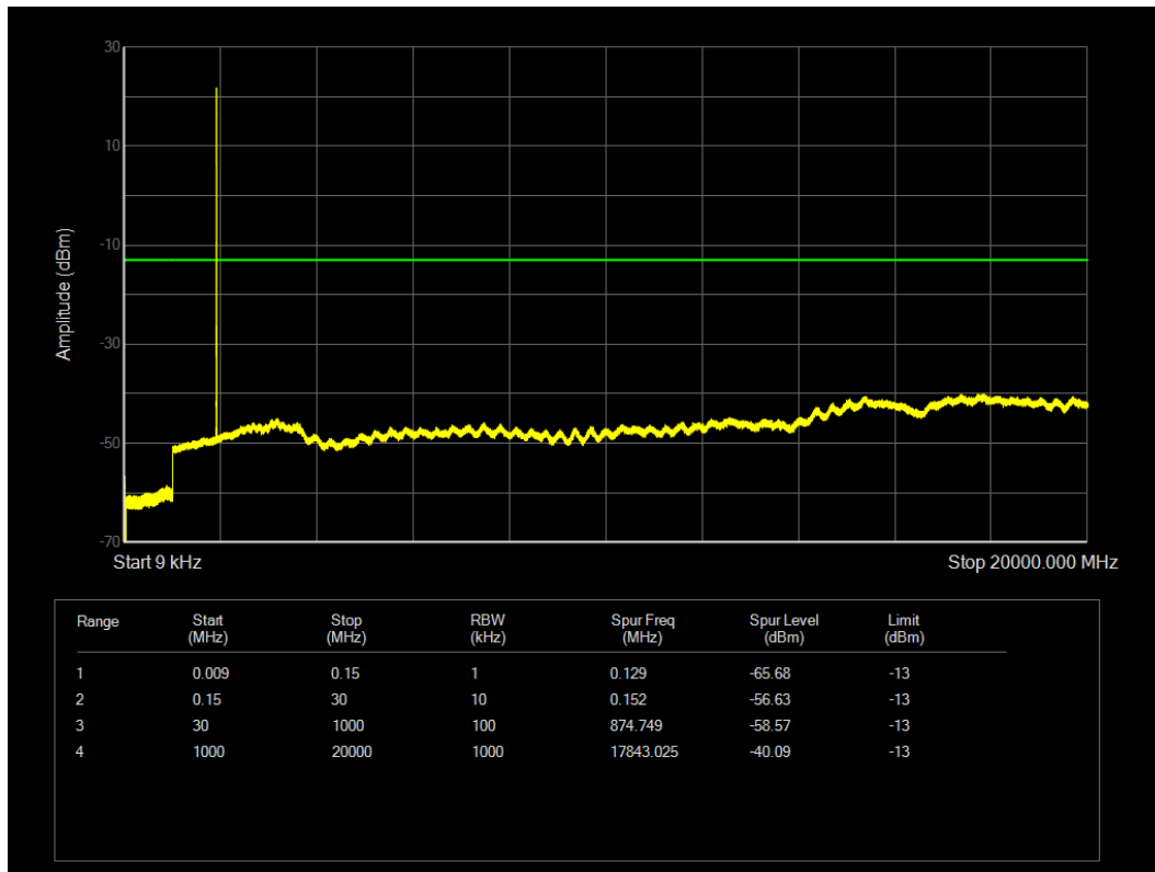
LTE Band25 QPSK BW=5MHz Channel=26665 RB Size=1 Position=#0
