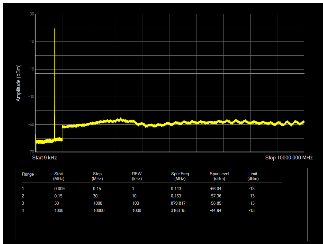
LTE Band12 QPSK BW=5MHz Channel=23155 RB Size=1 Position=#0
