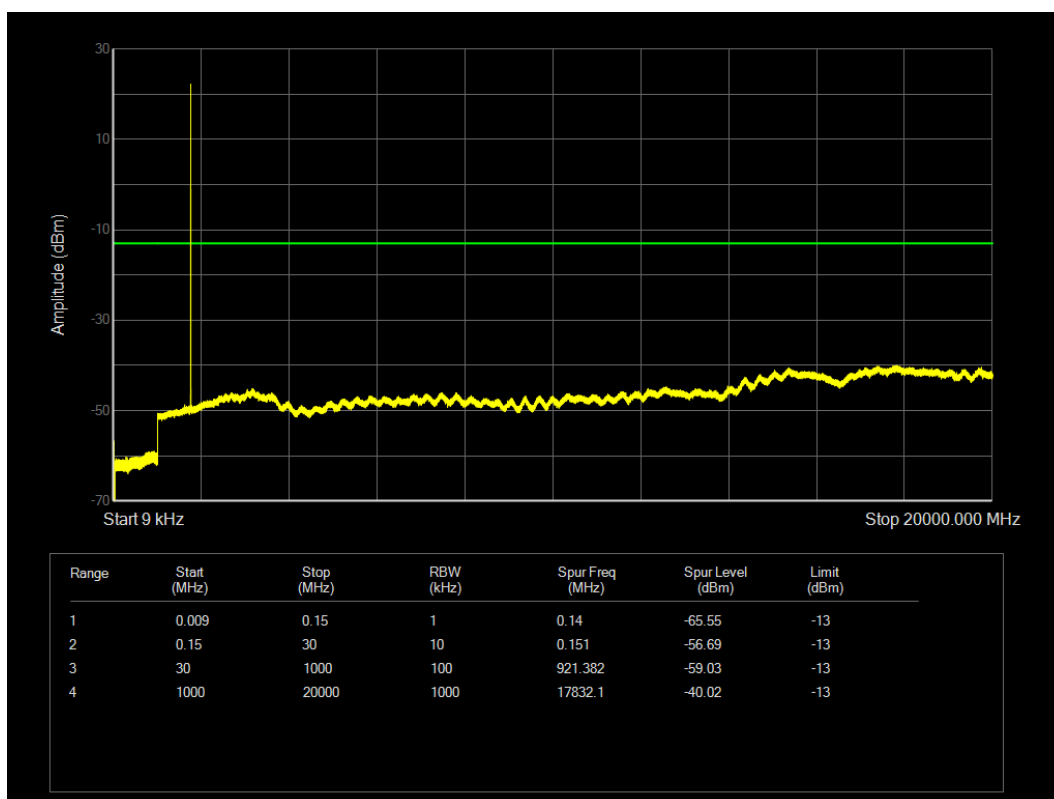
LTE Band4 QPSK BW=1.4MHz Channel=20393 RB Size=1 Position=#0
