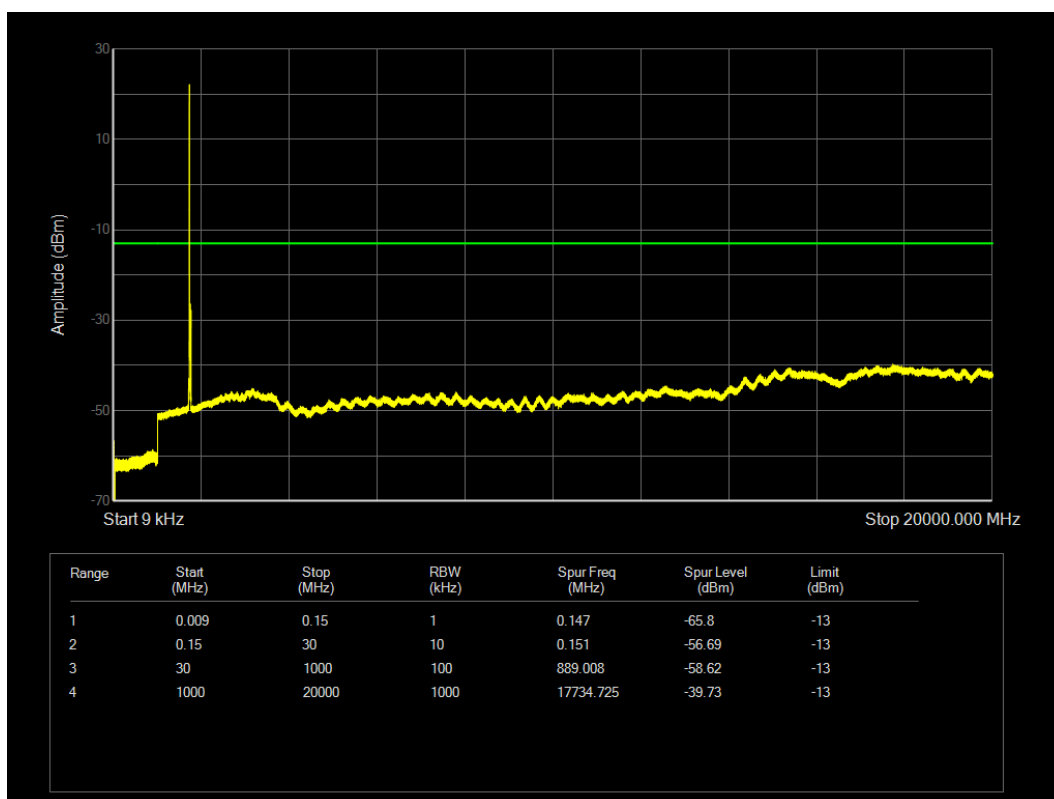
LTE Band4 QPSK BW=20MHz Channel=20175 RB Size=1 Position=#0
