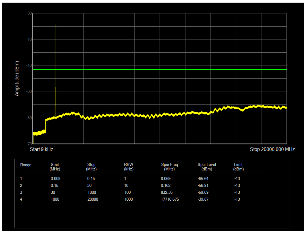
LTE Band4 QPSK BW=5MHz Channel=20375 RB Size=1 Position=#0
