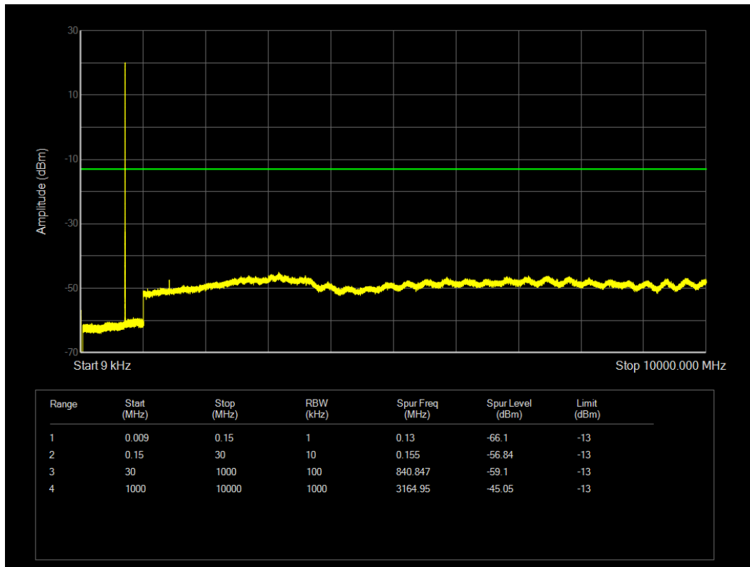
LTE Band12 QPSK BW=1.4MHz Channel=23095 RB Size=1 Position=#0
