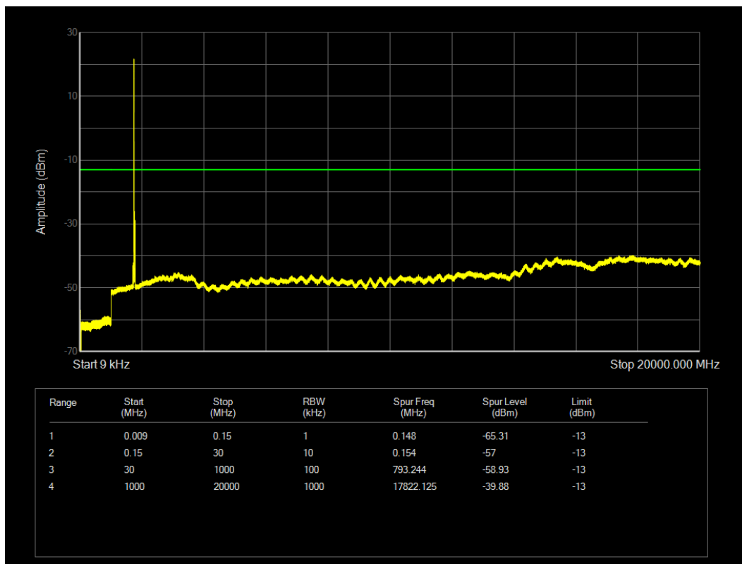
LTE Band4 QPSK BW=20MHz Channel=20300 RB Size=1 Position=#0
