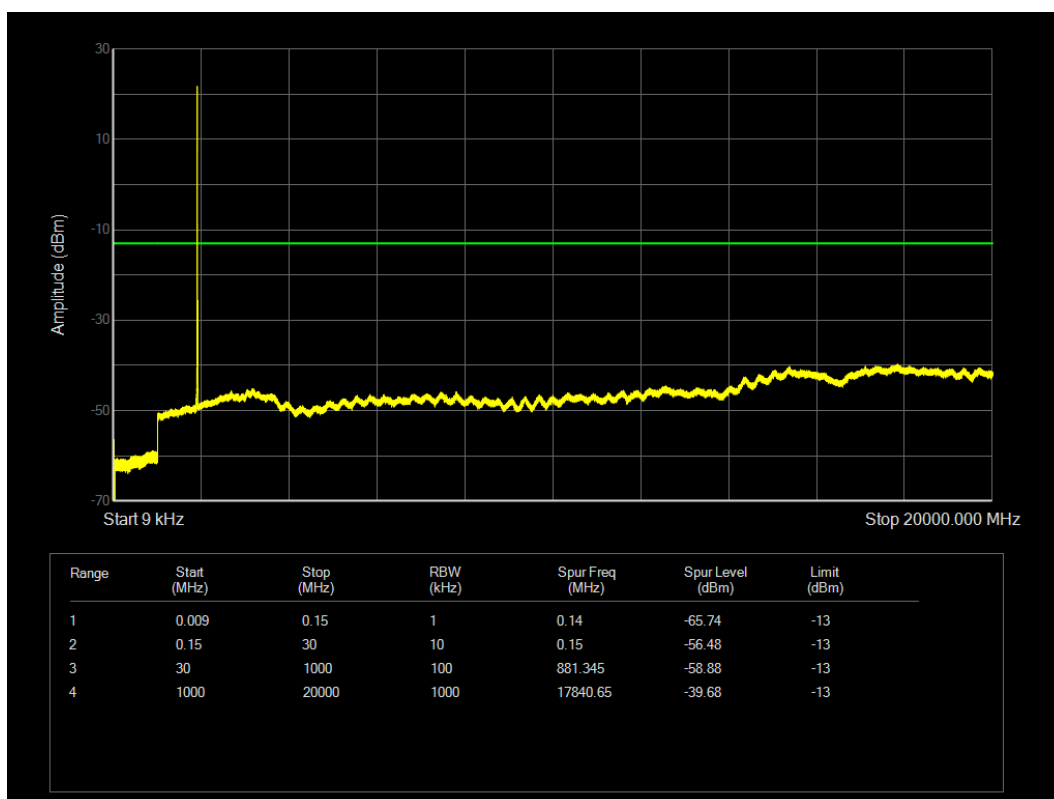
LTE Band25 QPSK BW=15MHz Channel=26615 RB Size=1 Position=#0
