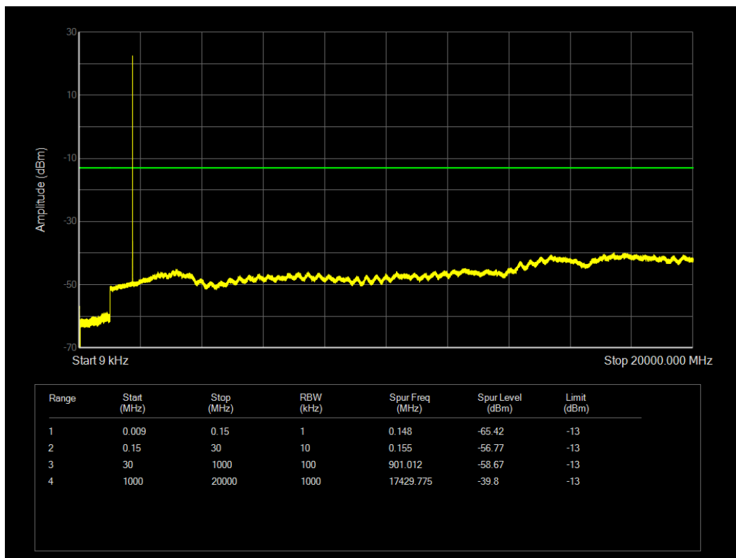
LTE Band4 QPSK BW=1.4MHz Channel=20175 RB Size=1 Position=#0
