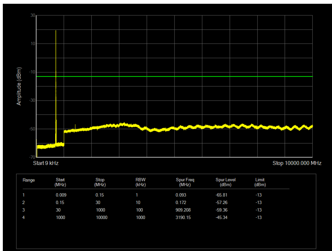
LTE Band12 QPSK BW=10MHz Channel=23095 RB Size=1 Position=#0
