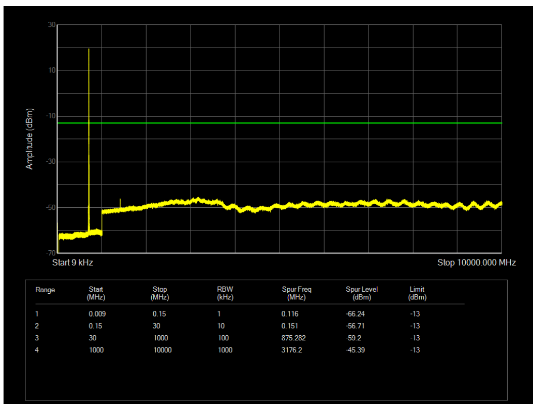
LTE Band12 QPSK BW=5MHz Channel=23095 RB Size=1 Position=#0
