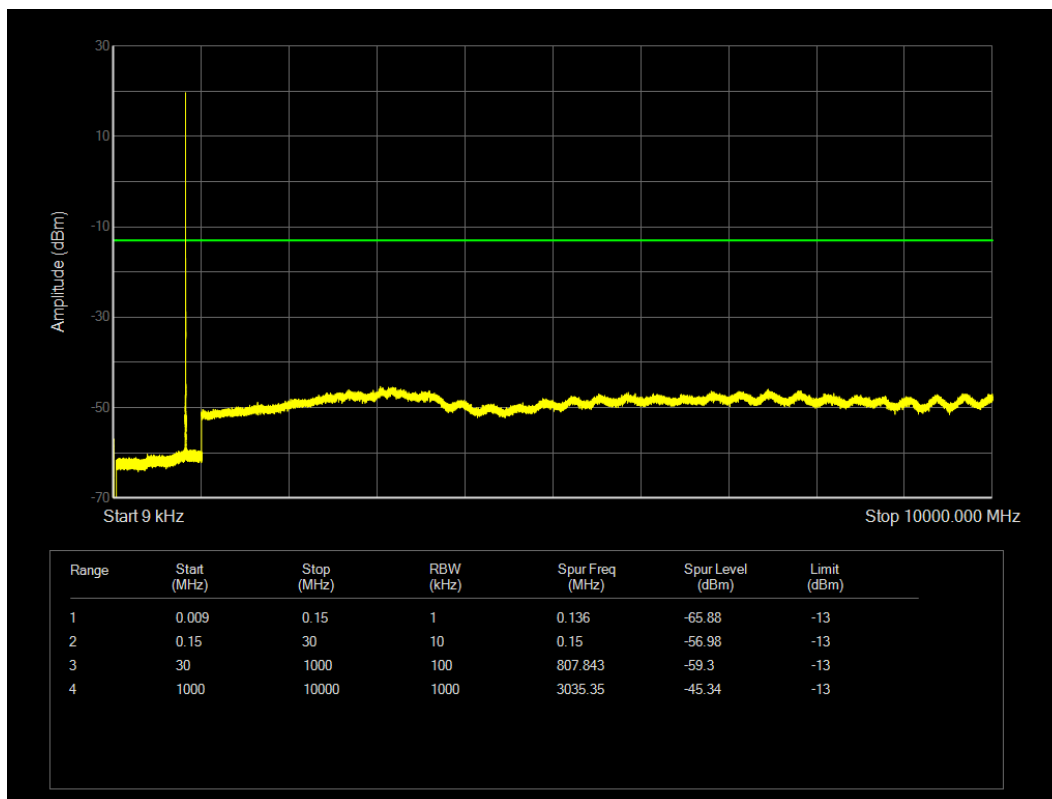
LTE Band26(814-824) QPSK BW=1.4MHz Channel=26740 RB Size=1 Position=#0
