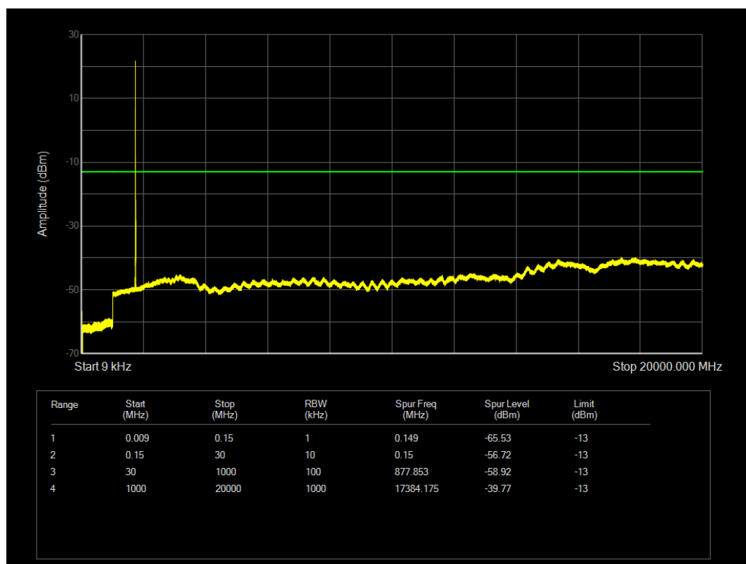
LTE Band4 QPSK BW=5MHz Channel=20175 RB Size=1 Position=#0
