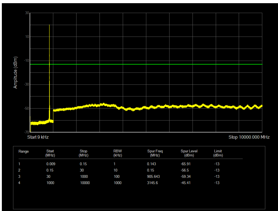
LTE Band26(824-849) QPSK BW=10MHz Channel=26915 RB Size=1 Position=#0
