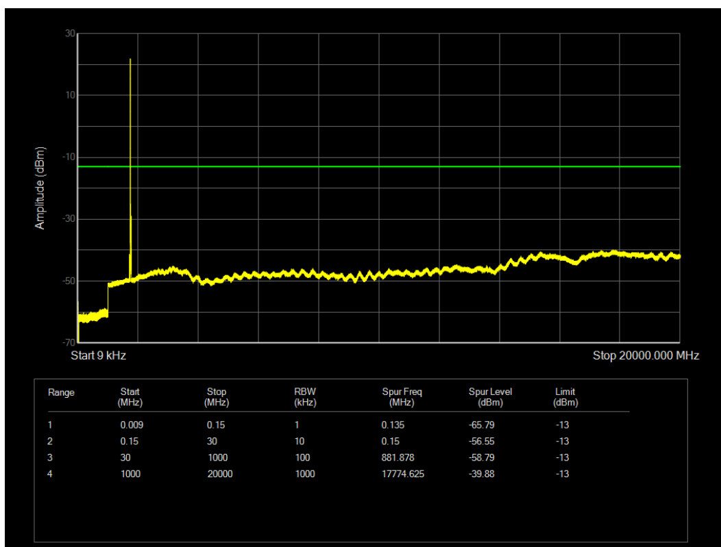
LTE Band4 QPSK BW=15MHz Channel=20325 RB Size=1 Position=#0
