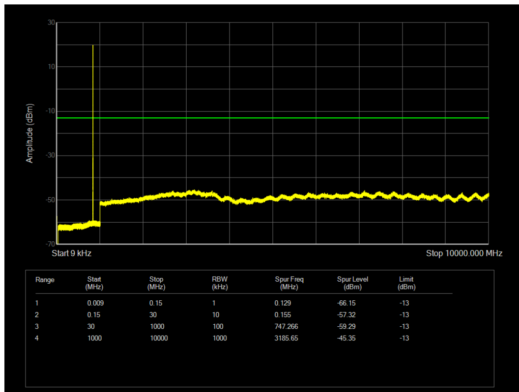
LTE Band5 QPSK BW=1.4MHz Channel=20525 RB Size=1 Position=#0
