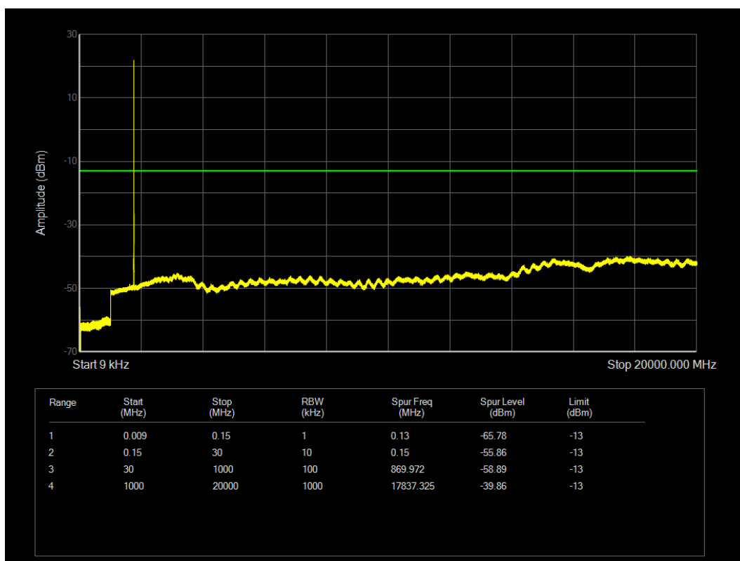
LTE Band4 QPSK BW=3MHz Channel=20385 RB Size=1 Position=#0
