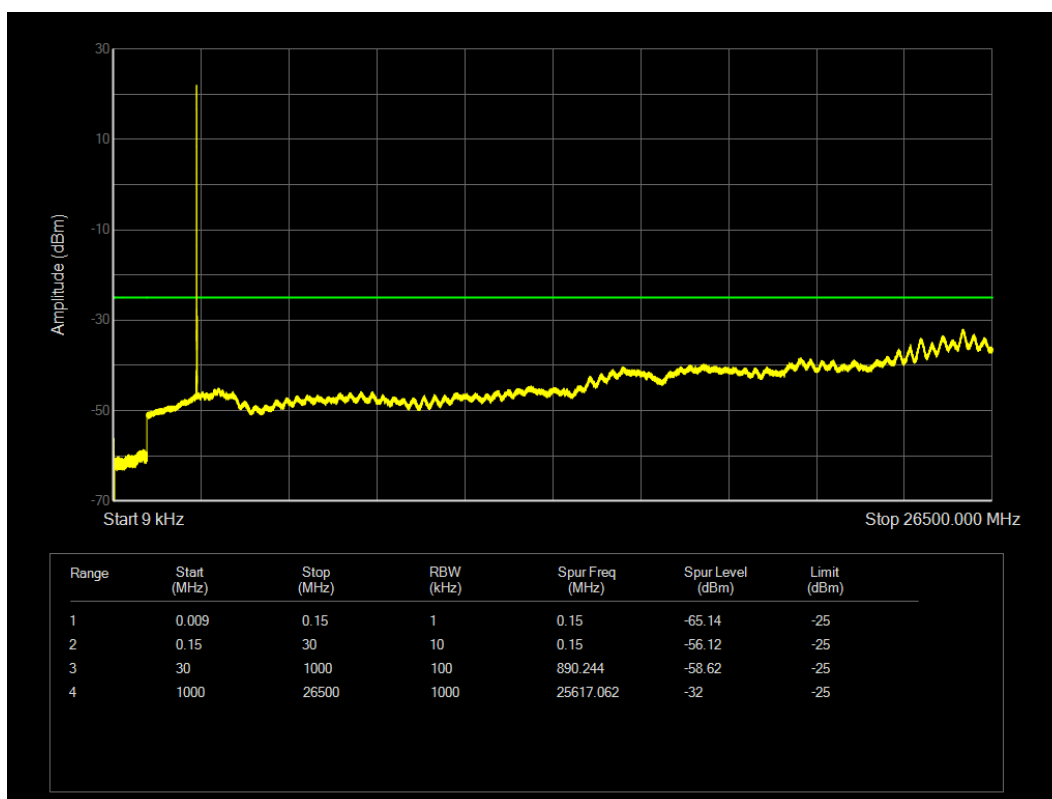
LTE Band7 QPSK BW=10MHz Channel=20800 RB Size=1 Position=#0
