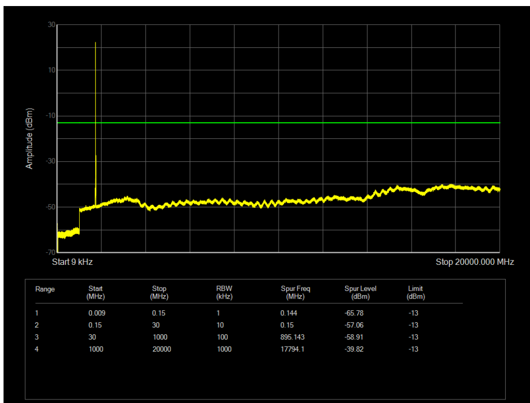
LTE Band4 QPSK BW=10MHz Channel=20175 RB Size=1 Position=#0
