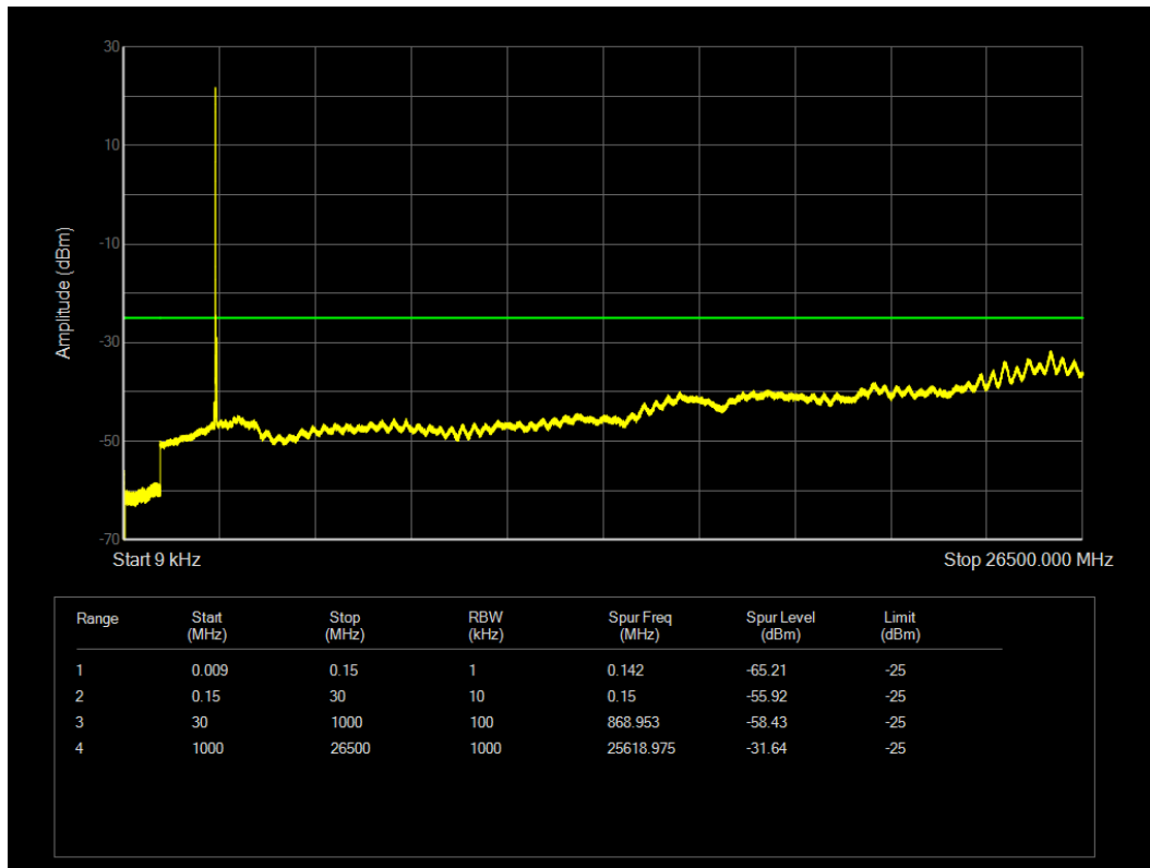
LTE Band7 QPSK BW=20MHz Channel=21100 RB Size=1 Position=#0
