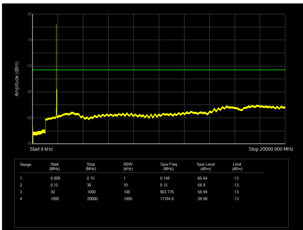
LTE Band25 QPSK BW=20MHz Channel=26365 RB Size=1 Position=#0
