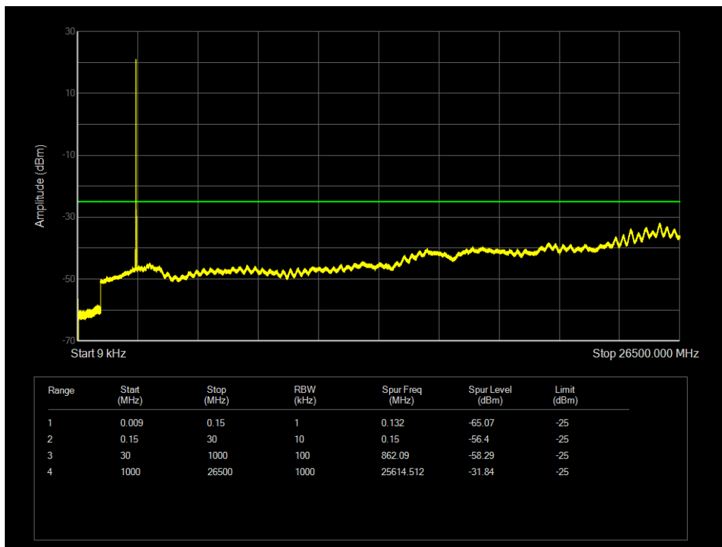
LTE Band7 QPSK BW=15MHz Channel=21375 RB Size=1 Position=#0
