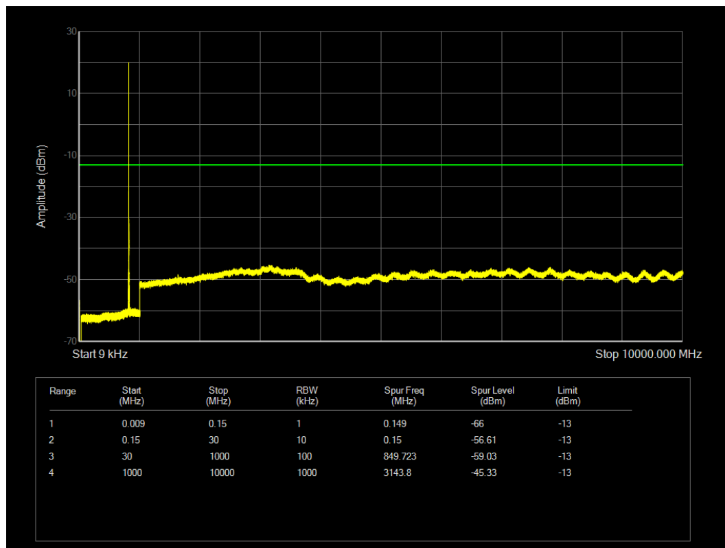
LTE Band26(814-824) QPSK BW=3MHz Channel=26740 RB Size=1 Position=#0
