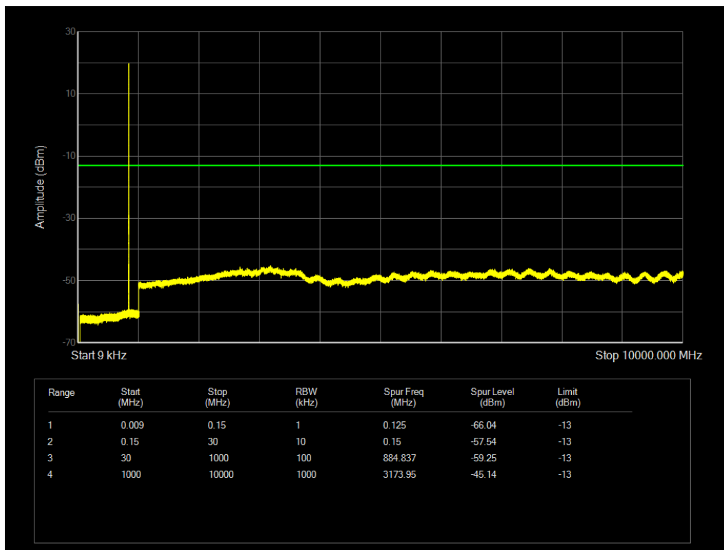
LTE Band26(824-849) QPSK BW=1.4MHz Channel=26915 RB Size=1 Position=#0
