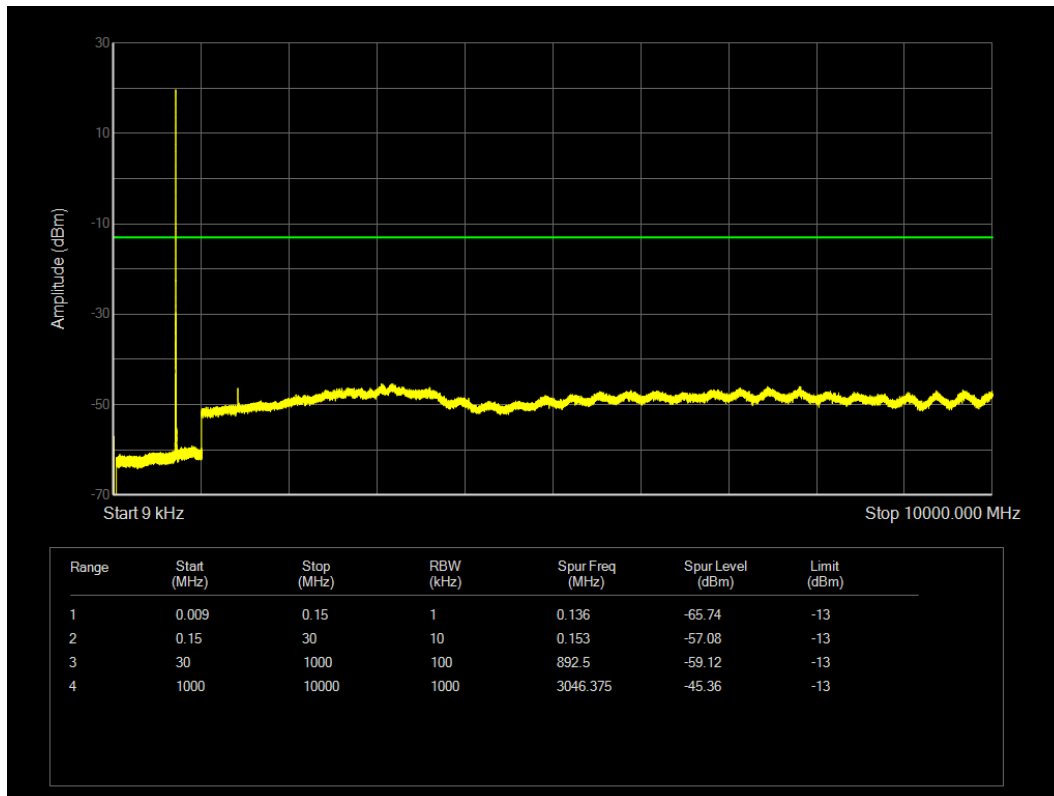
LTE Band12 QPSK BW=3MHz Channel=23095 RB Size=1 Position=#0
