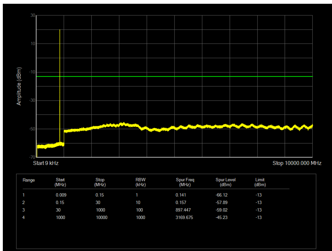
LTE Band5 QPSK BW=1.4MHz Channel=20643 RB Size=1 Position=#0
