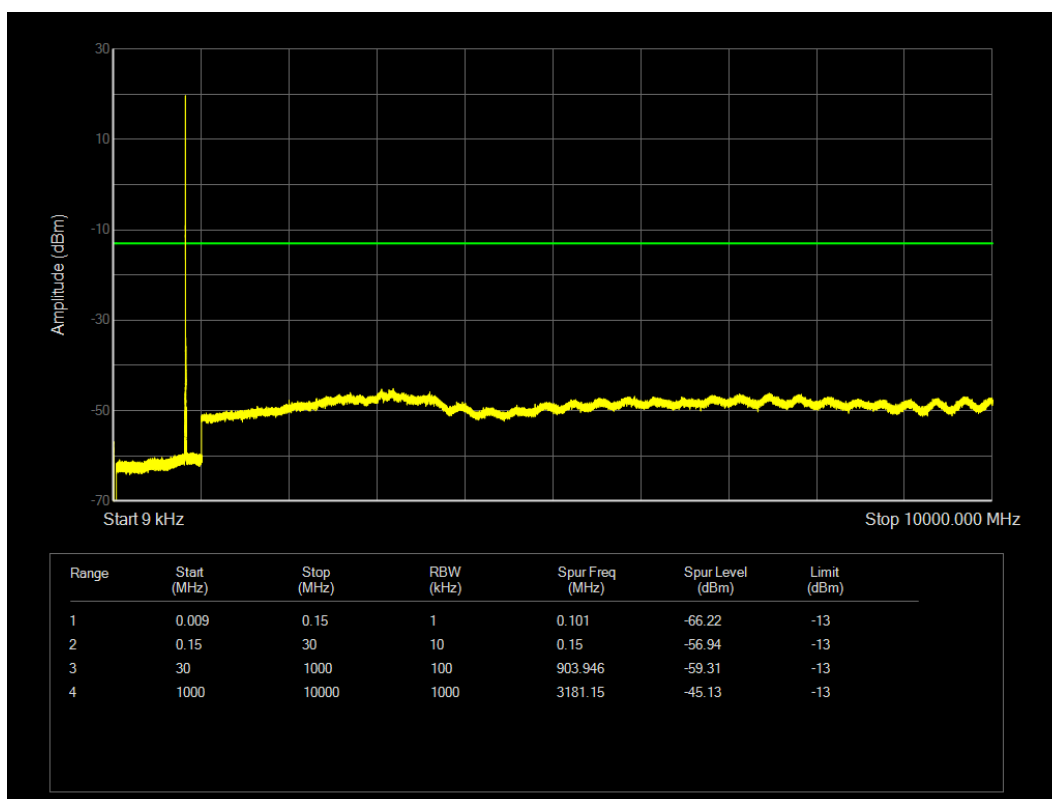
LTE Band26(814-824) QPSK BW=5MHz Channel=26740 RB Size=1 Position=#0
