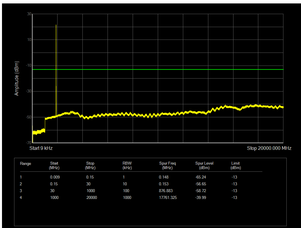
LTE Band25 QPSK BW=10MHz Channel=26365 RB Size=1 Position=#0
