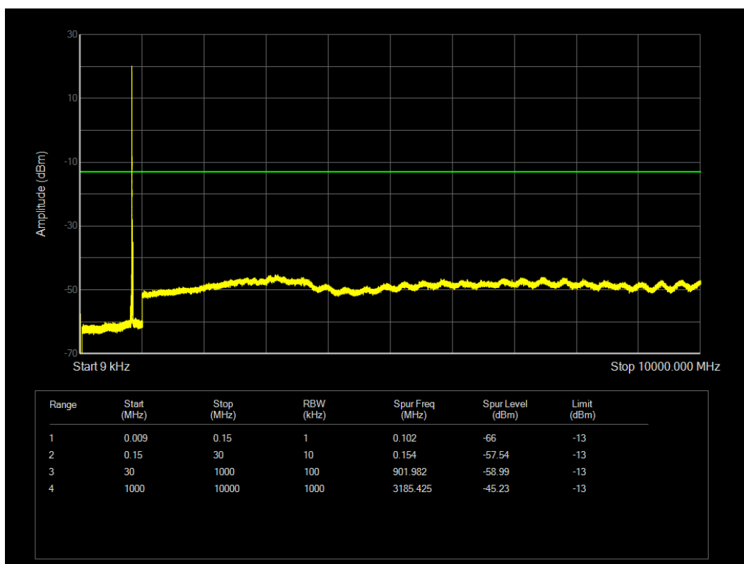
LTE Band5 QPSK BW=10MHz Channel=20525 RB Size=1 Position=#0
