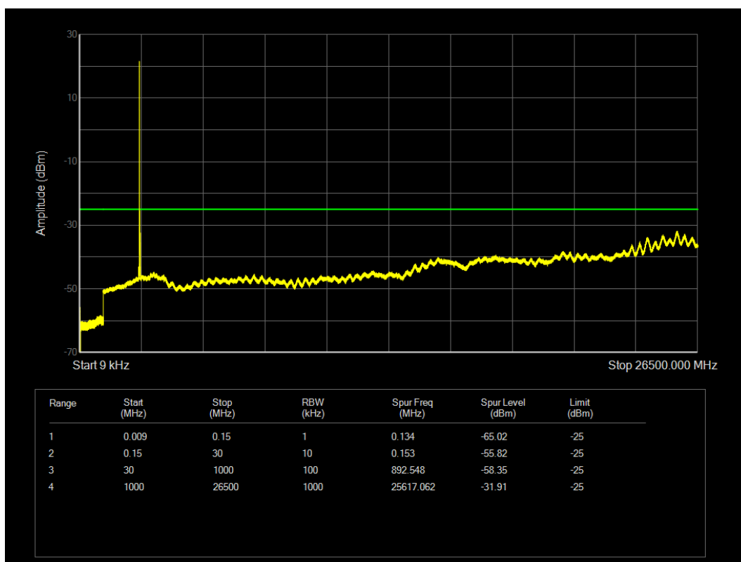
LTE Band7 QPSK BW=20MHz Channel=21350 RB Size=1 Position=#0
