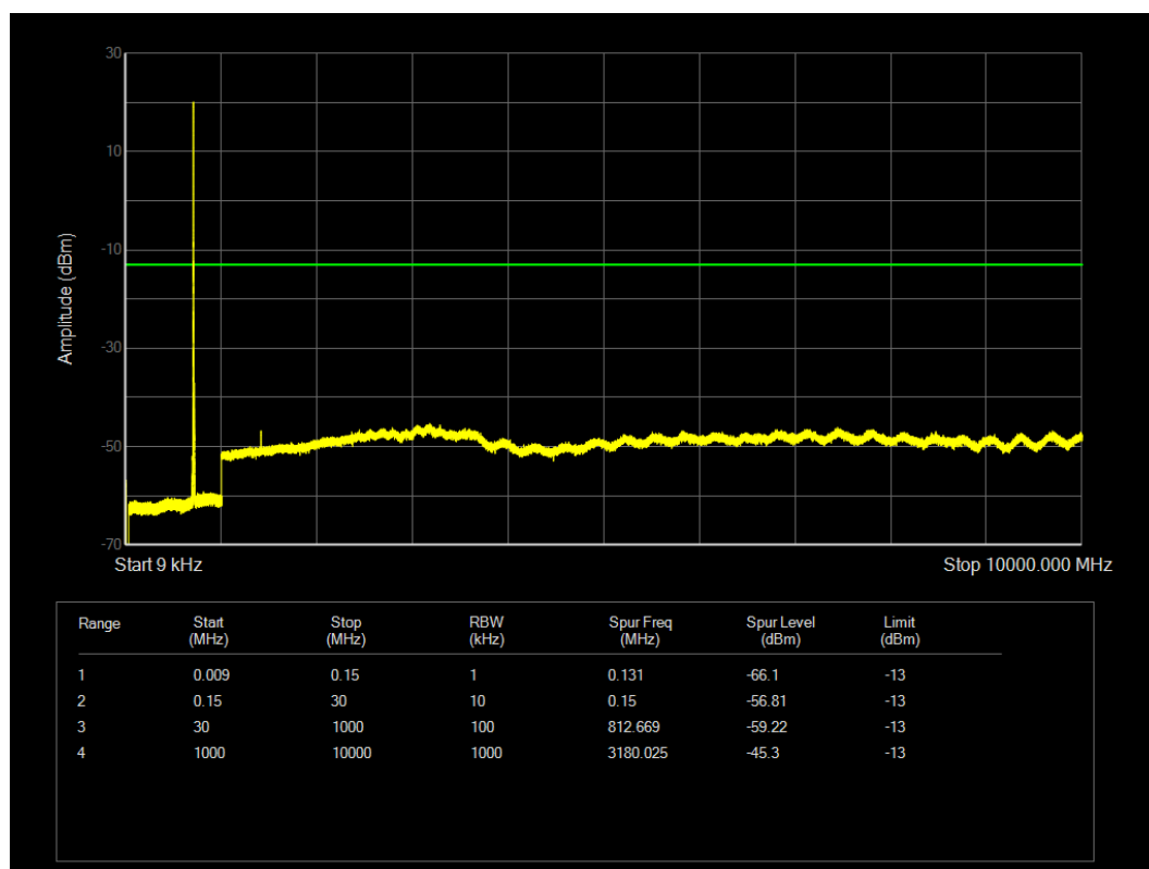
LTE Band17 QPSK BW=10MHz Channel=23800 RB Size=1 Position=#0
