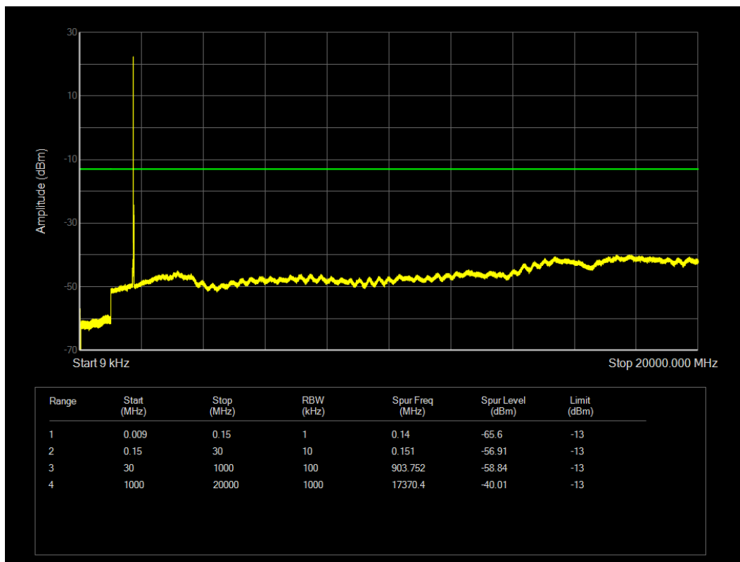
LTE Band4 QPSK BW=15MHz Channel=20175 RB Size=1 Position=#0
