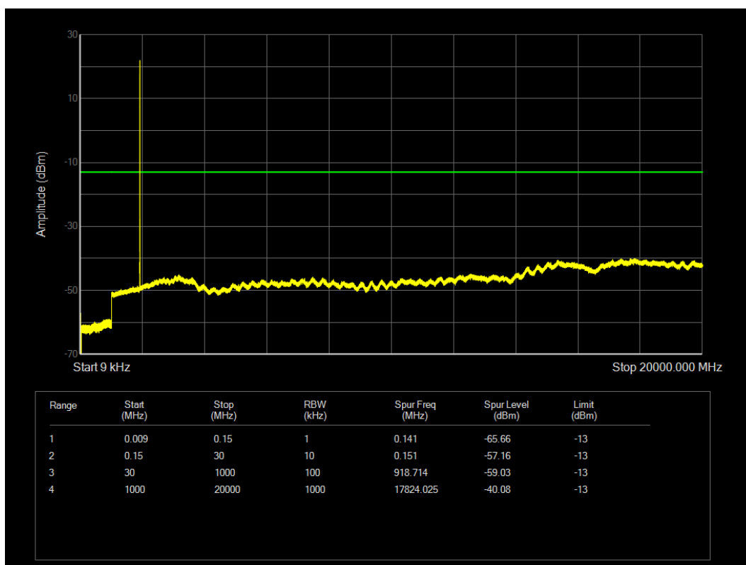
LTE Band25 QPSK BW=3MHz Channel=26675 RB Size=1 Position=#0
