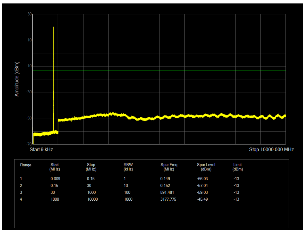
LTE Band26(814-824) QPSK BW=1.4MHz Channel=26783 RB Size=1 Position=#0
