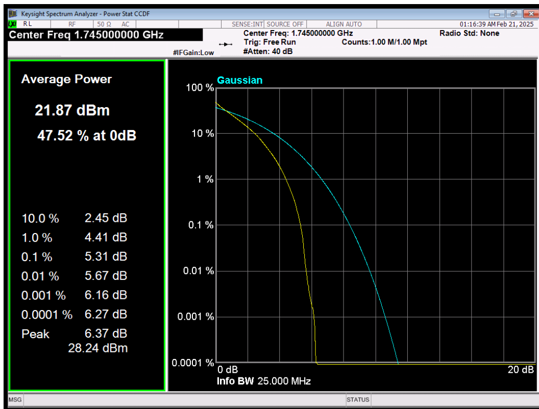
LTE Band66 QPSK BW=15MHz Channel=132322 RB Size=75 Position=#0
