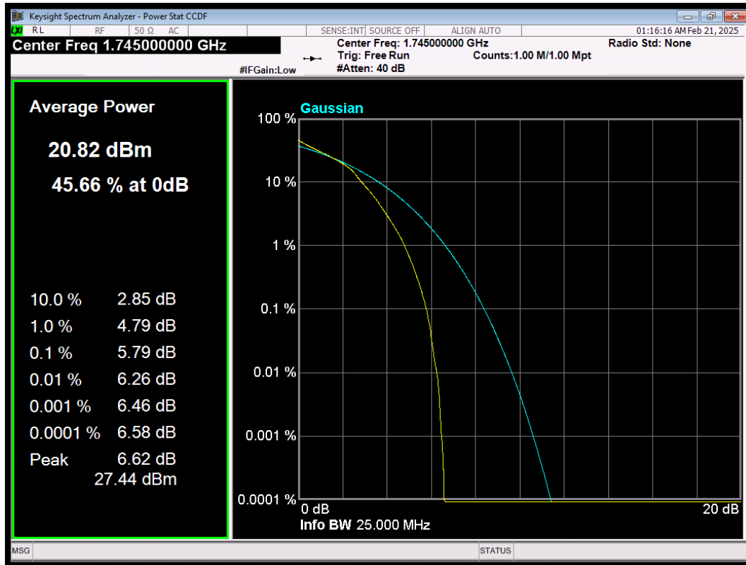
LTE Band66 QAM16 BW=10MHz Channel=132322 RB Size=50 Position=#0
