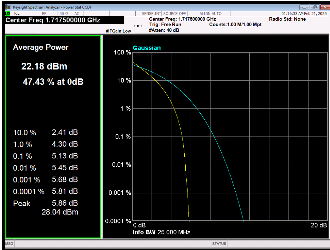
LTE Band66 QPSK BW=15MHz Channel=132047 RB Size=75 Position=#0
