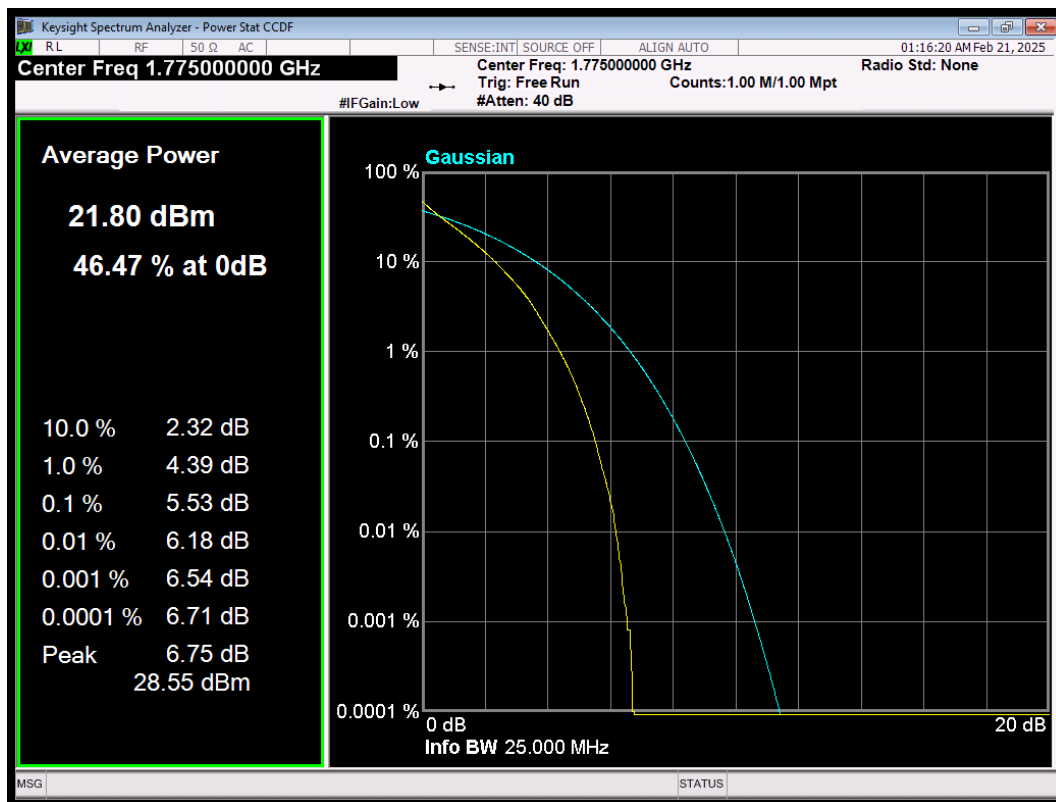
LTE Band66 QPSK BW=10MHz Channel=132622 RB Size=50 Position=#0
