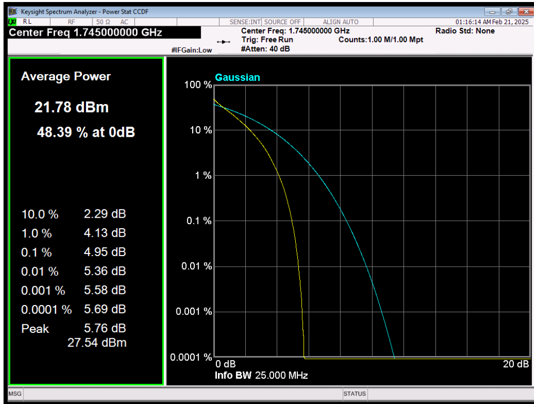
LTE Band66 QPSK BW=10MHz Channel=132322 RB Size=50 Position=#0
