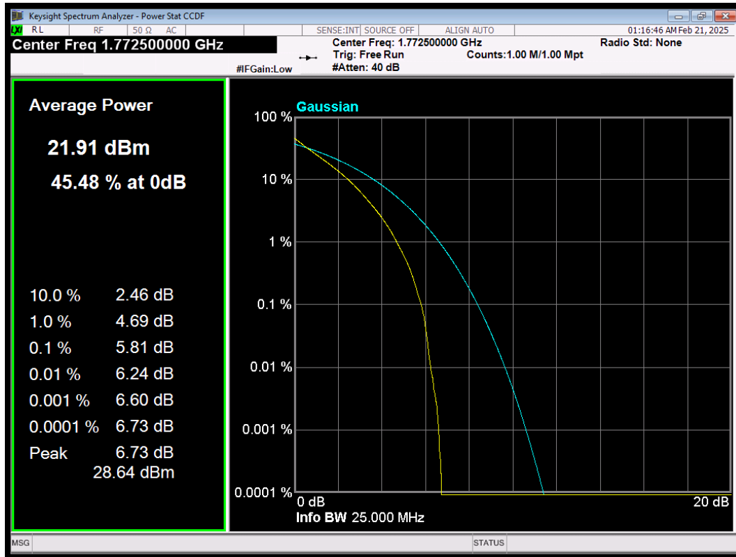
LTE Band66 QPSK BW=15MHz Channel=132597 RB Size=75 Position=#0
