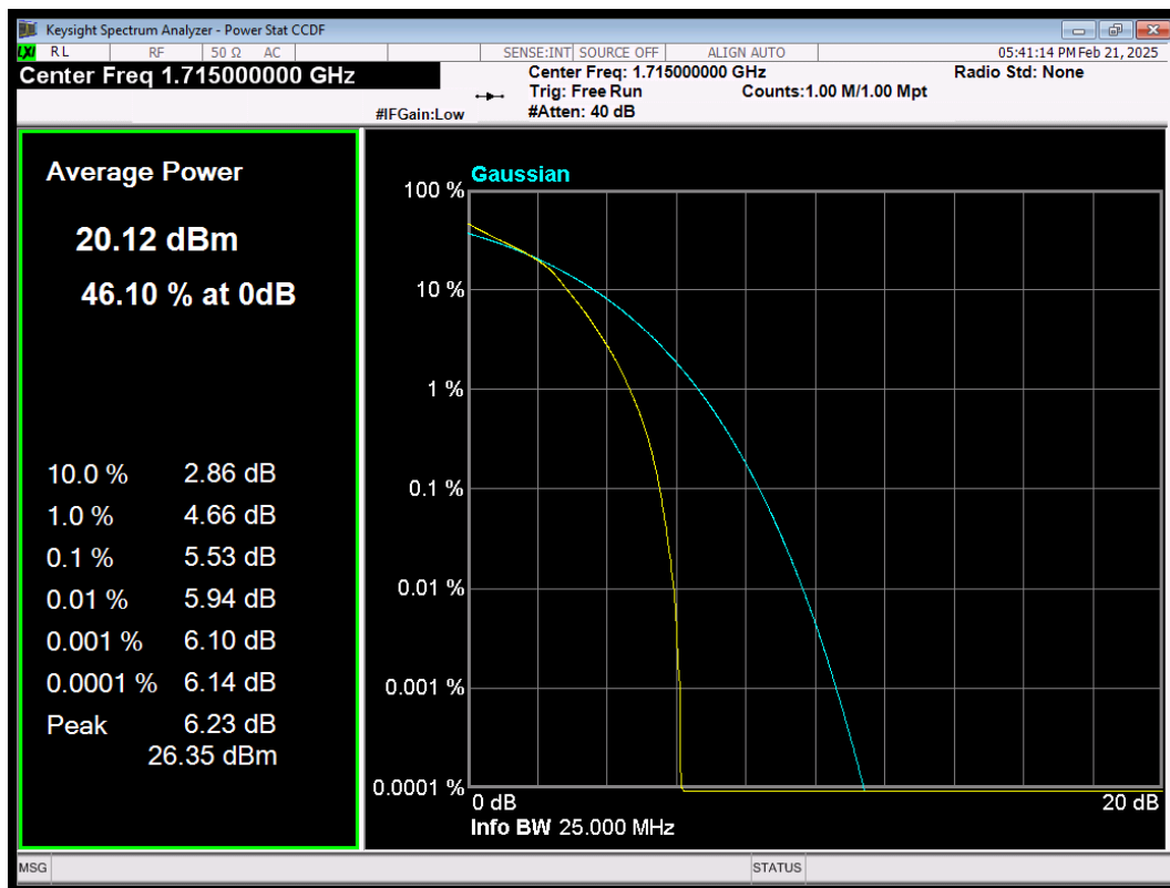
LTE Band66 QAM64 BW=10MHz Channel=132022 RB Size=50 Position=#0
