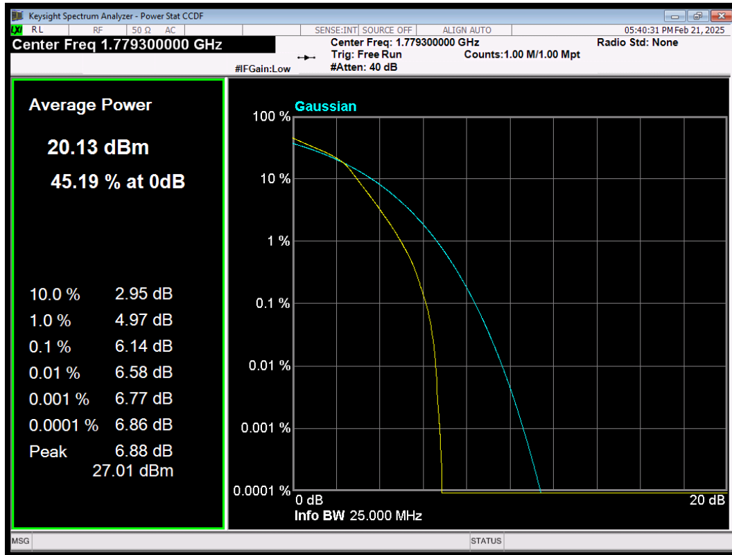
LTE Band66 QAM64 BW=1.4MHz Channel=132665 RB Size=6 Position=#0
