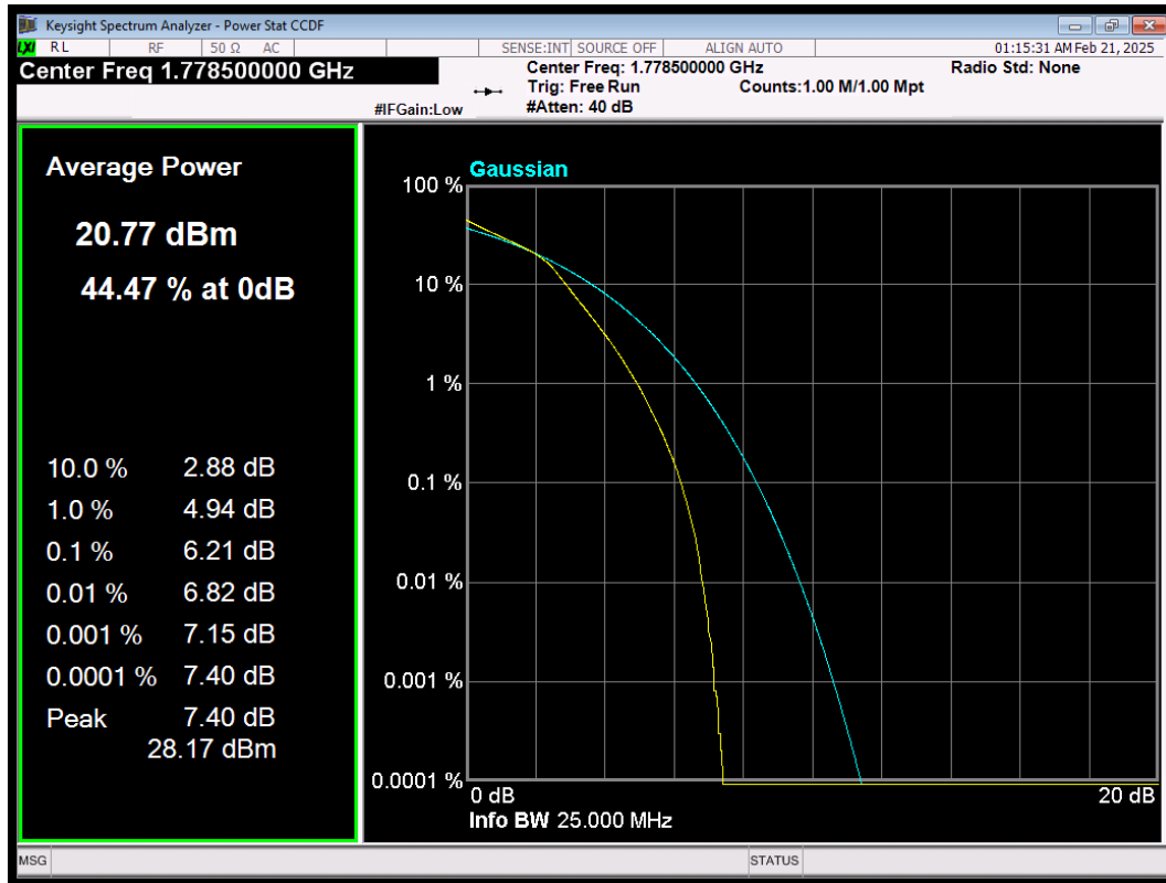
LTE Band66 QAM16 BW=3MHz Channel=132657 RB Size=15 Position=#0
