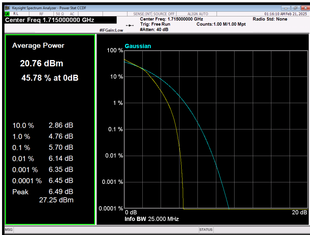
LTE Band66 QAM16 BW=10MHz Channel=132022 RB Size=50 Position=#0
