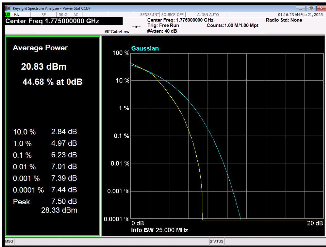
LTE Band66 QAM16 BW=10MHz Channel=132622 RB Size=50 Position=#0
