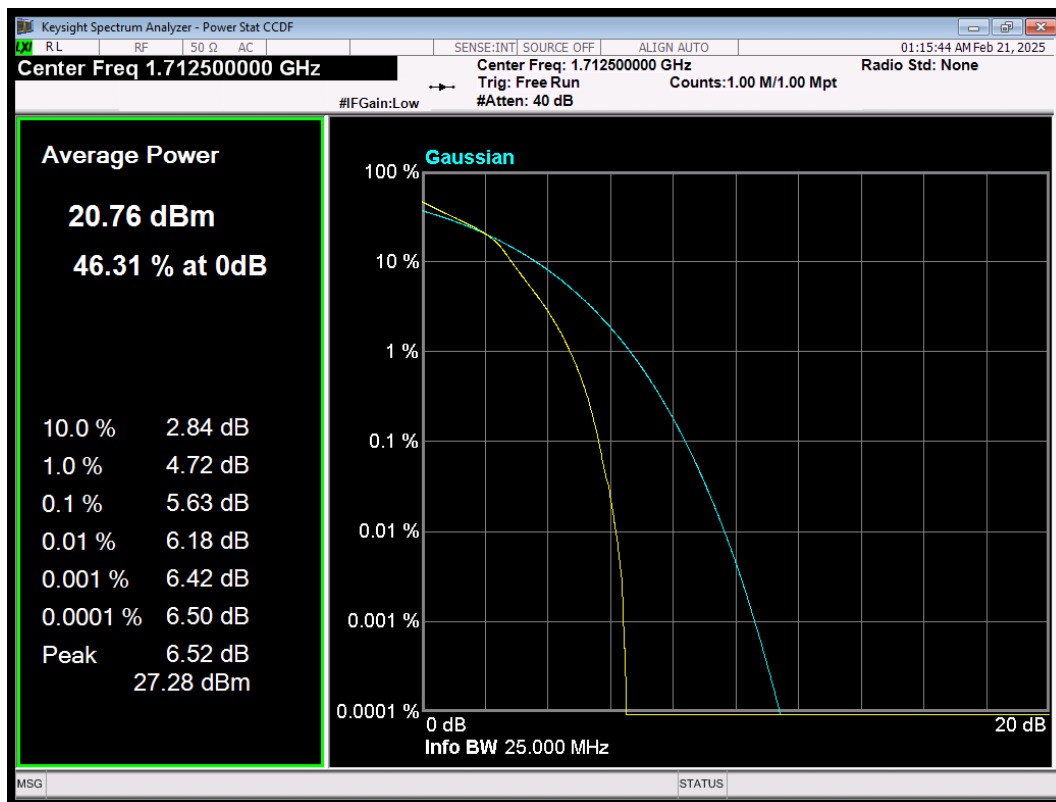
LTE Band66 QAM16 BW=5MHz Channel=131997 RB Size=25 Position=#0
