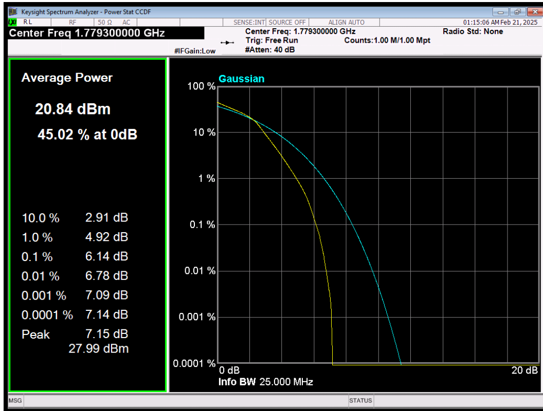
LTE Band66 QAM16 BW=1.4MHz Channel=132665 RB Size=6 Position=#0
