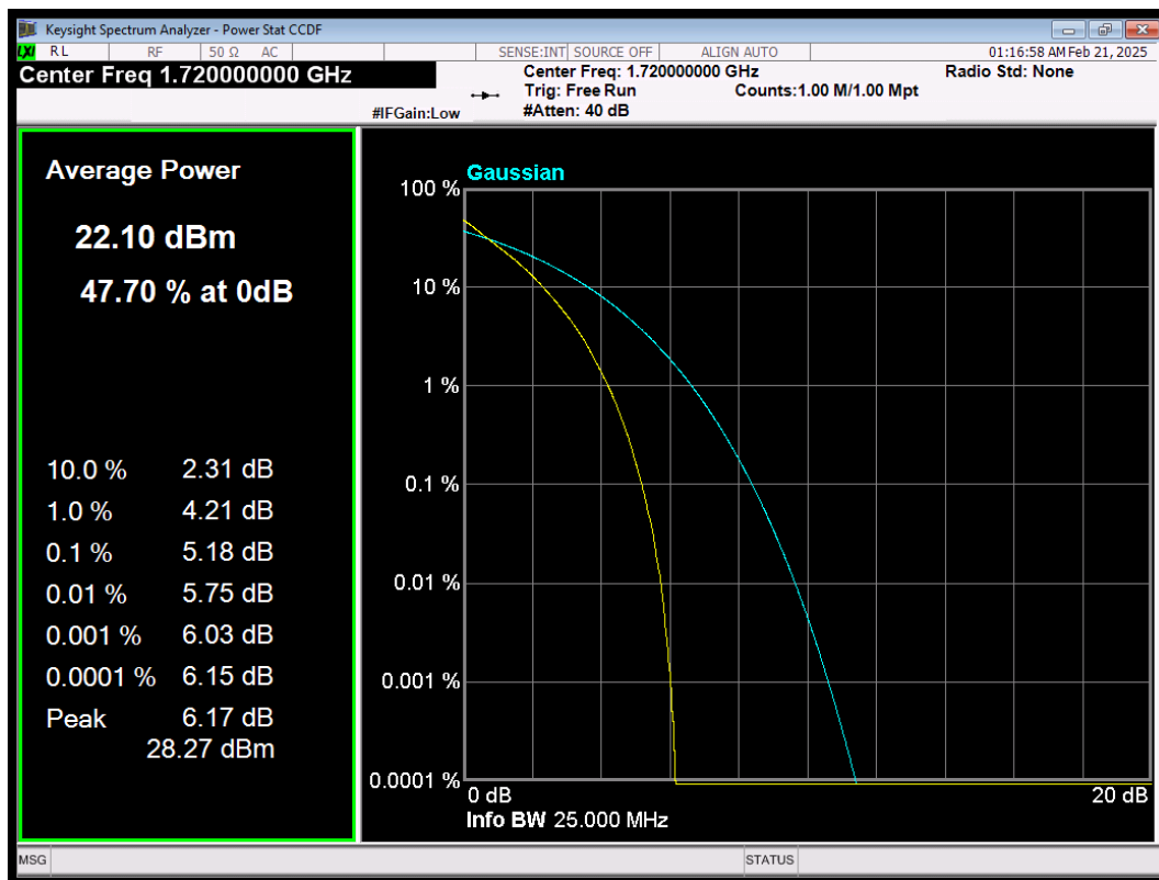
LTE Band66 QPSK BW=20MHz Channel=132072 RB Size=100 Position=#0
