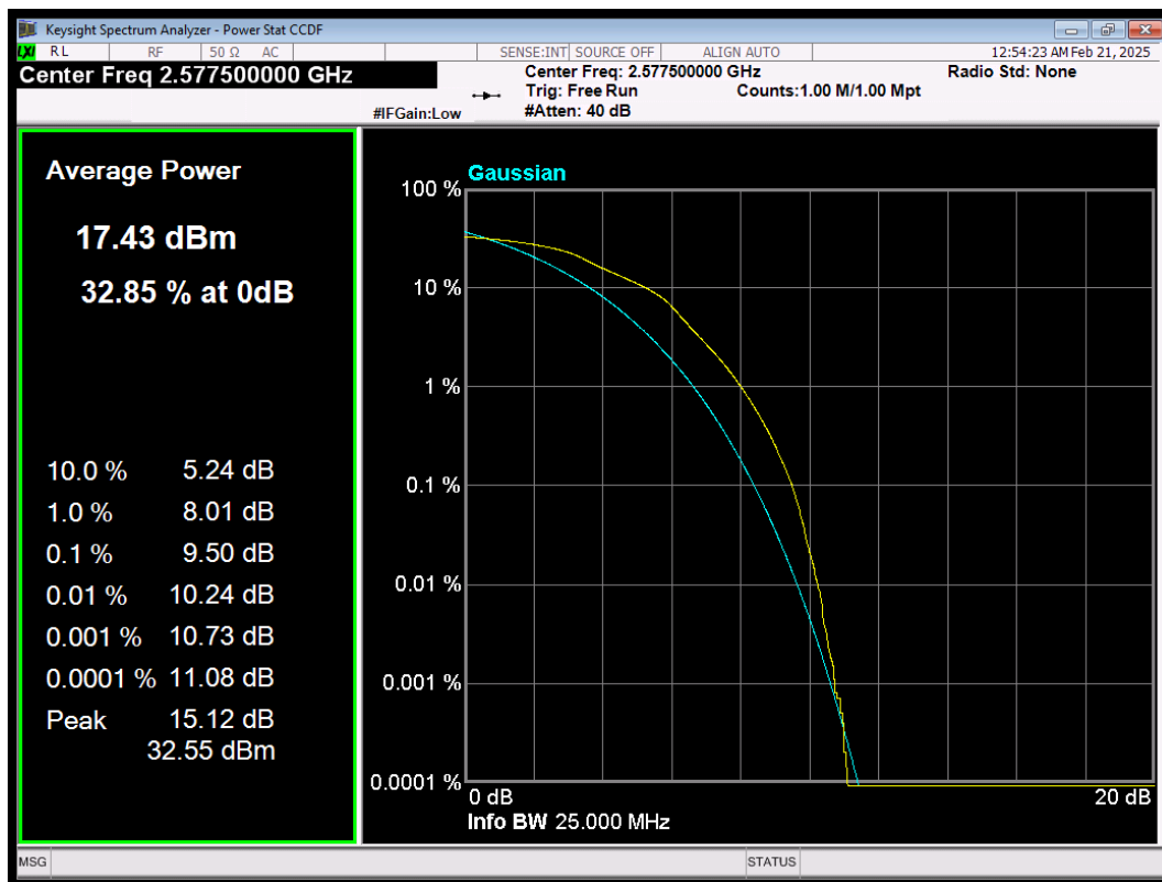
LTE Band38 QAM16 BW=15MHz Channel=37825 RB Size=75 Position=#0
