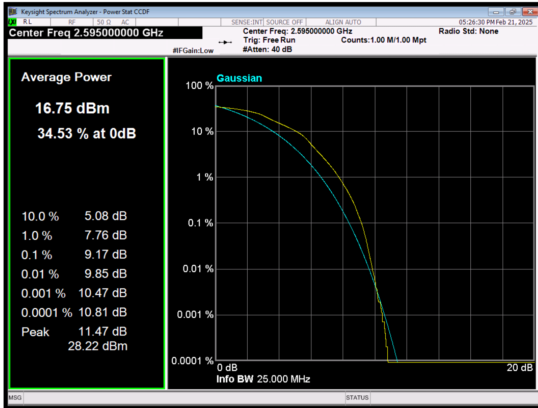
LTE Band38 QAM64 BW=15MHz Channel=38000 RB Size=75 Position=#0
