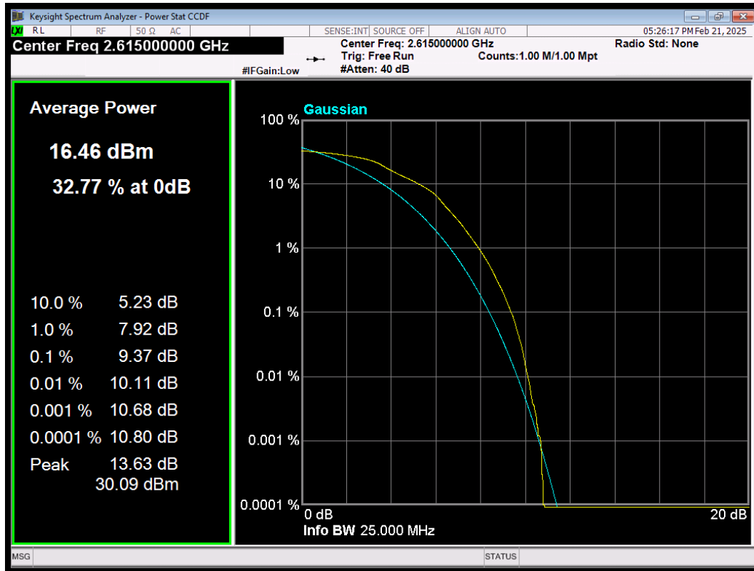
LTE Band38 QAM64 BW=10MHz Channel=38200 RB Size=50 Position=#0
