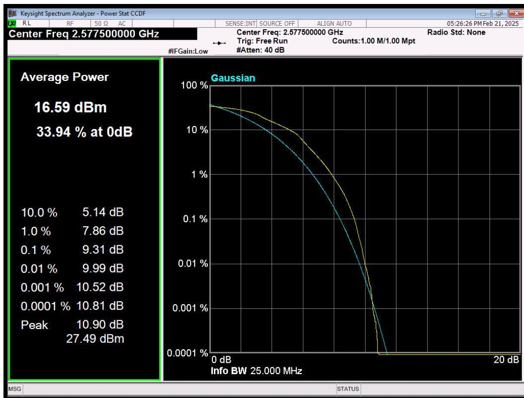
LTE Band38 QAM64 BW=15MHz Channel=37825 RB Size=75 Position=#0
