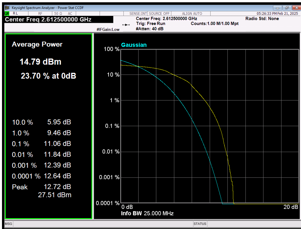
LTE Band38 QAM64 BW=15MHz Channel=38175 RB Size=75 Position=#0
