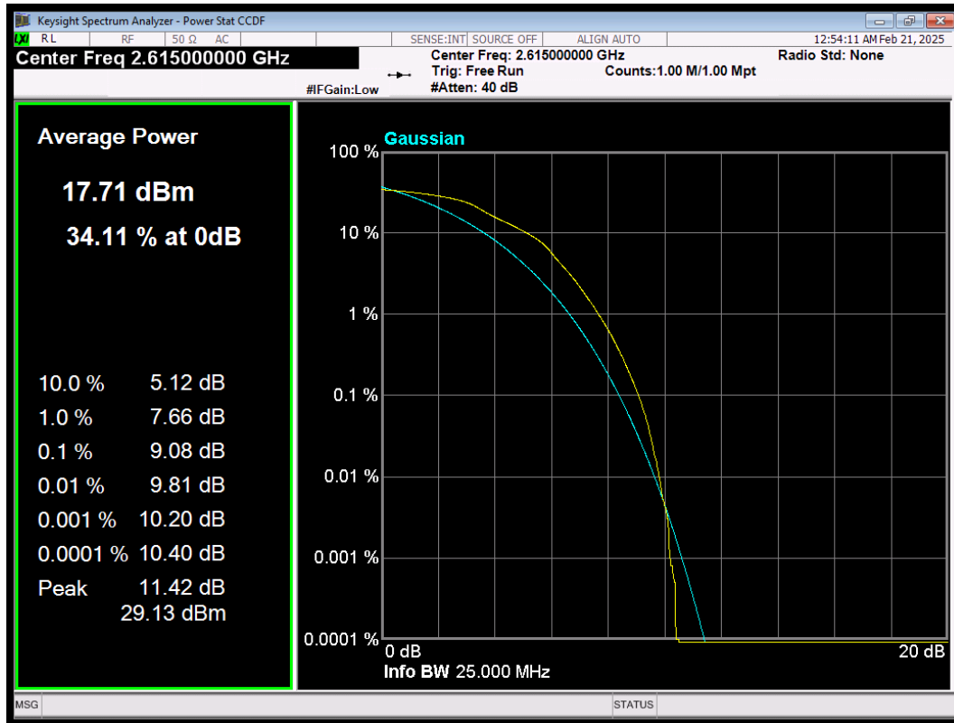
LTE Band38 QAM16 BW=10MHz Channel=38200 RB Size=50 Position=#0
