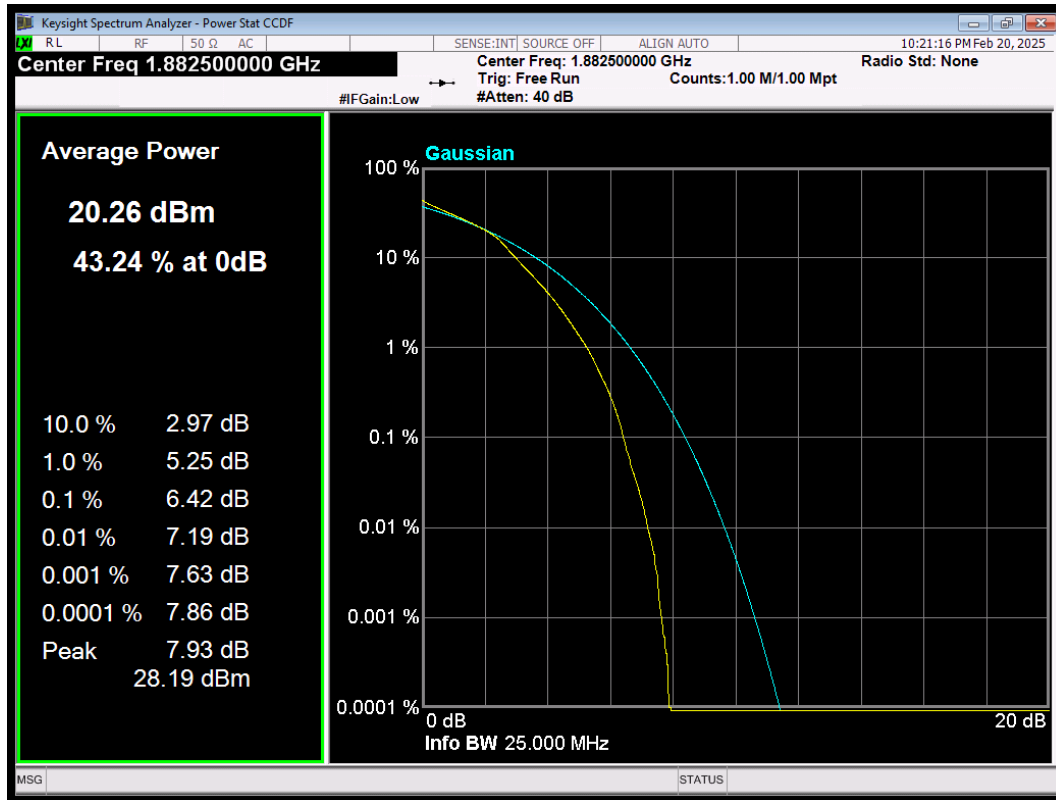
LTE Band25 QAM16 BW=15MHz Channel=26365 RB Size=75 Position=#0
