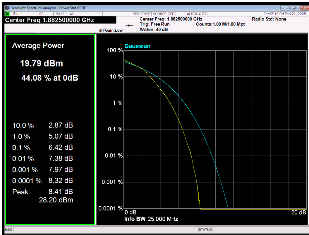
LTE Band25 QAM64 BW=20MHz Channel=26365 RB Size=100 Position=#0
