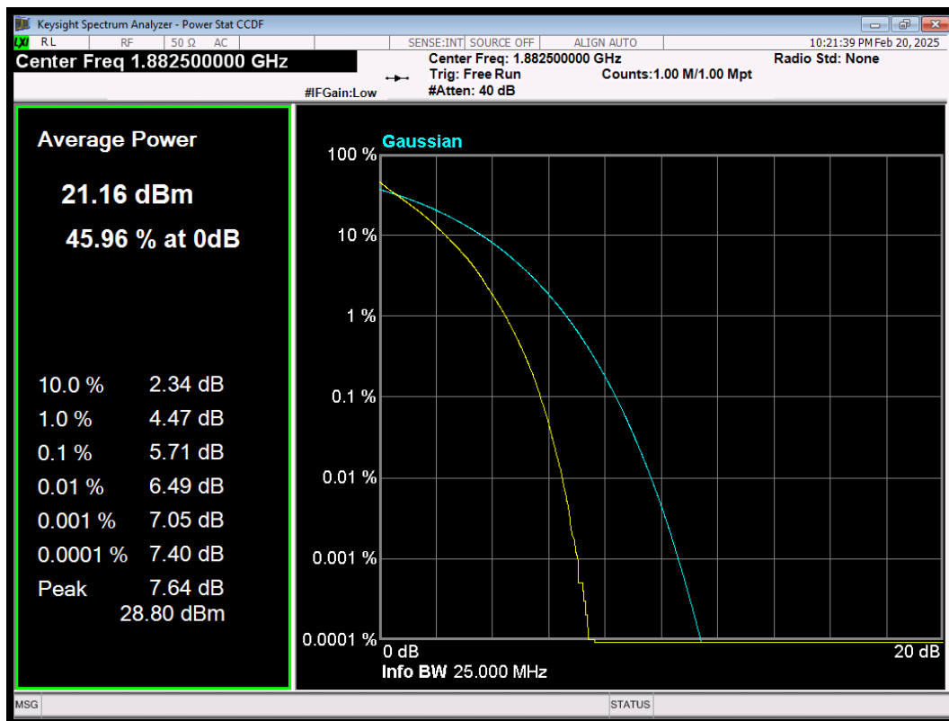
LTE Band25 QPSK BW=20MHz Channel=26365 RB Size=100 Position=#0
