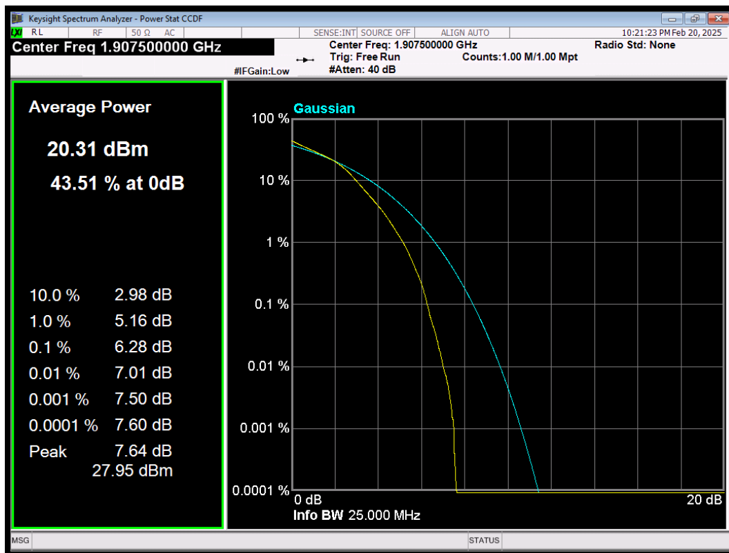
LTE Band25 QAM16 BW=15MHz Channel=26615 RB Size=75 Position=#0
