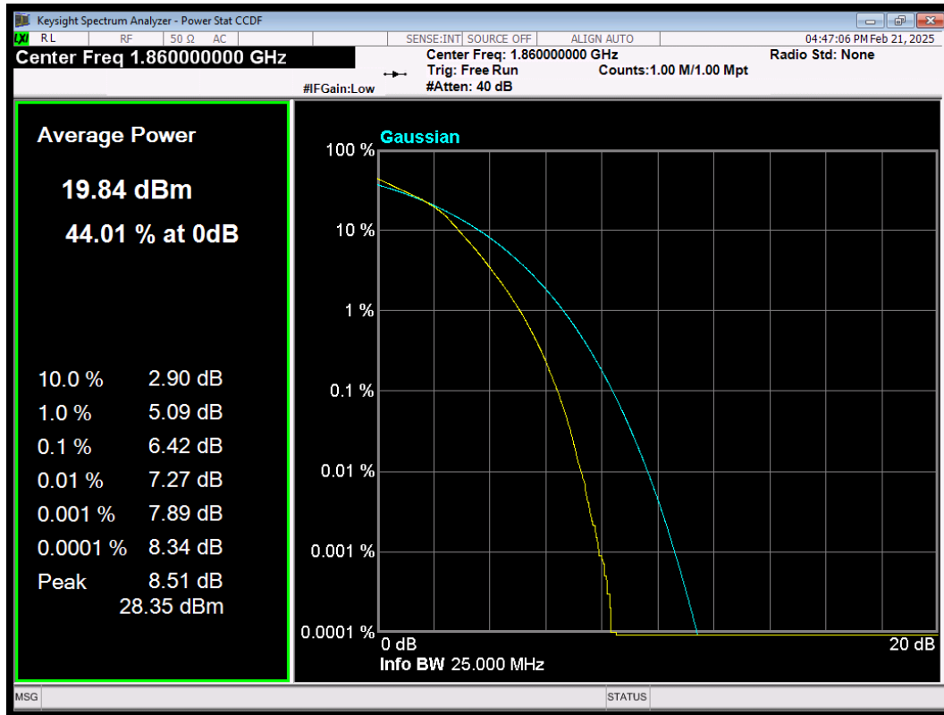
LTE Band25 QAM64 BW=20MHz Channel=26140 RB Size=100 Position=#0
