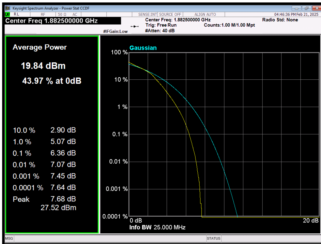
LTE Band25 QAM64 BW=10MHz Channel=26365 RB Size=50 Position=#0
