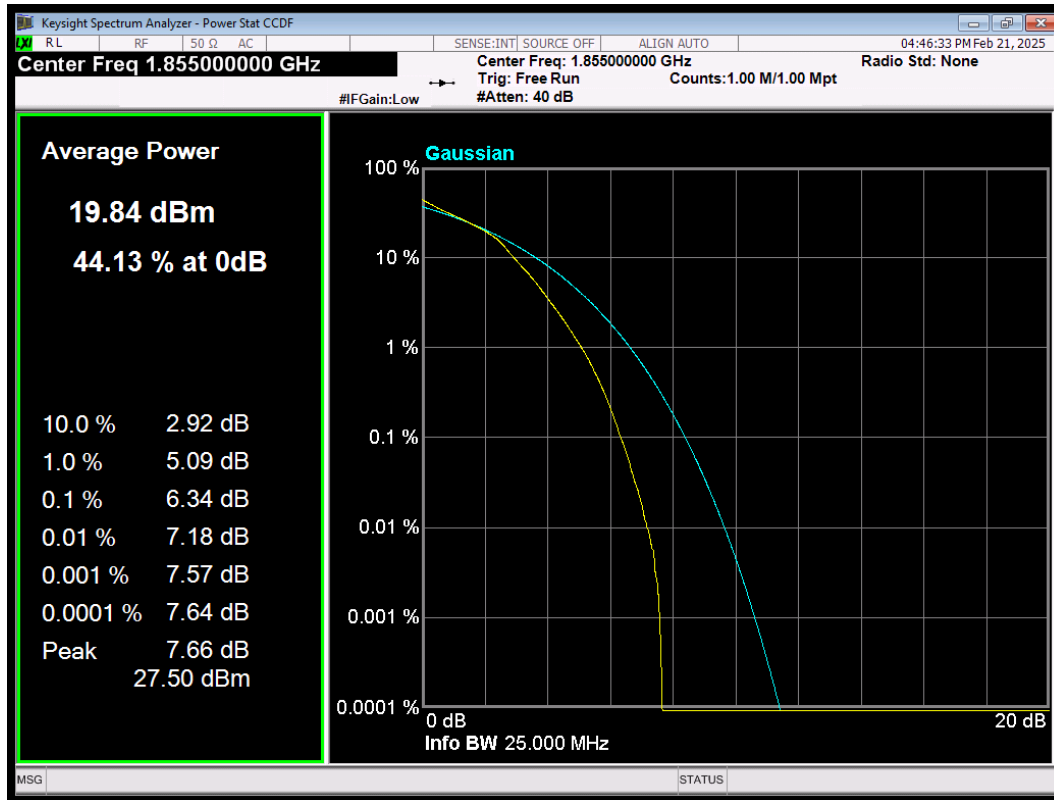
LTE Band25 QAM64 BW=10MHz Channel=26090 RB Size=50 Position=#0
