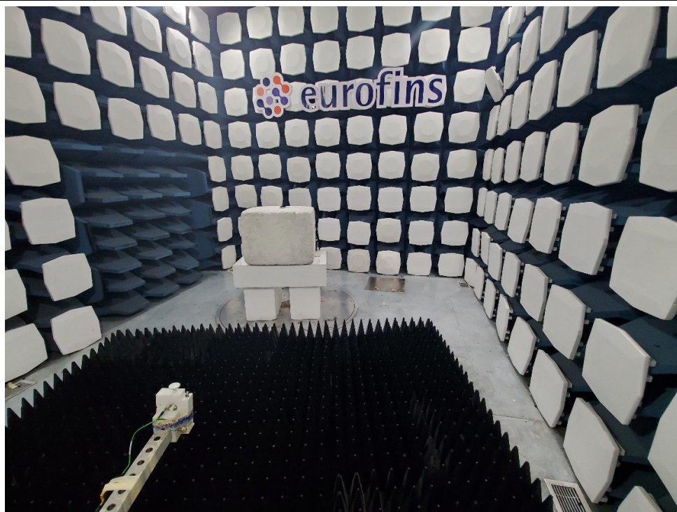
Picture 1 Radiated Emission Test Setup
