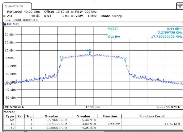
802.11n20_5280MHz
