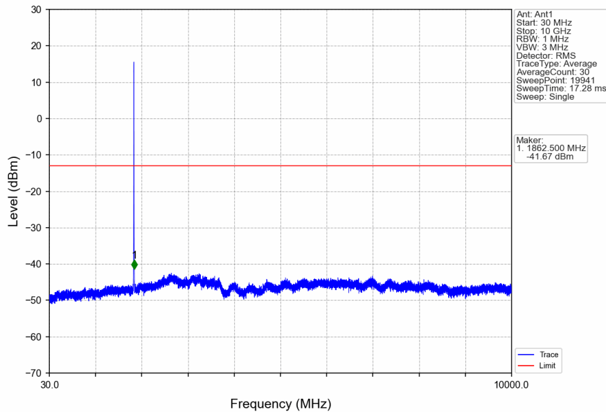
Band2_RMC_LCH_1852.4MHz_12.2kbps RMC_NTNV
