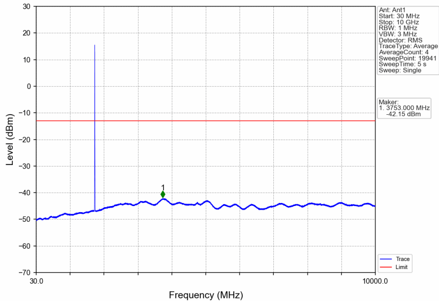
Band4_RMC_HCH_1752.6MHz_12.2kbps RMC_NTNV
