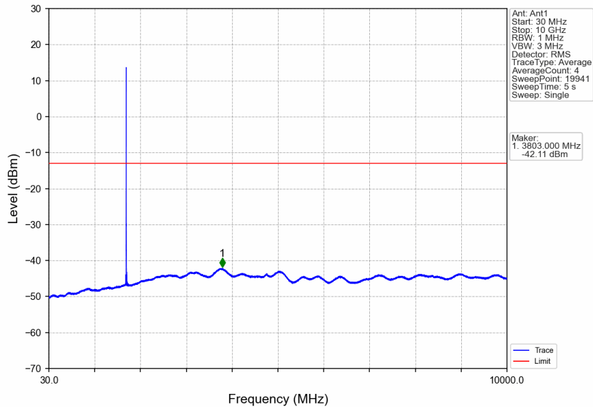
Band4_HSDPA_LCH_1712.4MHz_Subtest 1_NTNV
