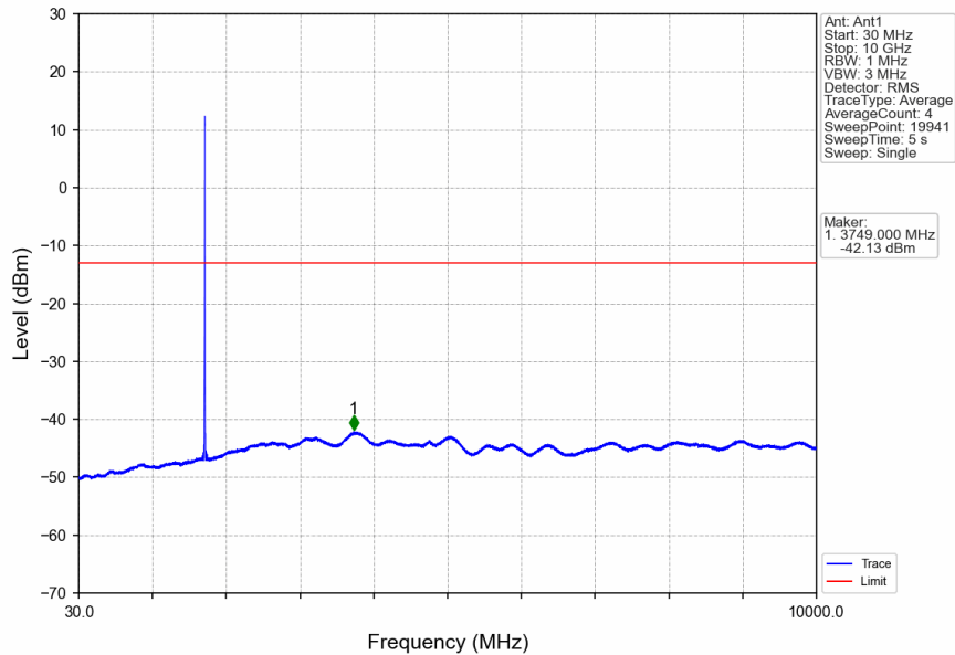
Band4_HSDPA_MCH_1732.6MHz_Subtest 1_NTNV
