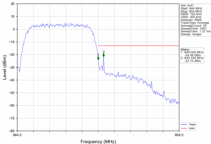
Band5_HSUPA_HCH_846.6MHz_Subtest 1_NTNV
