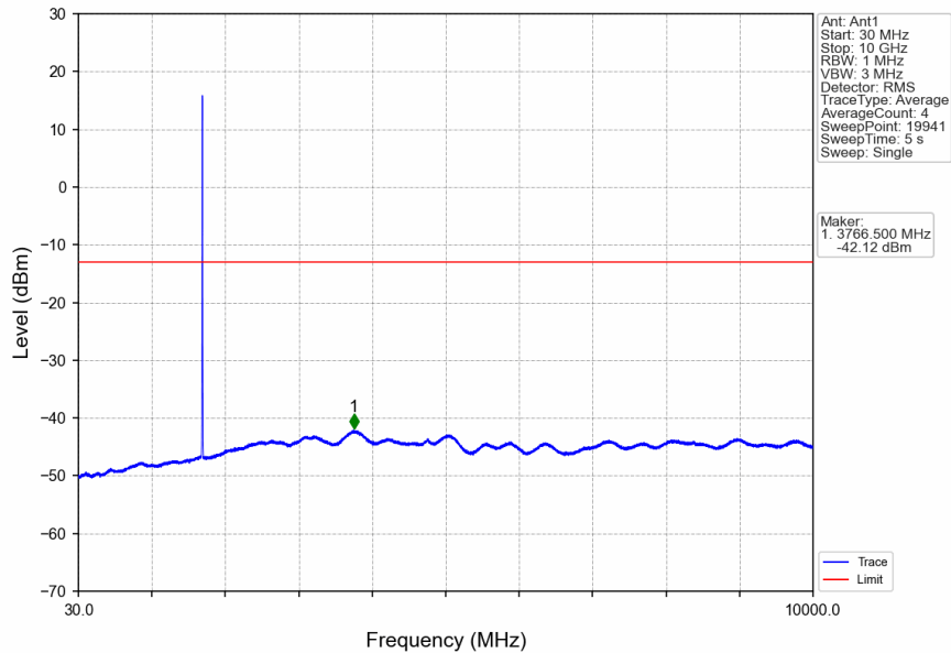
Band4_RMC_LCH_1712.4MHz_12.2kbps RMC_NTNV
