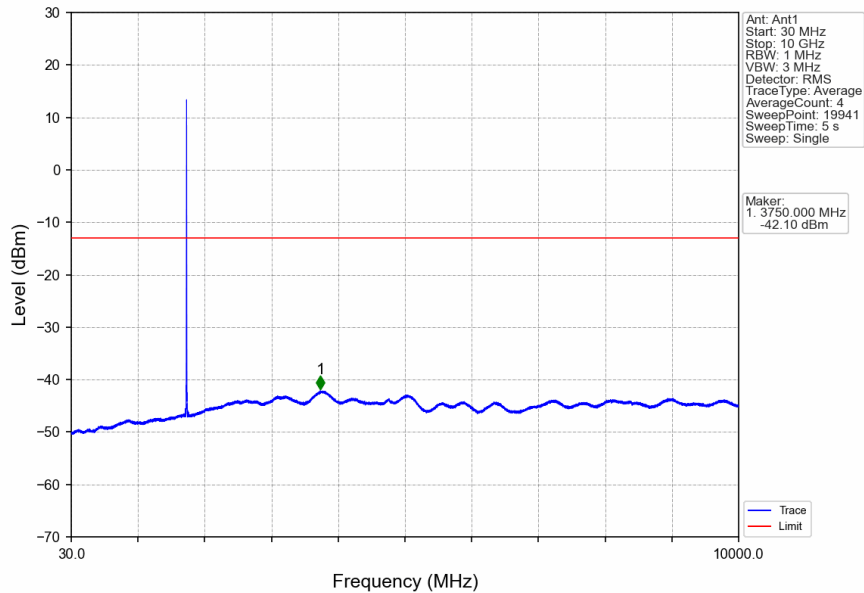
Band4_HSDPA_HCH_1752.6MHz_Subtest 1_NTNV
