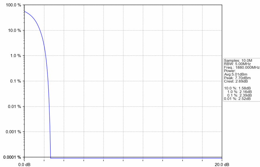
Band2_RMC_MCH_1880MHz_12.2kbps RMC_NTNV
