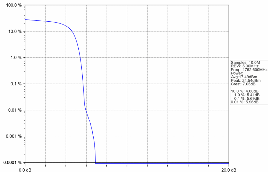
Band4_HSDPA_HCH_1752.6MHz_Subtest 1_NTNV
