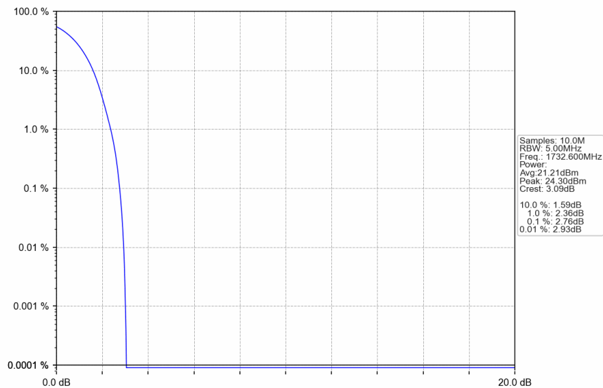
Band4_RMC_MCH_1732.6MHz_12.2kbps RMC_NTNV
