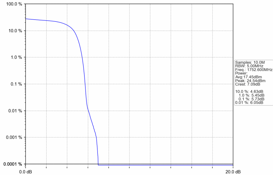
Band4_HSUPA_HCH_1752.6MHz_Subtest 1_NTNV
