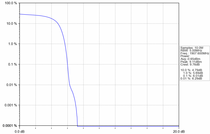
Band2_HSUPA_HCH_1907.6MHz_Subtest 1_NTNV
