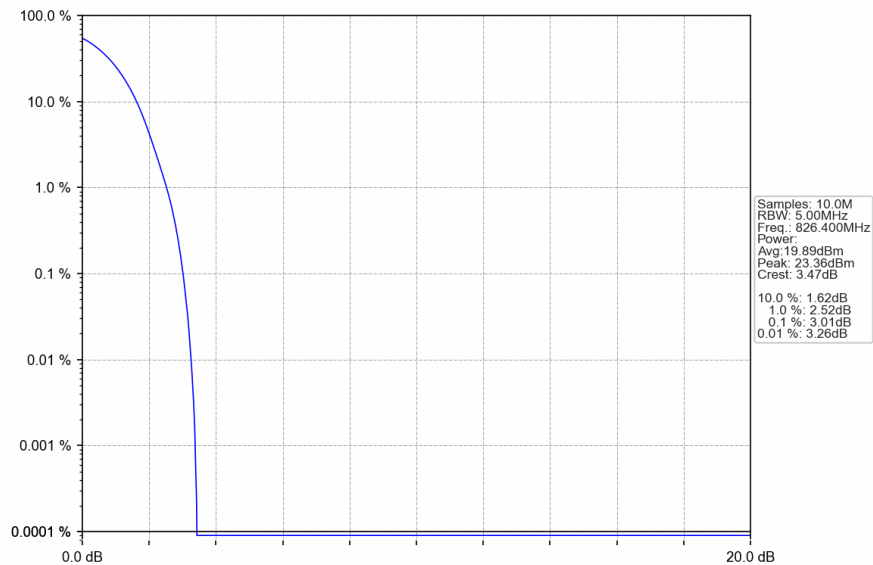
Band5_RMC_LCH_826.4MHz_12.2kbps RMC_NTNV
