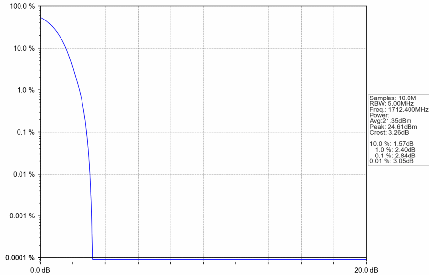
Band4_RMC_LCH_1712.4MHz_12.2kbps RMC_NTNV
