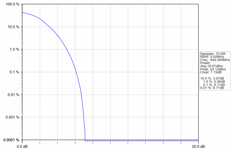
Band26b_10MHz_16QAM_HCH_844MHz_RB_50_0_NTNV
