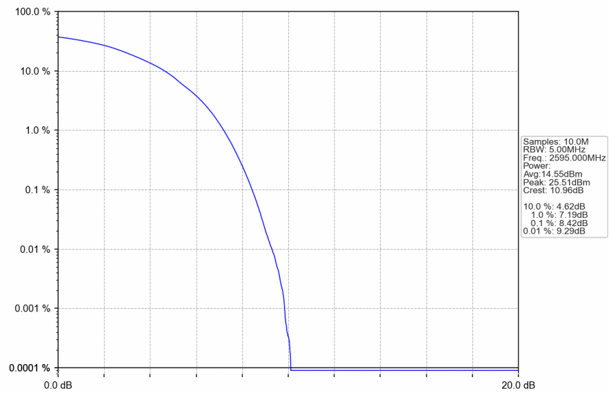
Band38_15MHz_16QAM_MCH_2595.000MHz_RB_75_0_NTNV
