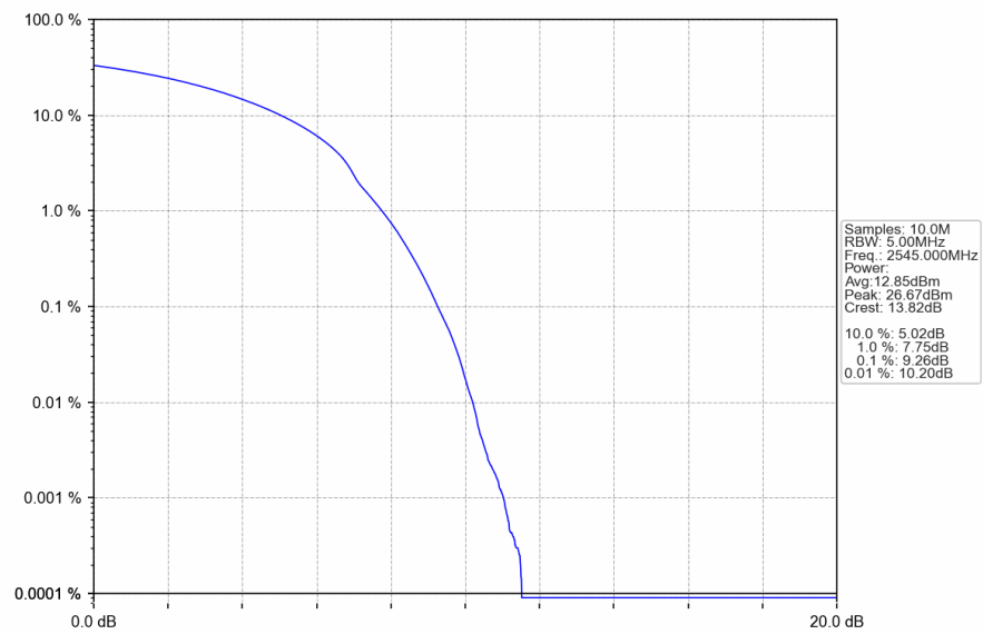
Band41_20MHz_16QAM_LCH_2545MHz_RB_100_0_NTNV
