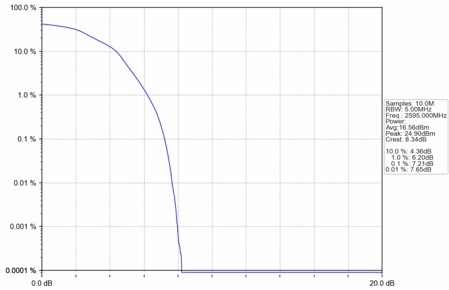
Band41_5MHz_16QAM_MCH_2595MHz_RB_25_0_NTNV
