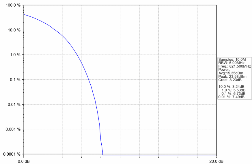
Band26c_15MHz_16QAM_LCH_821.5MHz_RB_75_0_NTNV
