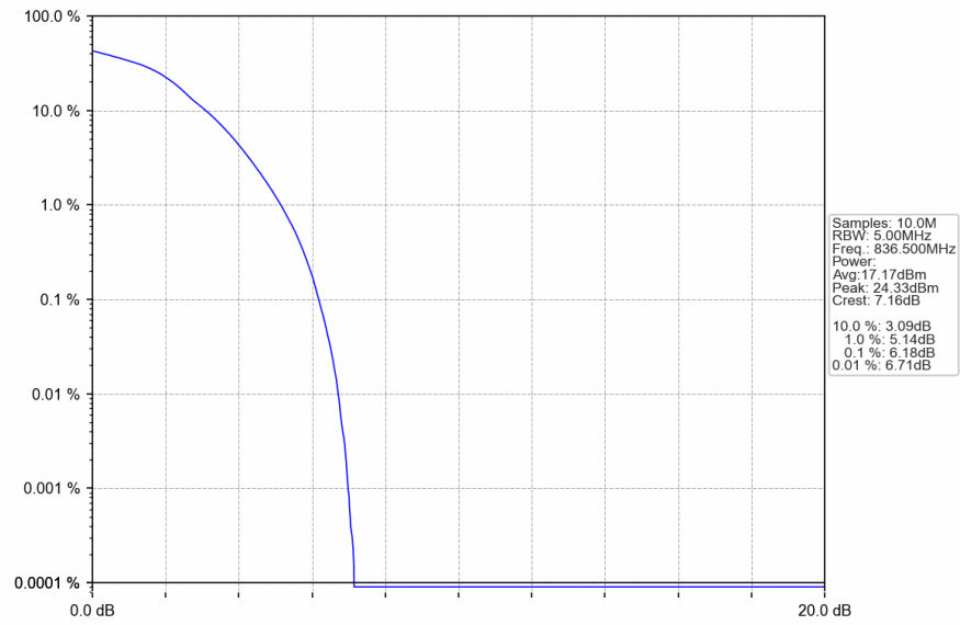
Band26b_10MHz_16QAM_MCH_836.5MHz_RB_50_0_NTNV
