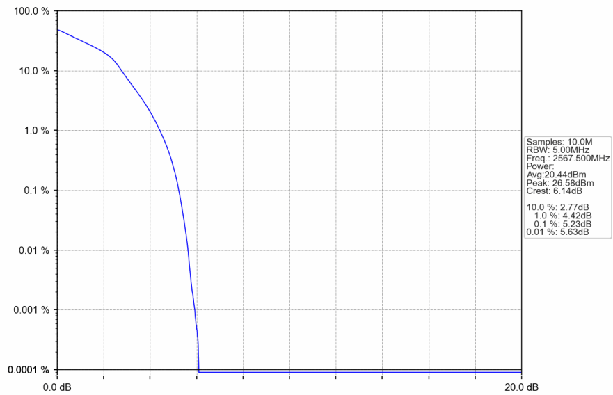
Band7_5MHz_16QAM_HCH_2567.500MHz_RB_25_0_NTNV
