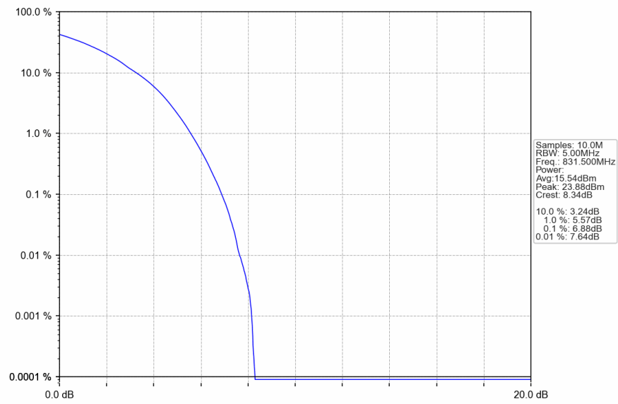
Band26c_15MHz_16QAM_MCH_831.5MHz_RB_75_0_NTNV
