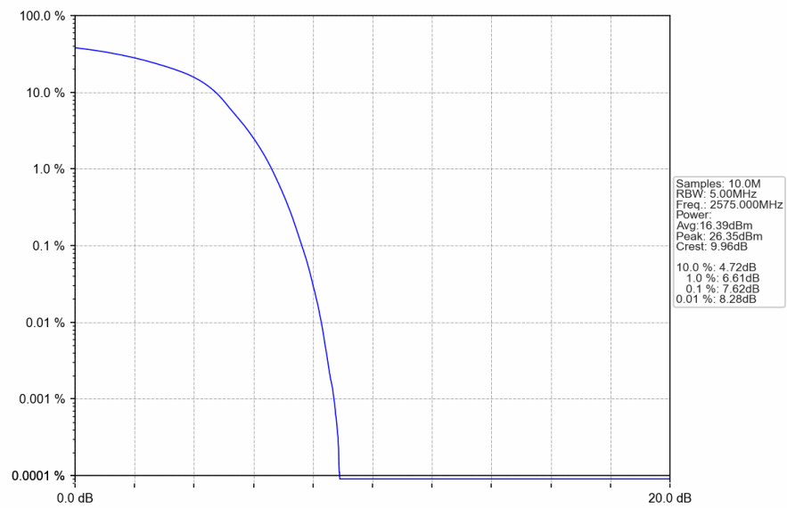
Band38_10MHz_16QAM_LCH_2575MHz_RB_50_0_NTNV
