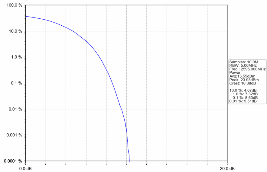
Band41_15MHz_16QAM_MCH_2595MHz_RB_75_0_NTNV
