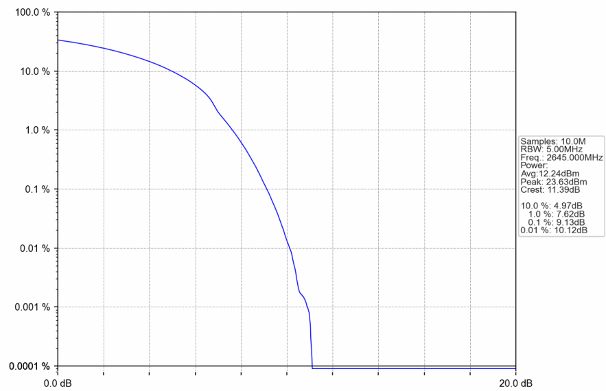
Band41_20MHz_16QAM_HCH_2645MHz_RB_100_0_NTNV
