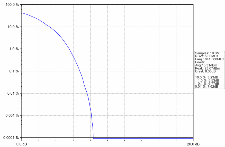
Band26c_15MHz_16QAM_HCH_841.5MHz_RB_75_0_NTNV
