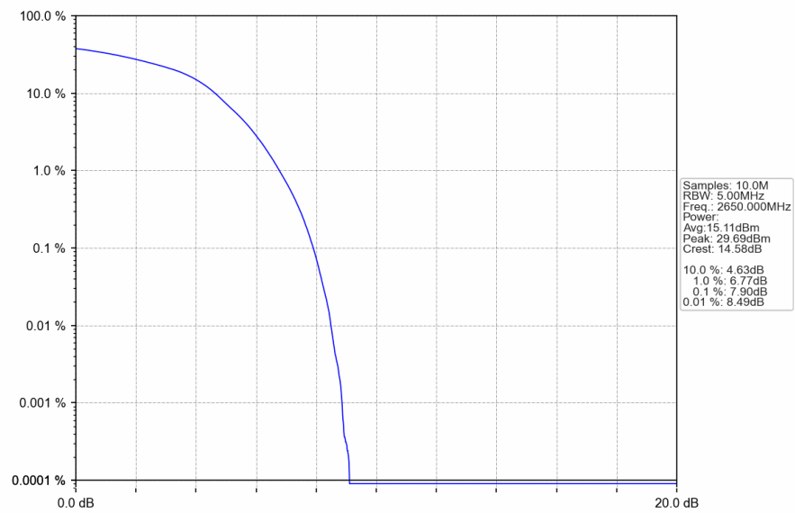
Band41_10MHz_16QAM_HCH_2650MHz_RB_50_0_NTNV
