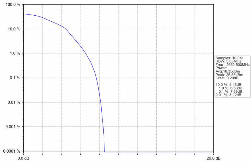
Band41_5MHz_16QAM_HCH_2652.5MHz_RB_25_0_NTNV
