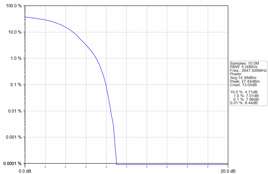
Band41_15MHz_QPSK_HCH_2647.5MHz_RB_75_0_NTNV
