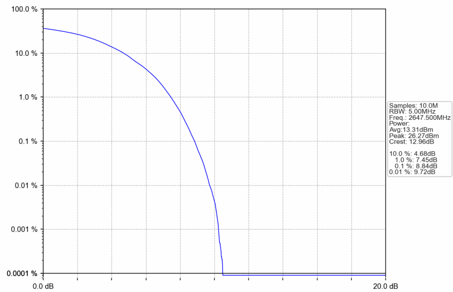
Band41_15MHz_16QAM_HCH_2647.5MHz_RB_75_0_NTNV
