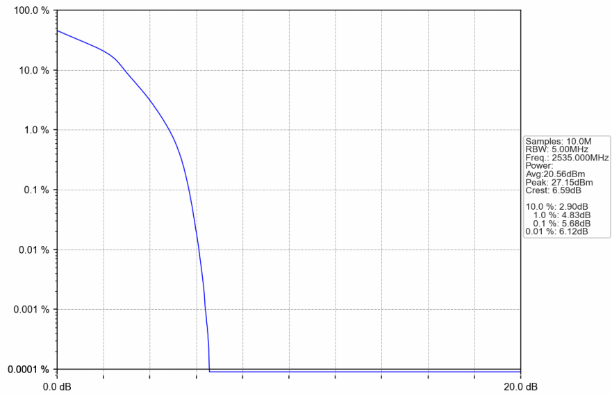
Band7_5MHz_16QAM_MCH_2535.000MHz_RB_25_0_NTNV
