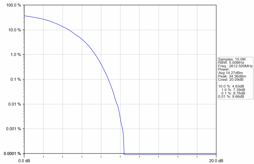
Band38_15MHz_16QAM_HCH_2612.500MHz_RB_75_0_NTNV
