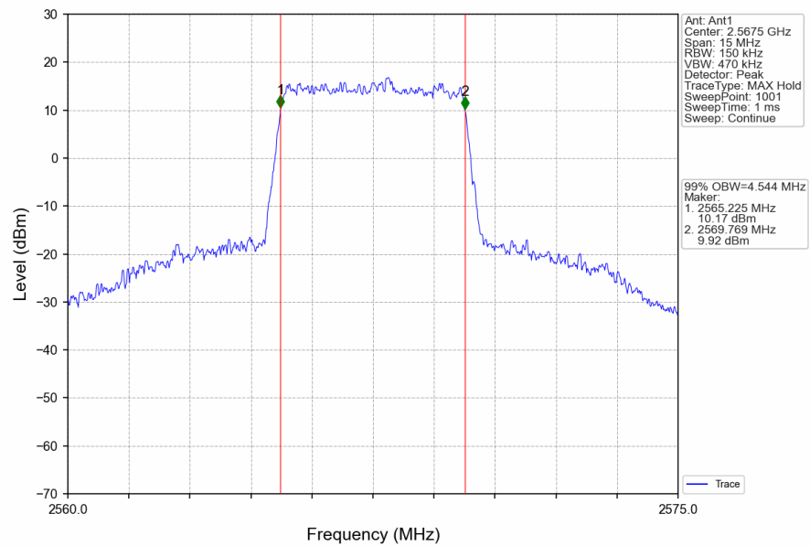
Band7_5MHz_16QAM_HCH_2567.5MHz_RB_25_0_NTNV
