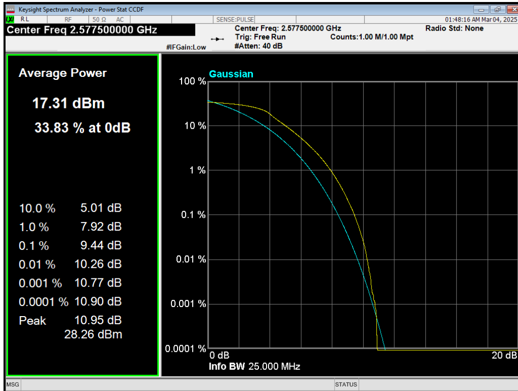
Band38 QPSK BW=15MHz Channel=37825 RB Size=75 Position=#0.png
