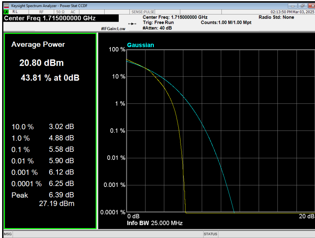
Band4 16QAM BW=10MHz Channel=20000 RB Size=50 Position=#0.png
