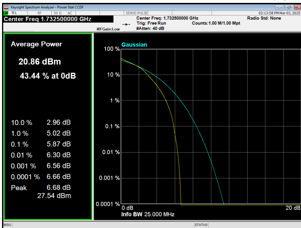
Band4 16QAM BW=10MHz Channel=20175 RB Size=50 Position=#0.png
