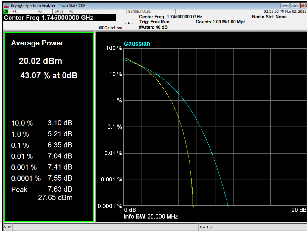
Band4 64QAM BW=20MHz Channel=20300 RB Size=100 Position=#0.png
