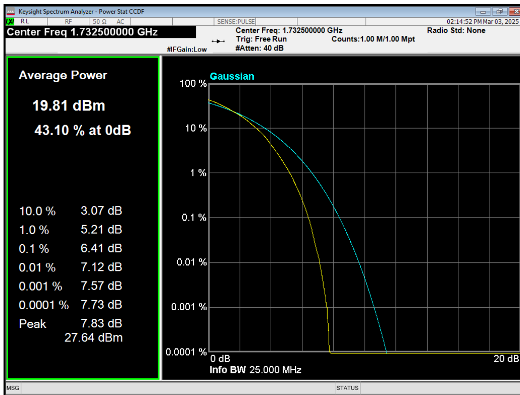
Band4 64QAM BW=20MHz Channel=20175 RB Size=100 Position=#0.png
