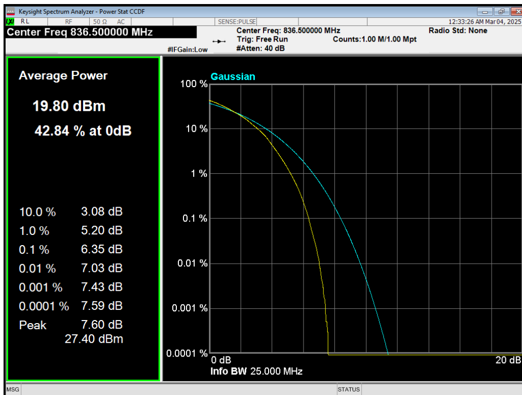
Band26(824-849) 64QAM BW=10MHz Channel=26915 RB Size=50 Position=#0.png
