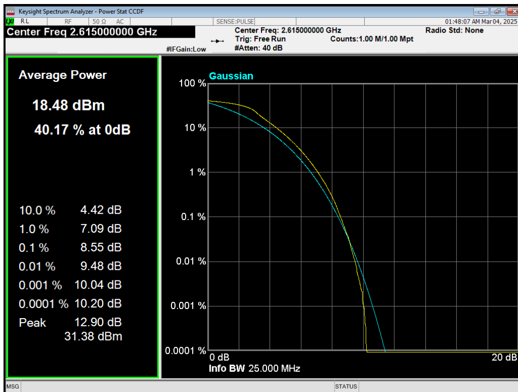
Band38 QPSK BW=10MHz Channel=38200 RB Size=50 Position=#0.png
