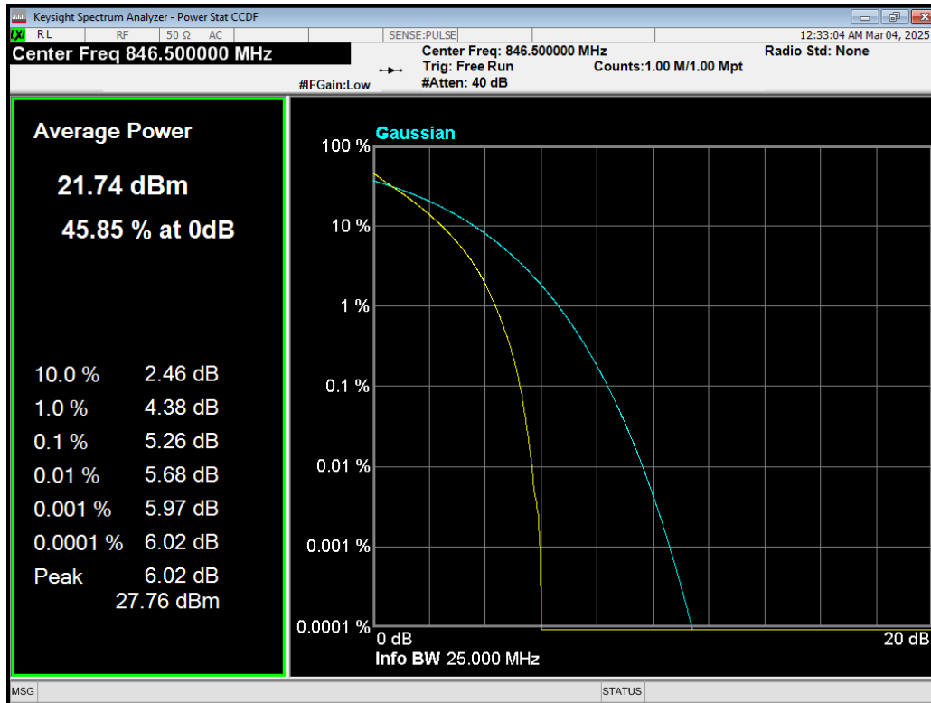
Band26(824-849) QPSK BW=5MHz Channel=27015 RB Size=25 Position=#0.png
