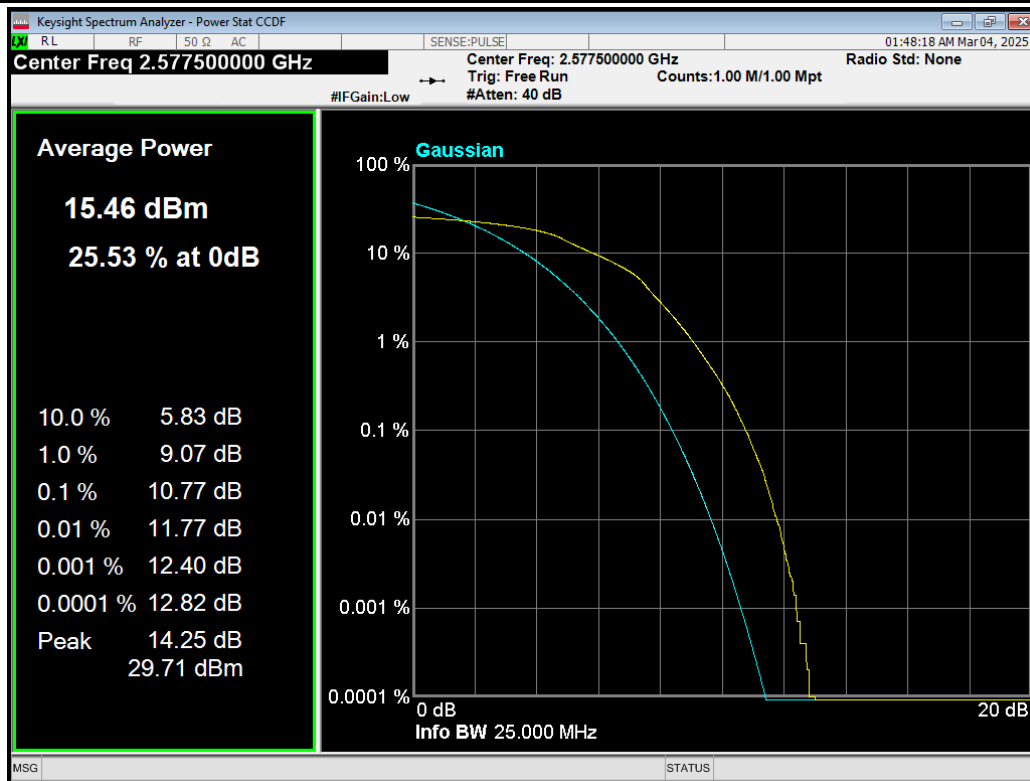
Band38 16QAM BW=15MHz Channel=37825 RB Size=75 Position=#0.png
