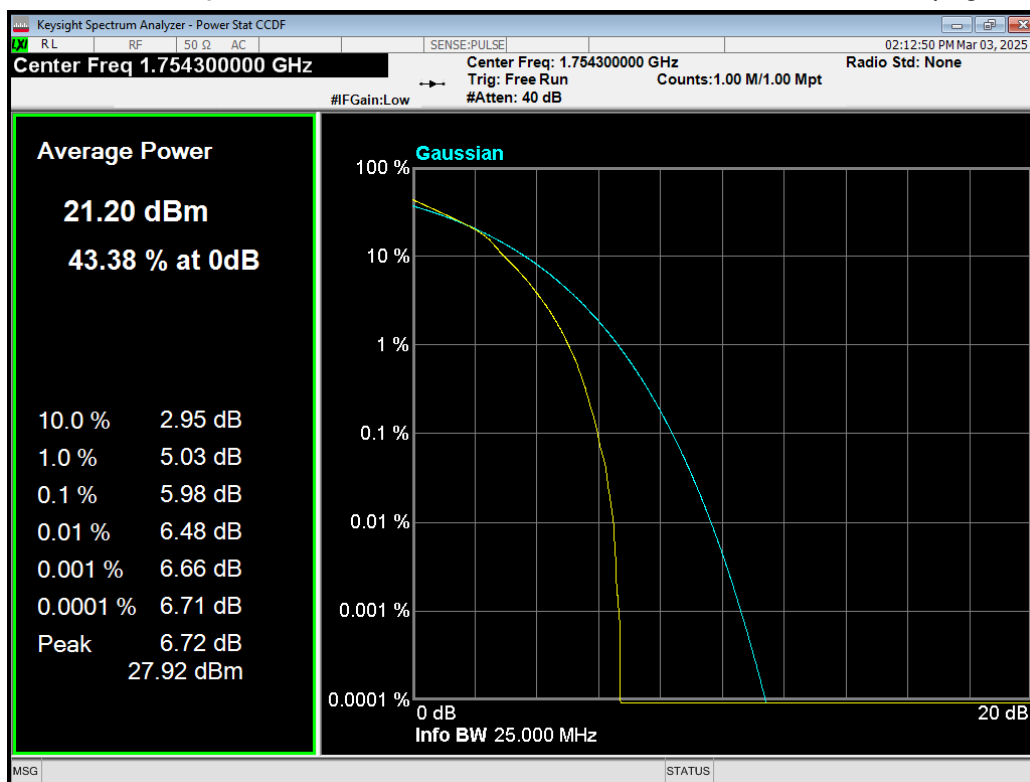
Band4 16QAM BW=1.4MHz Channel=20393 RB Size=6 Position=#0.png
