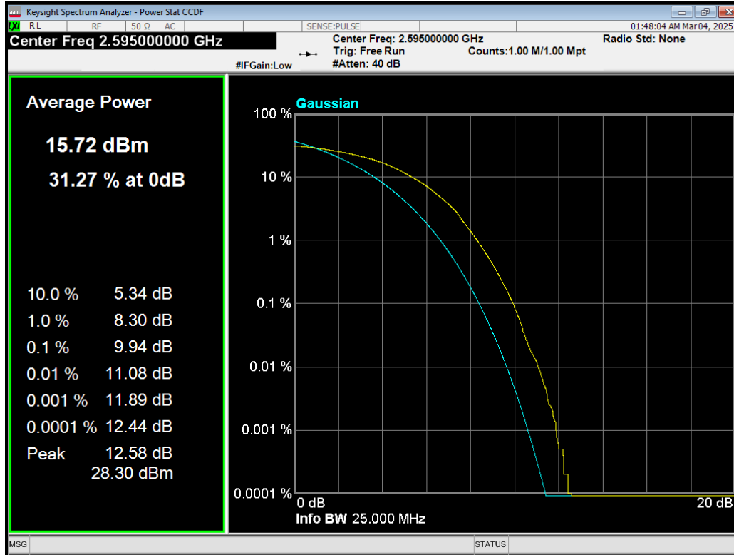
Band38 64QAM BW=10MHz Channel=38000 RB Size=50 Position=#0.png
