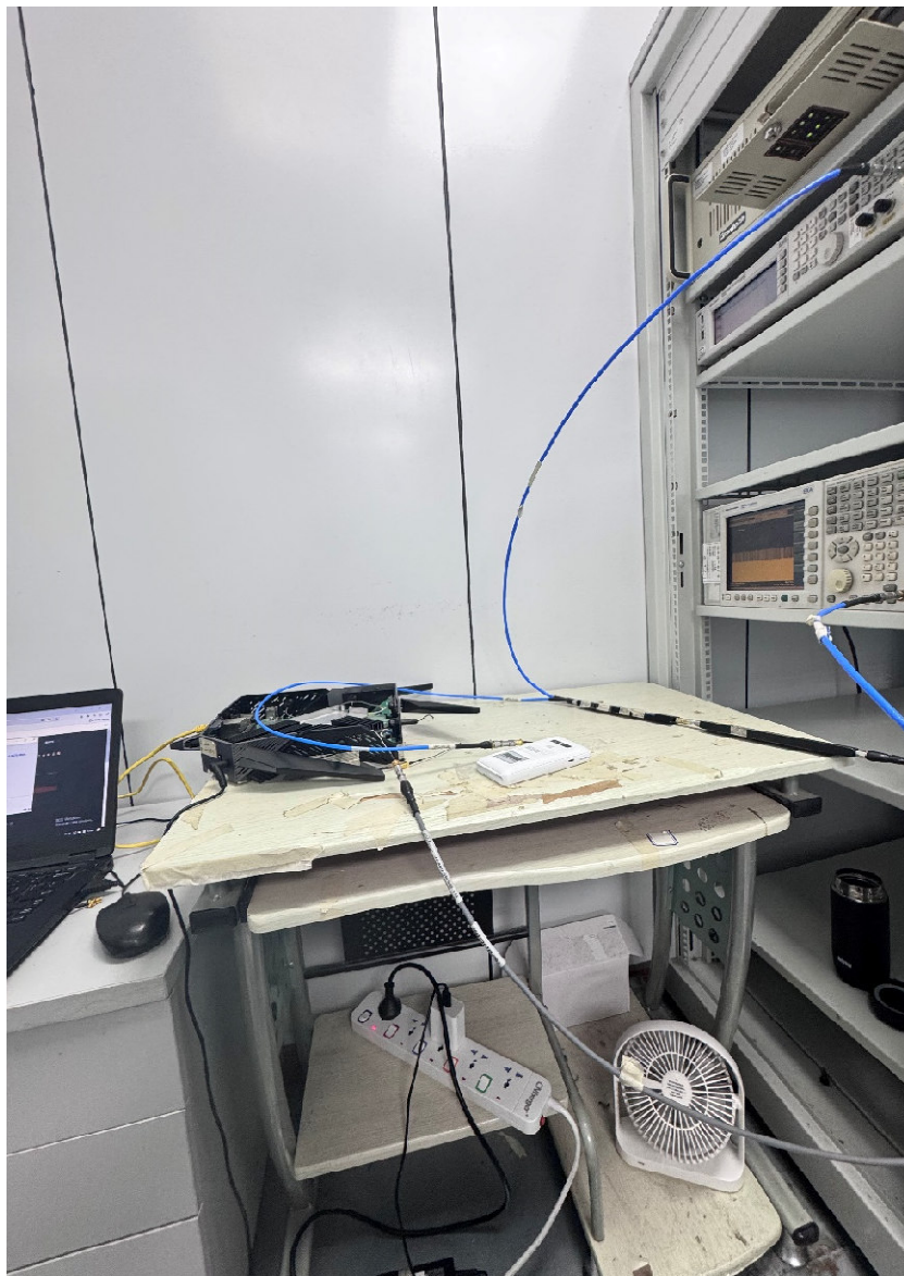
Picture 1 DFS Test Setup
