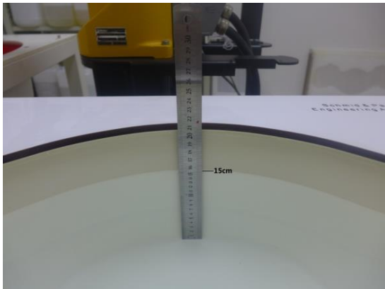
Photo 5: Tissue Simulant Liquid for Head 2450
