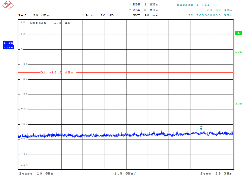
RF Conducted Spurious Emissions_BLE_2440_Ant1
