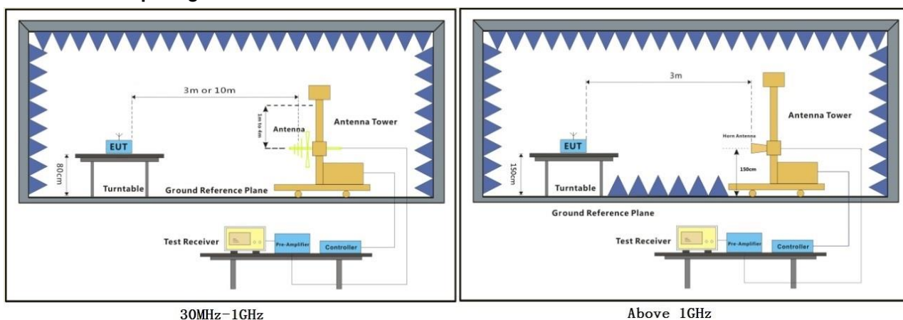
30MHz-1GHz
