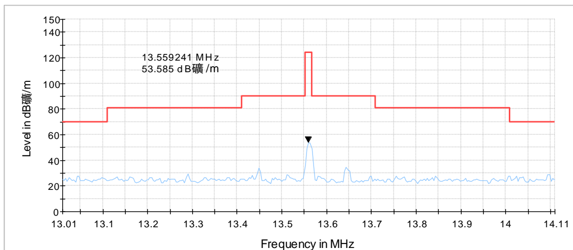
Radiates Emission from 13.01MHz to 14.11MHz
