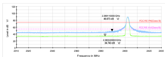
Bluetooth LE (1M) Channel 0 Peak+ Average
