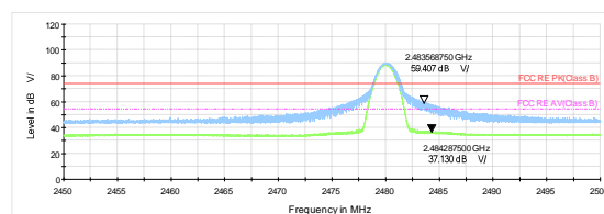
Bluetooth LE (1M) Channel 39 Peak+Average
