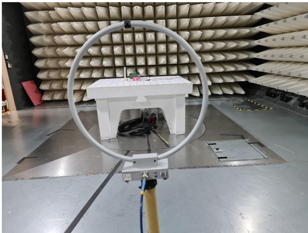
Radiated Emission measurement setup
