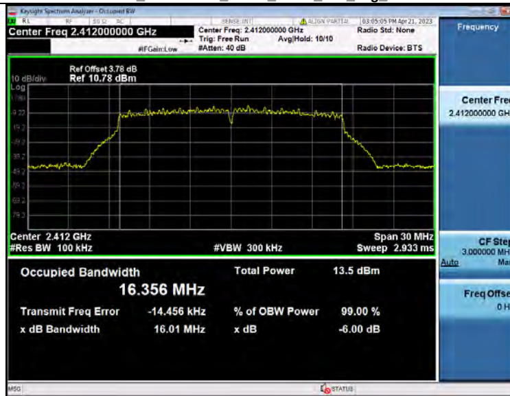
-6dB Bandwidth_NVNT_ANT2_802_11g_2412
