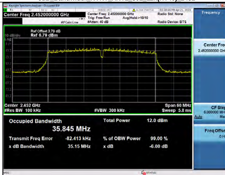
-6dB_Bandwidth_NVNT_ANT2_802_11n(HT40)_2452
