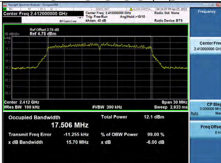
-6dB_Bandwidth_NVNT_ANT3_802_11n(HT20)_2412
