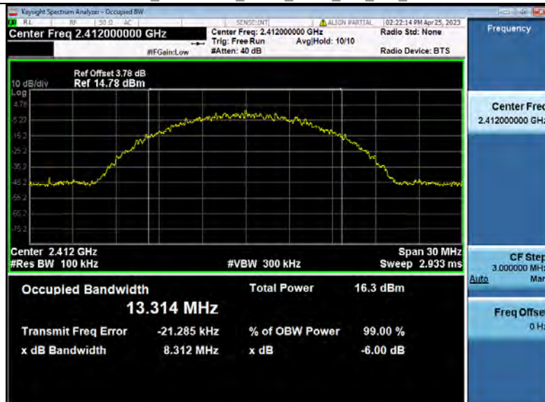
-6dB_Bandwidth_NVNT_ANT1_802_11b_2412
