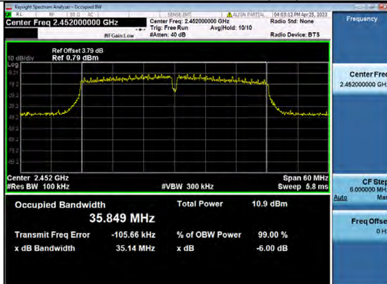
-6dB_Bandwidth_NVNT_ANT3_802_11n(HT40)_2452
