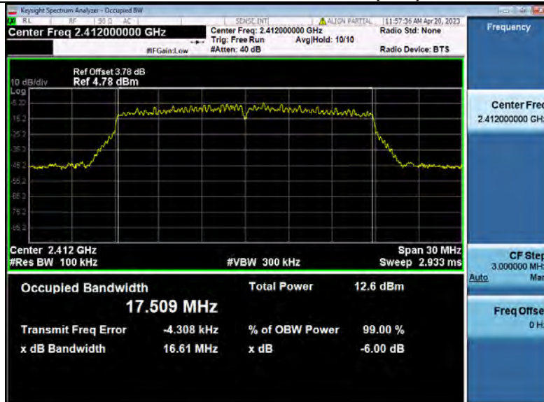
-6dB_Bandwidth_NVNT_ANT4_802_11n(HT20)_2412
