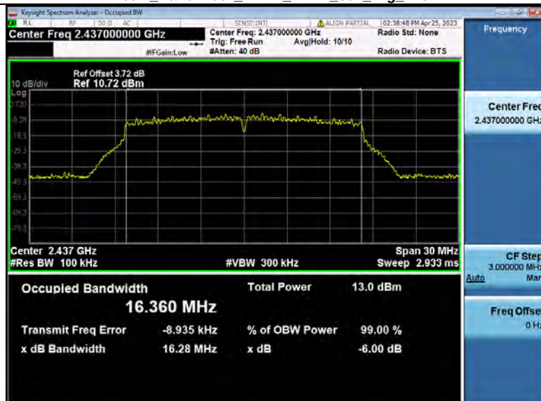
-6dB_Bandwidth_NVNT_ANT1_802_11g_2437
