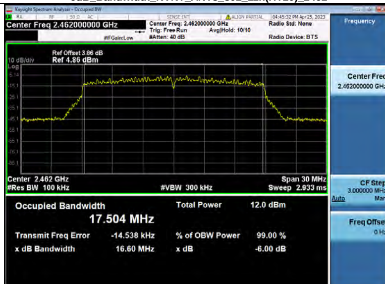
-6dB_Bandwidth_NVNT_ANT3_802_11n(HT20)_2462
