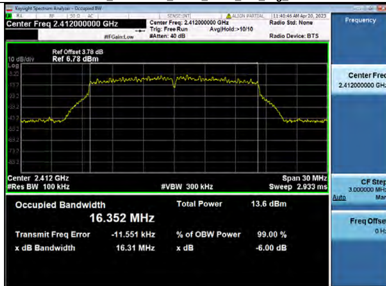
-6dB_Bandwidth_NVNT_ANT4_802_11g_2412
