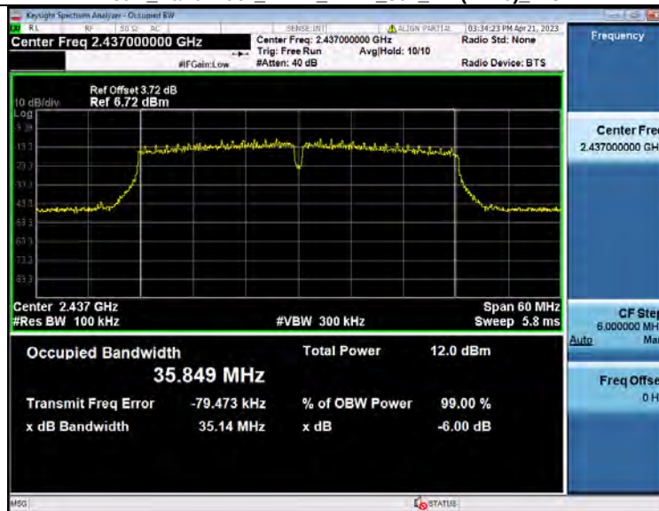
-6dB_Bandwidth_NVNT_ANT2_802_11n(HT40)_2437
