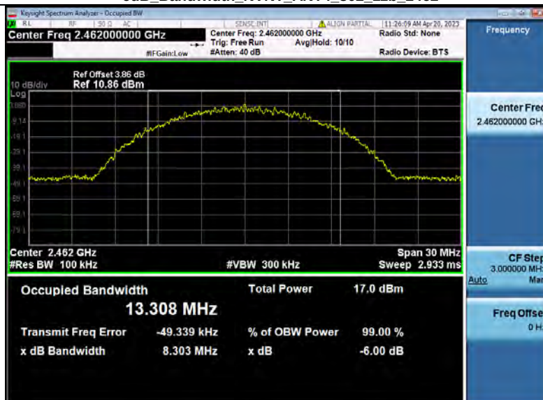
-6dB_Bandwidth_NVNT_ANT4_802_11b_2462
