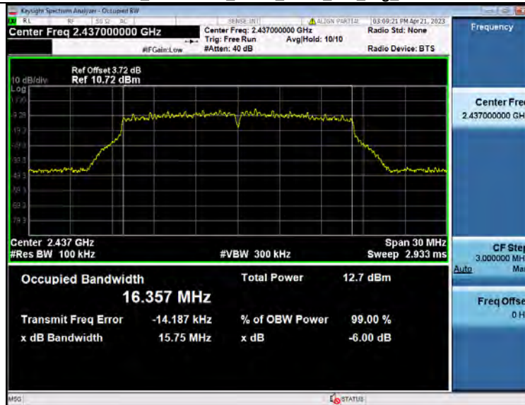
-6dB Bandwidth_NVNT_ANT2_802_11g_2437
