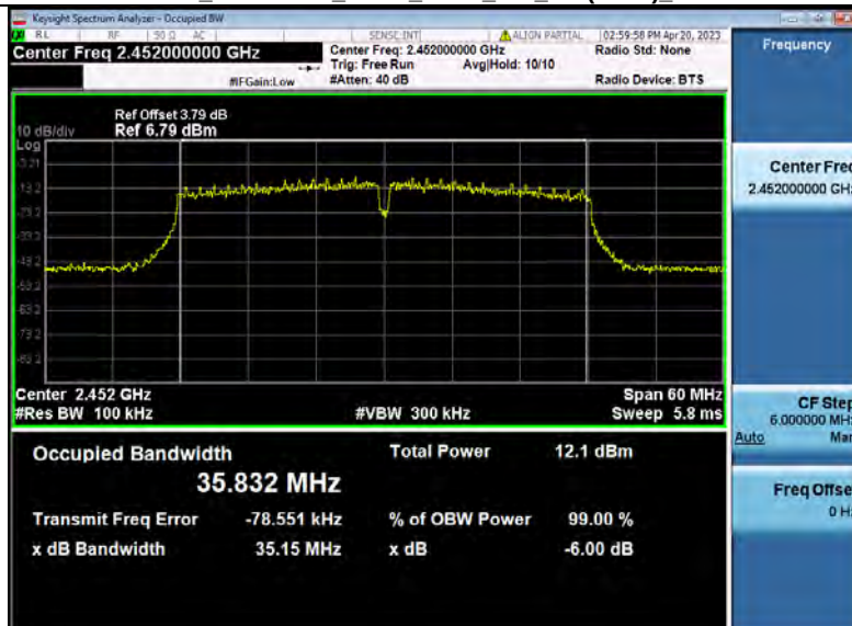
-6dB_Bandwidth_NVNT_ANT4_802_11n(HT40)_2452
