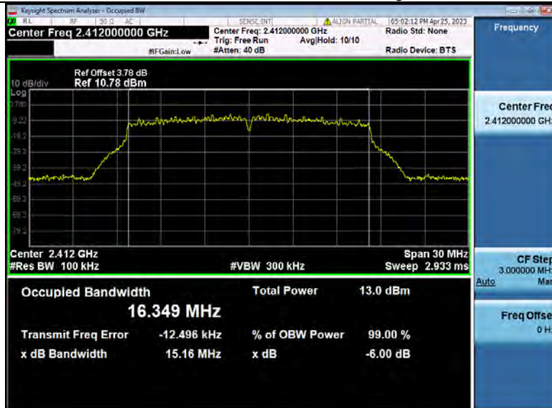
-6dB_Bandwidth_NVNT_ANT3_802_11g_2412
