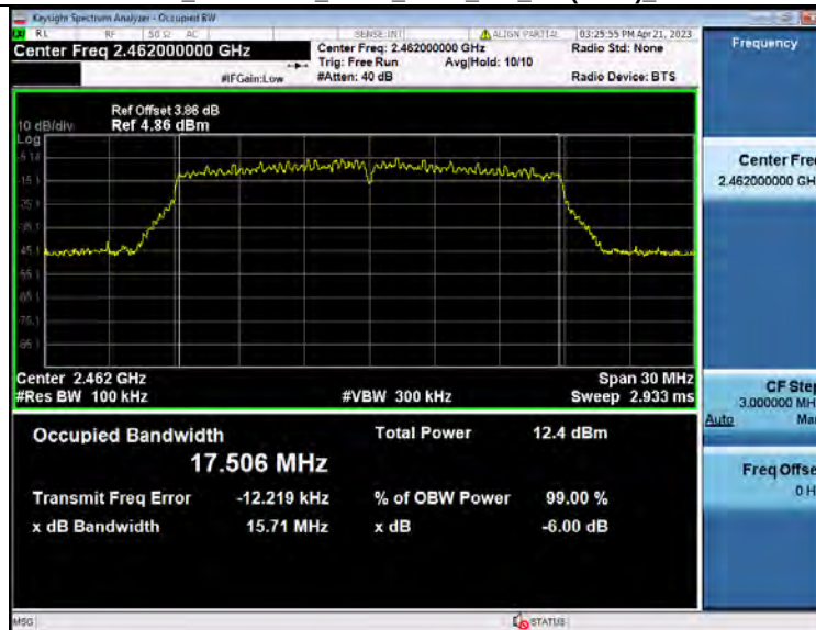
-6dB_Bandwidth_NVNT_ANT2_802_11n(HT20)_2462
