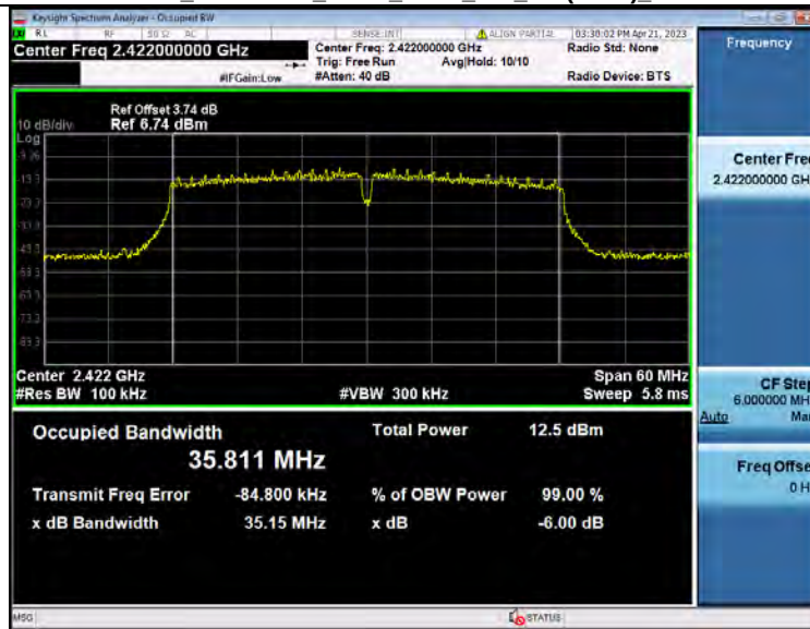
-6dB_Bandwidth_NVNT_ANT2_802_11n(HT40)_2422
