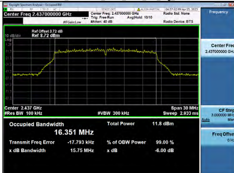
-6dB_Bandwidth_NVNT_ANT3_802_11g_2437
