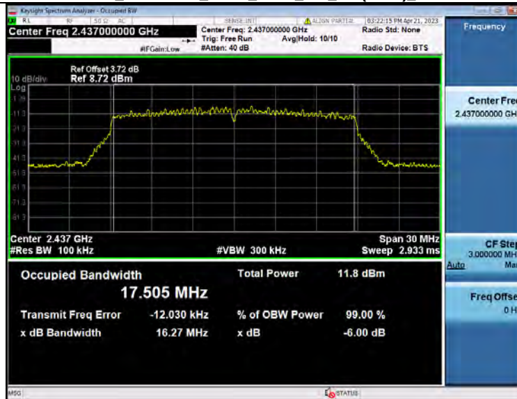
-6dB_Bandwidth_NVNT_ANT2_802_11n(HT20)_2437
