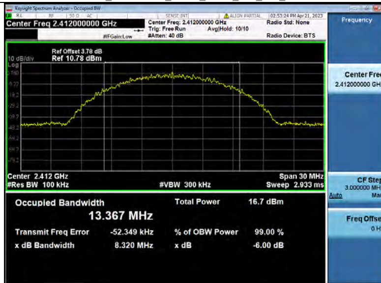
-6dB Bandwidth_NVNT_ANT2_802_11b_2412
