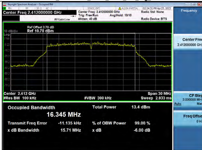
-6dB_Bandwidth_NVNT_ANT1_802_11g_2412
