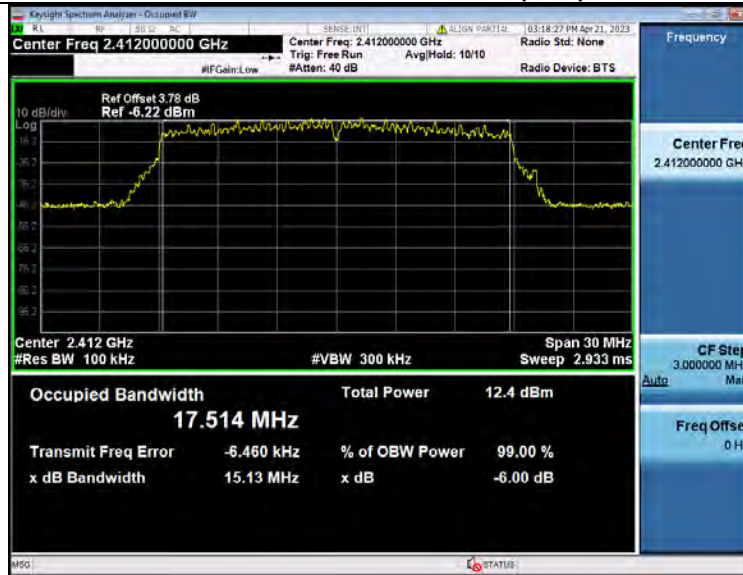
-6dB_Bandwidth_NVNT_ANT2_802_11n(HT20)_2412
