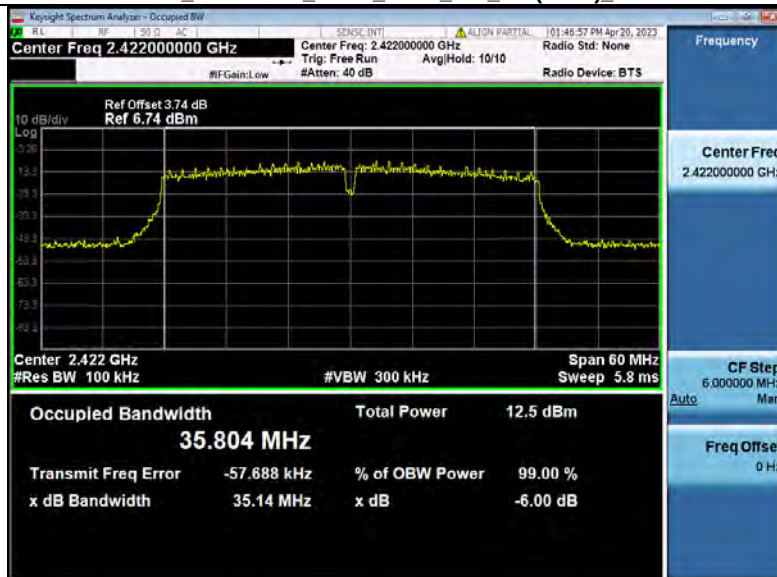
-6dB_Bandwidth_NVNT_ANT4_802_11n(HT40)_2422
