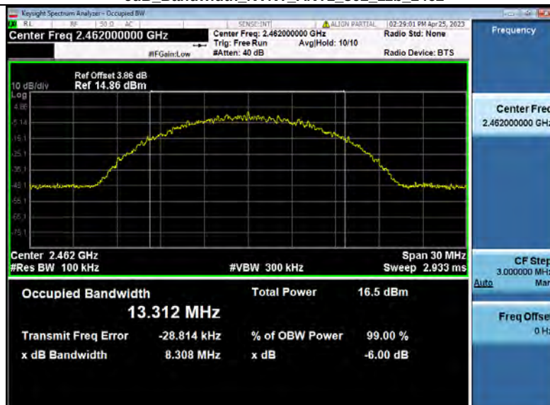
-6dB_Bandwidth_NVNT_ANT1_802_11b_2462
