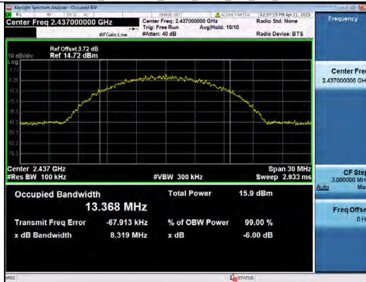
-6dB Bandwidth_NVNT_ANT2_802_11b_2437
