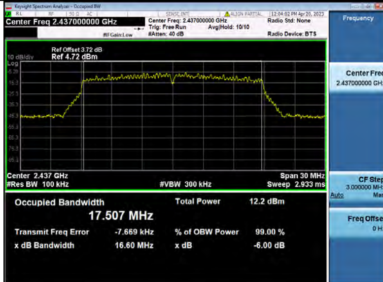
-6dB_Bandwidth_NVNT_ANT4_802_11n(HT20)_2437
