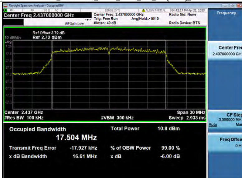
-6dB_Bandwidth_NVNT_ANT3_802_11n(HT20)_2437
