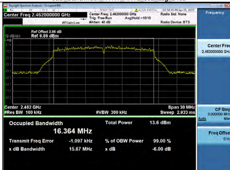
-6dB_Bandwidth_NVNT_ANT1_802_11g_2462
