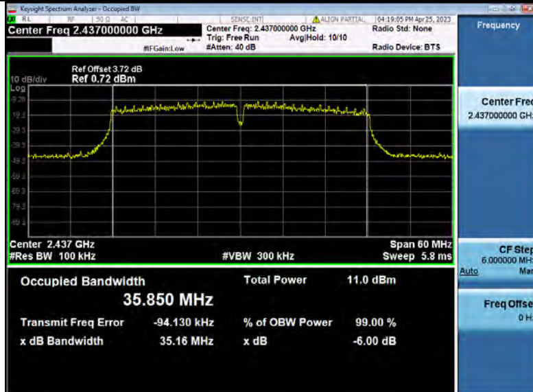
-6dB_Bandwidth_NVNT_ANT3_802_11n(HT40)_2437
