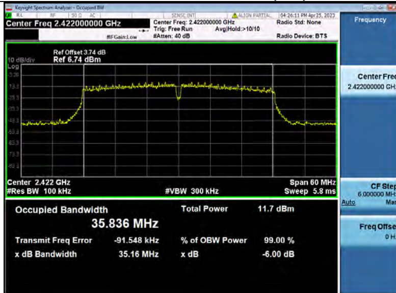
-6dB_Bandwidth_NVNT_ANT3_802_11n(HT40)_2422
