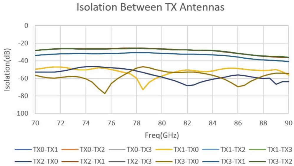
Figure 3 Isolation between TX Antennas
