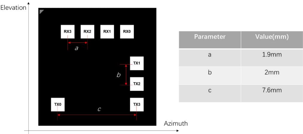
Figure 1 Configuration of CAL77S244-AB
