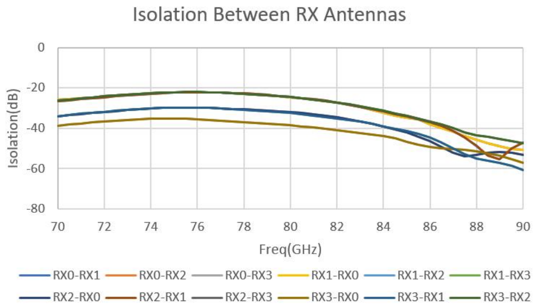
Figure 6 Isolation between RX Antennas
