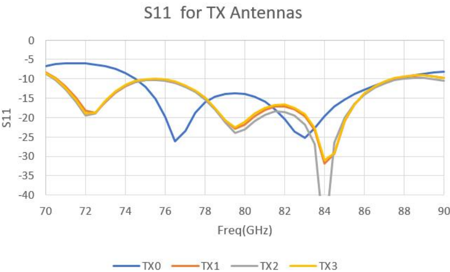
Figure 2 S11 for TX Antennas
