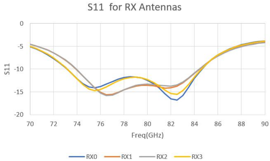
Figure 5 S11 for RX Antennas
