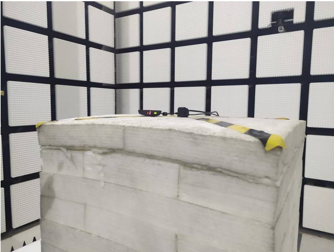
Radiated Emission Above 1GHz View 220G-231G
