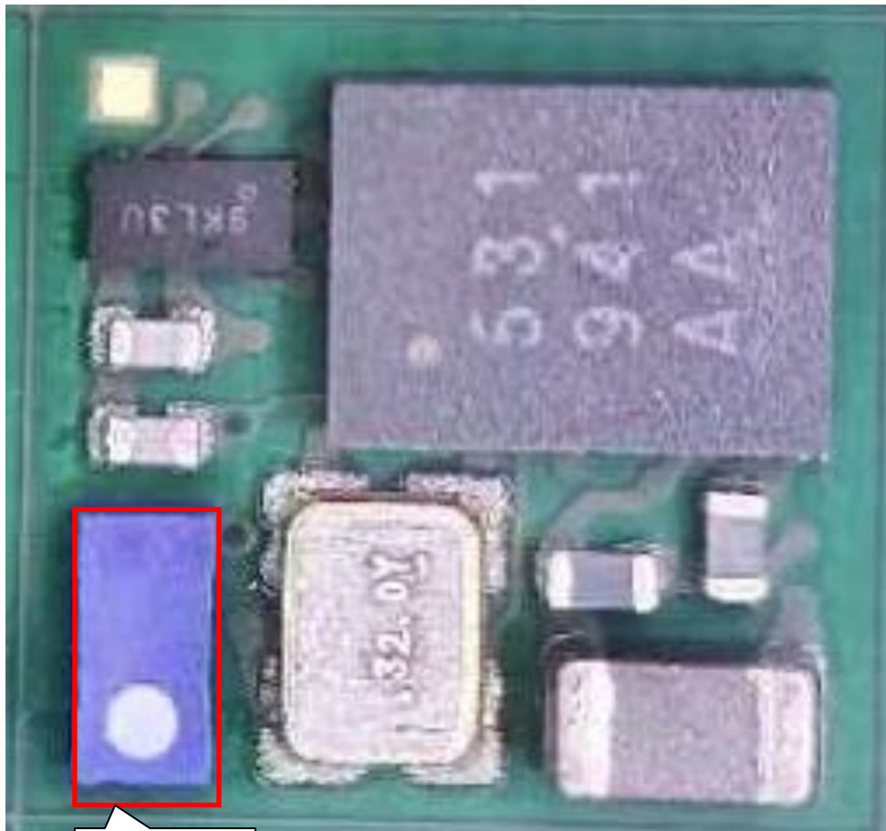
BT Antenna
