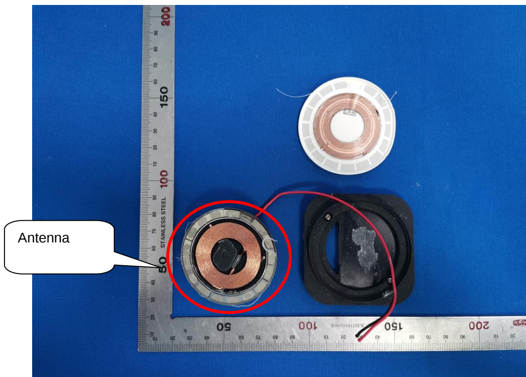
WPT ANTENNA
