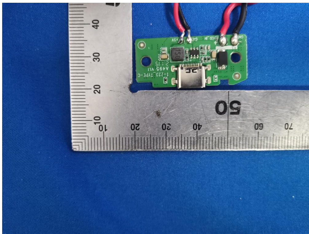
WPT-2 OPEN VIEW OF EUT (FIGURE 1)
