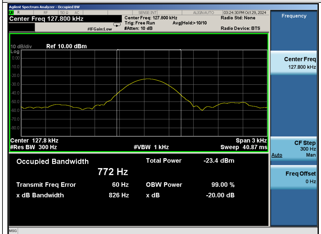
Test_Graph_ASK_127.8kHz _ 99% Occupied Bandwidth
