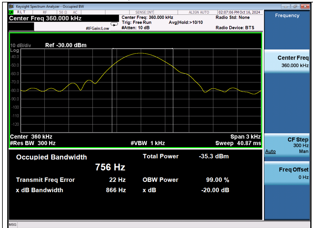
Test_Graph_ASK_360kHz _ 99% Occupied Bandwidth
