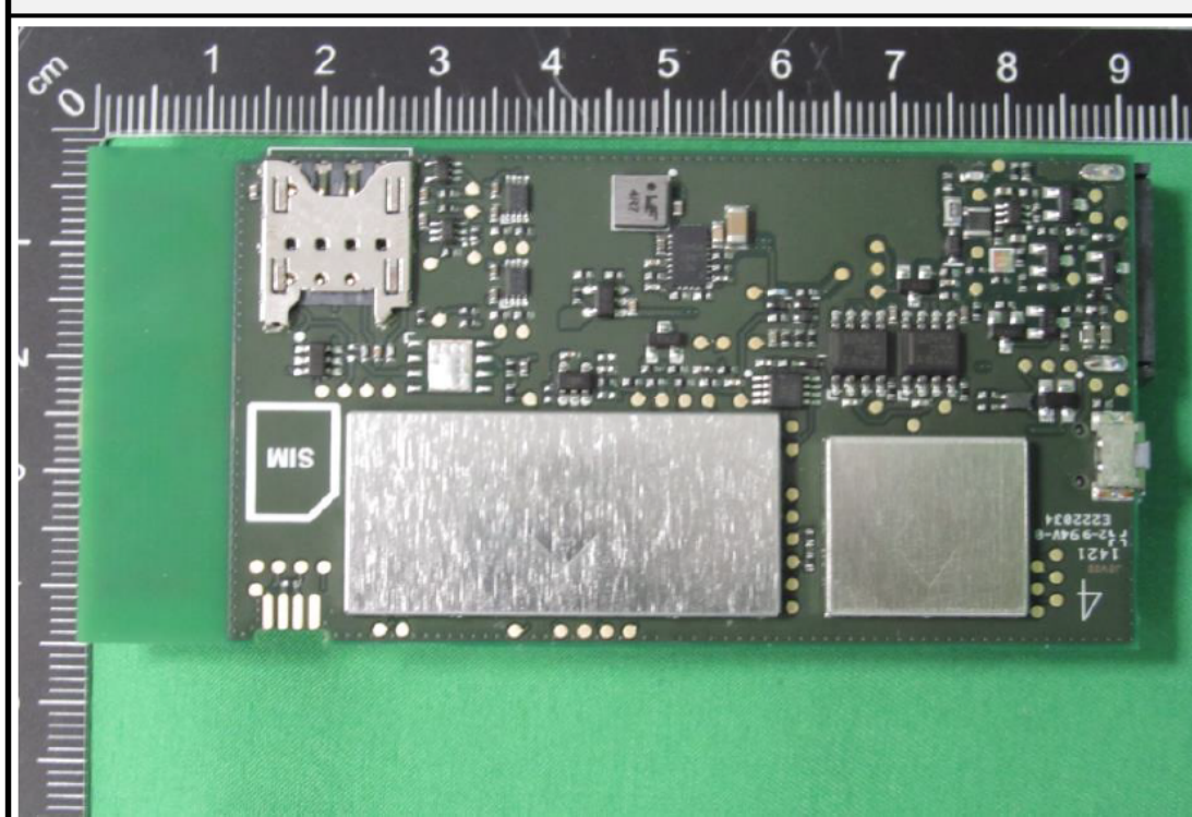
PCB back view
