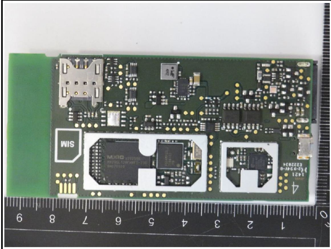
PCB back view without shielding
