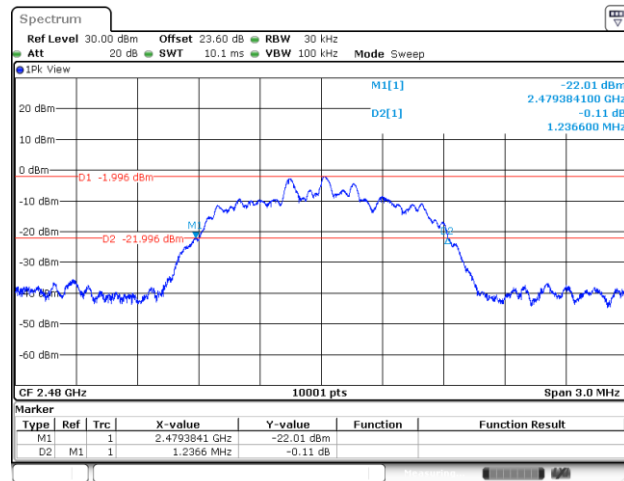
20 dB Bandwidth Plot in Channel 78
