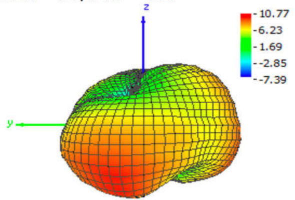
Theta = 90, Phi = 180
