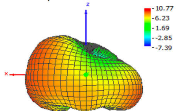
Theta = 90, Phi = 90
