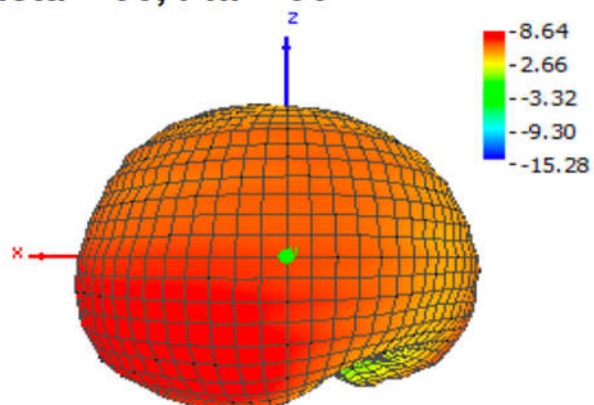
Theta = 90, Phi = 90
