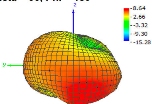
Theta = 90, Phi = 180
