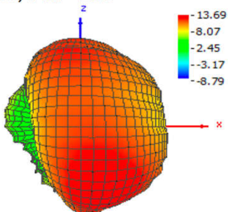
Theta = 90, Phi = 270
