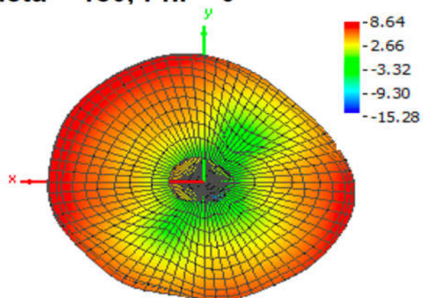
Theta = 180, Phi = 0
