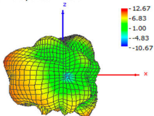
Theta = 90, Phi = 270
