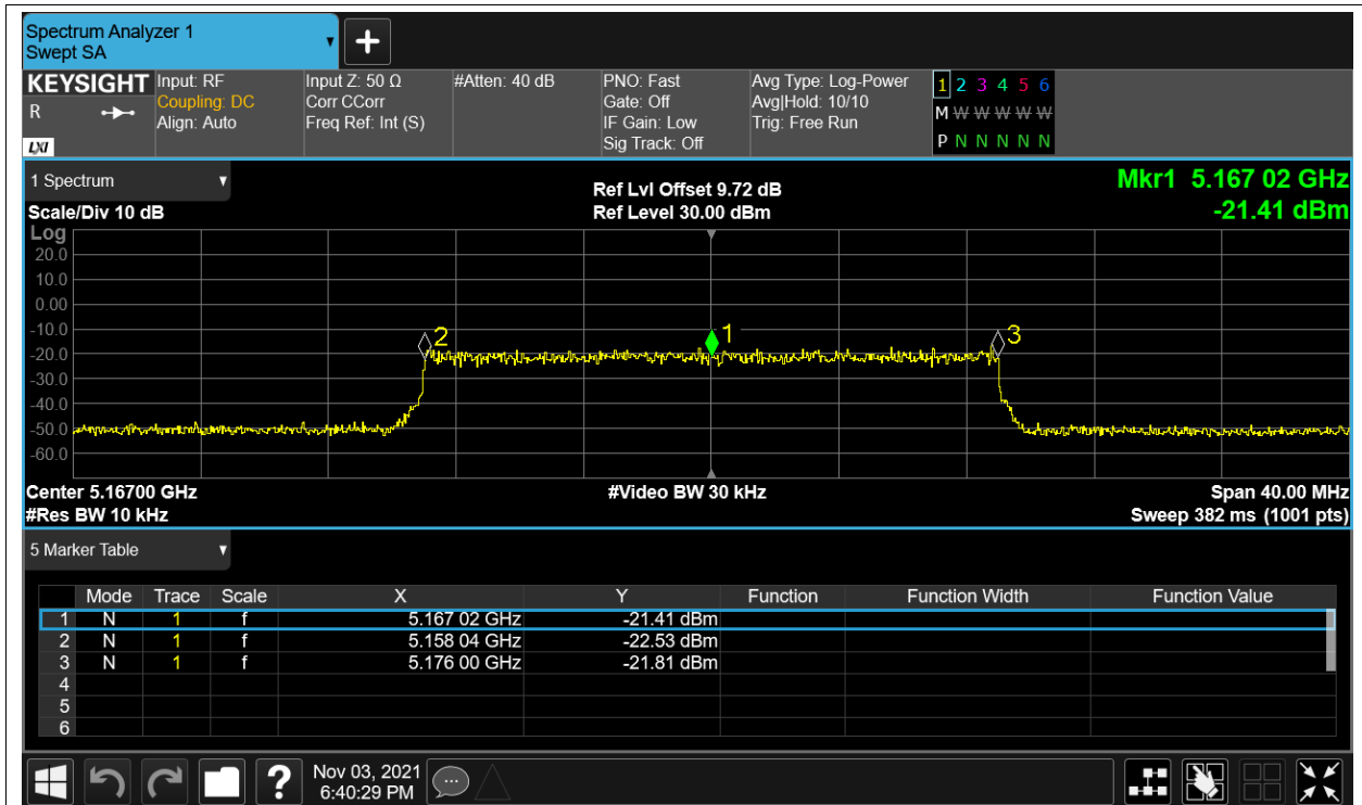
Freq. Stability LVL 5.2G-20M-16QAM 5167MHz Sum
